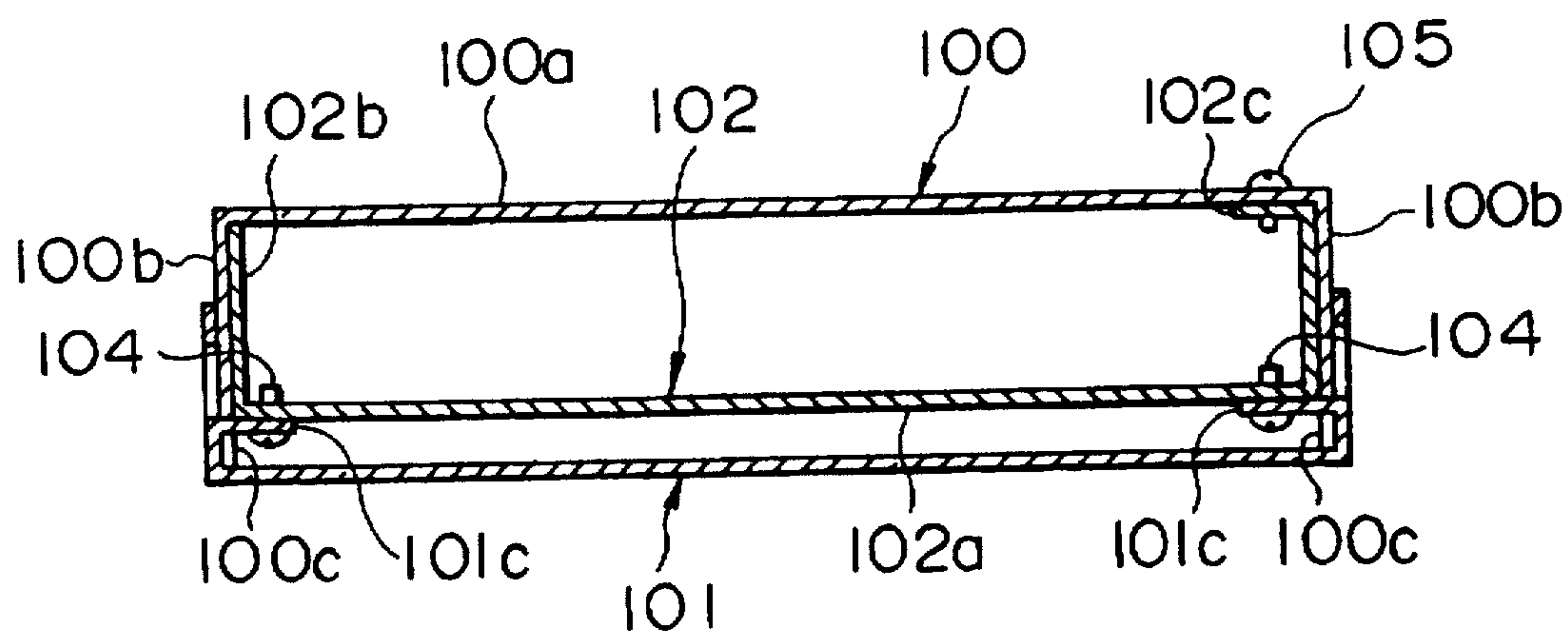
FIG. 51 PRIOR ART
