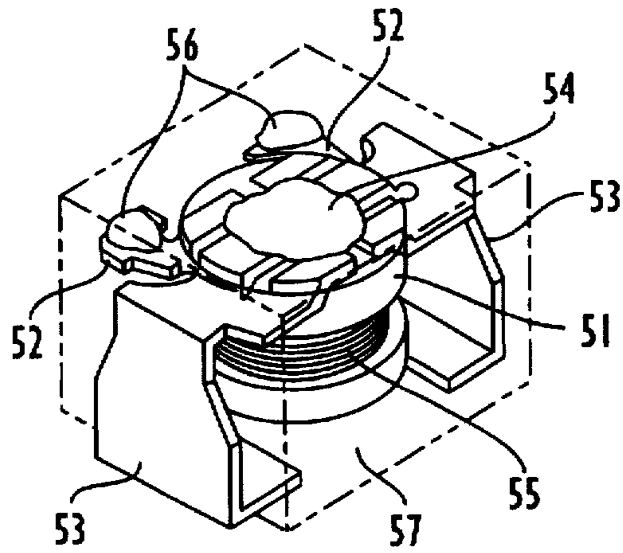
FIG. 13 PRIOR ART
