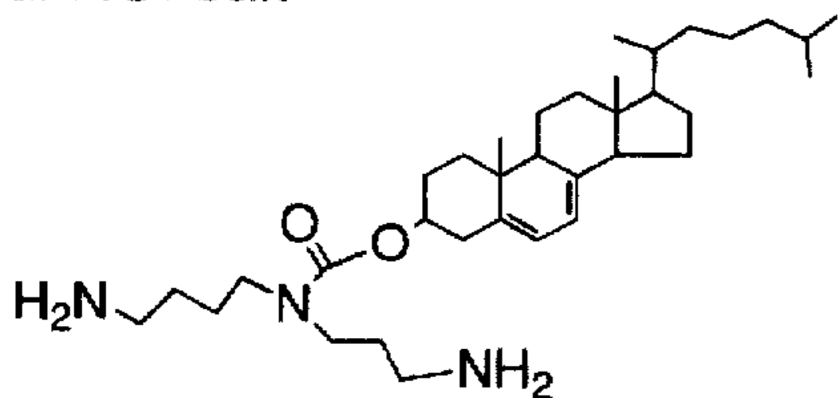
65 N 4 -spermidine-7 dehydro cholesteryl carbamate
