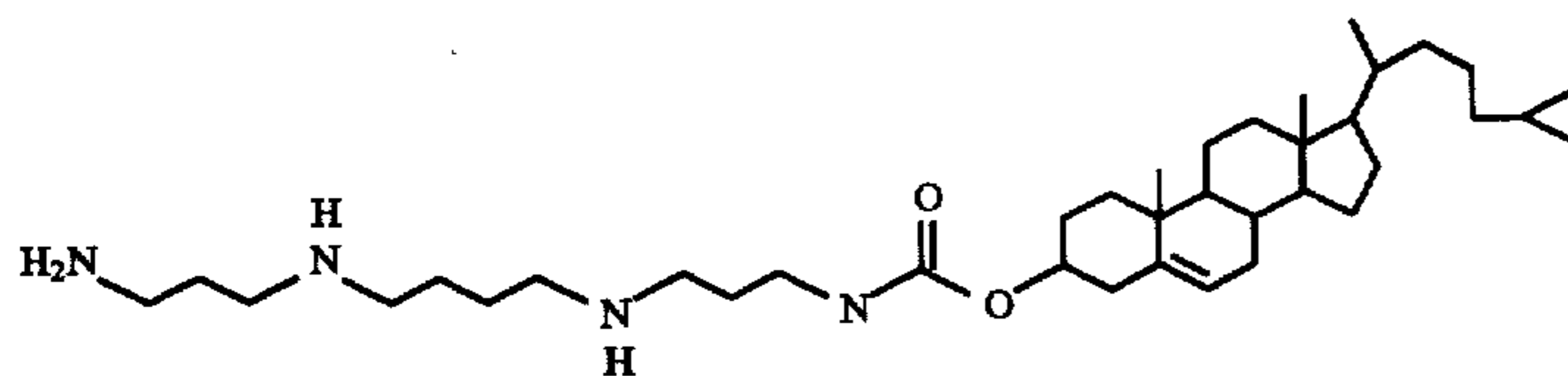
(N 1 -Spermine cholesteryl carbamate).
