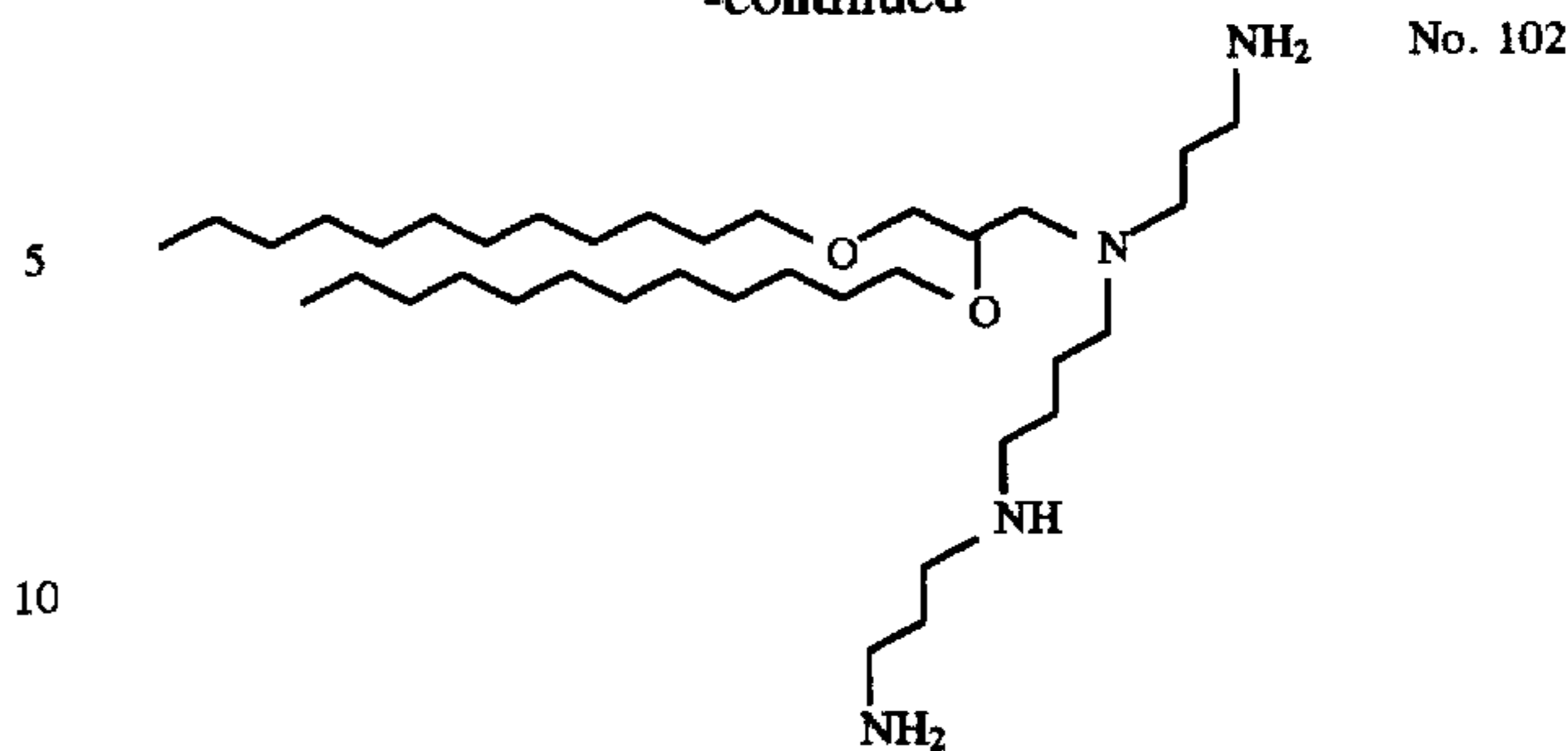
N 4 -spermine-2,3-dilauryl-oxypropylamine
