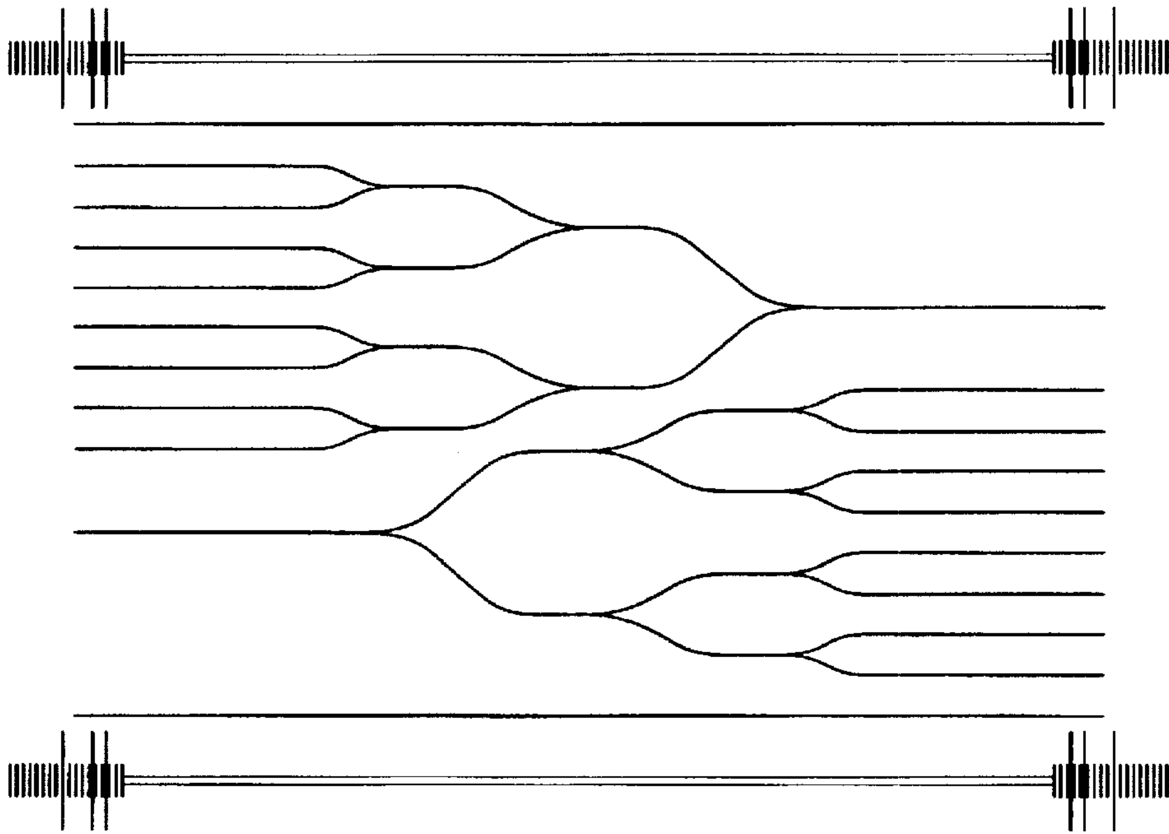
( 1 X 8 SPLITTER )
