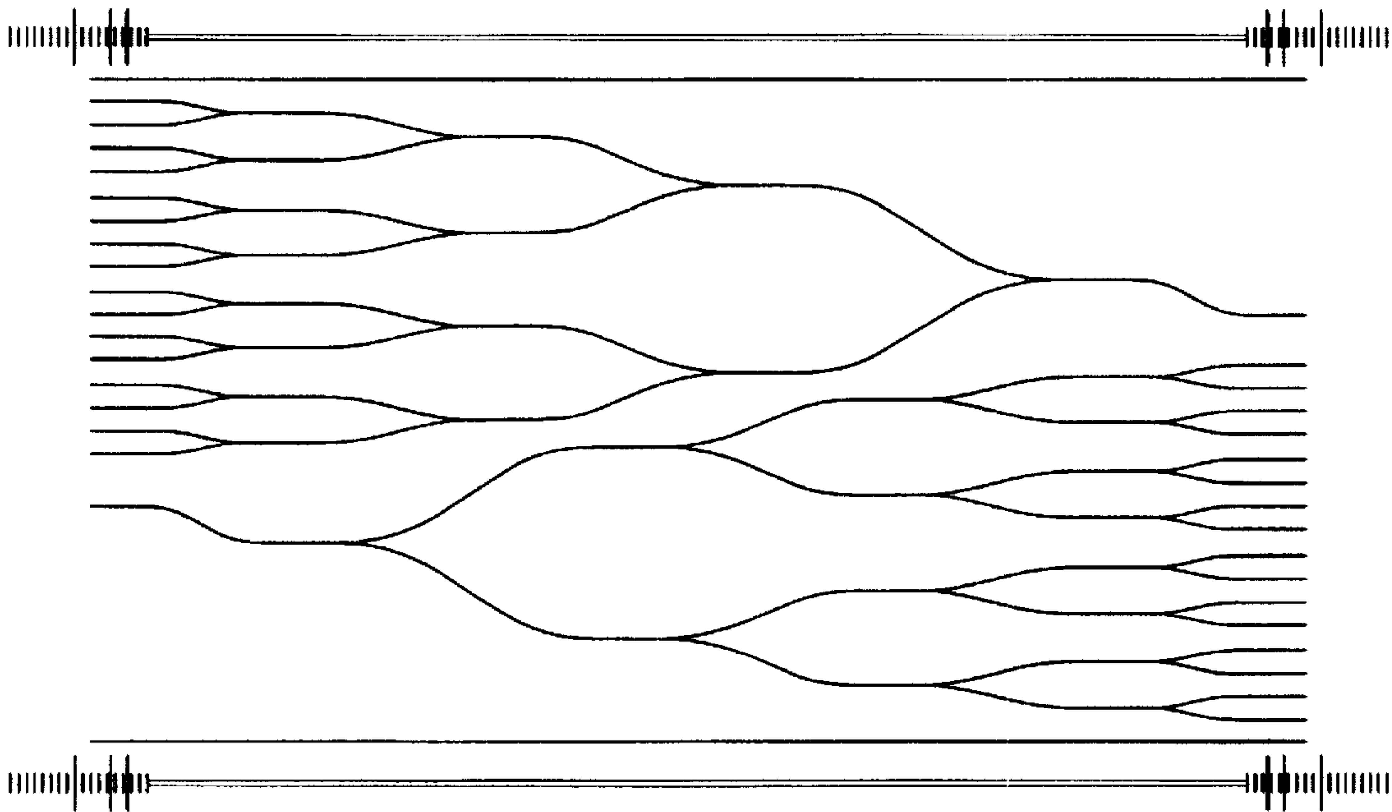
( 1 X 16 SPLITTER )
