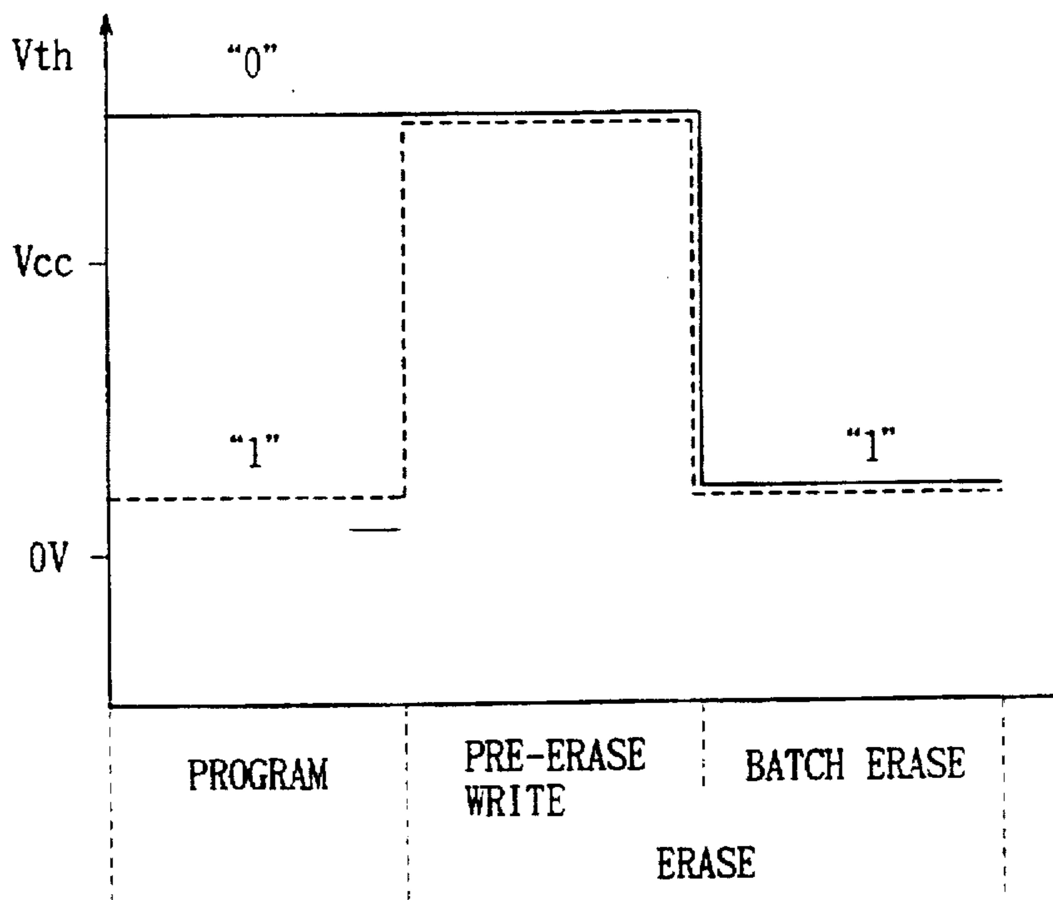
FIG. 140 PRIOR ART
