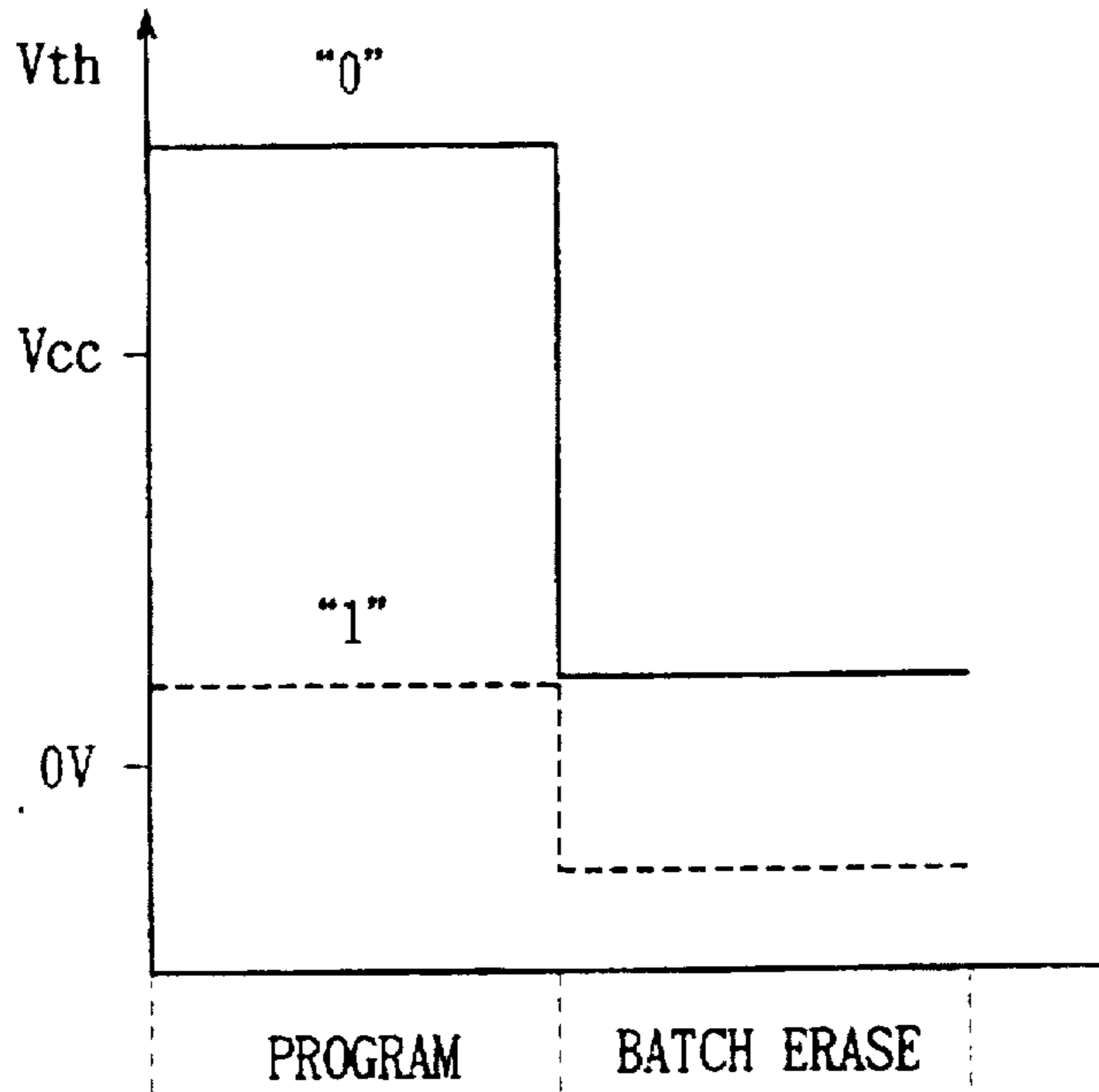
FIG. 139 PRIOR ART
