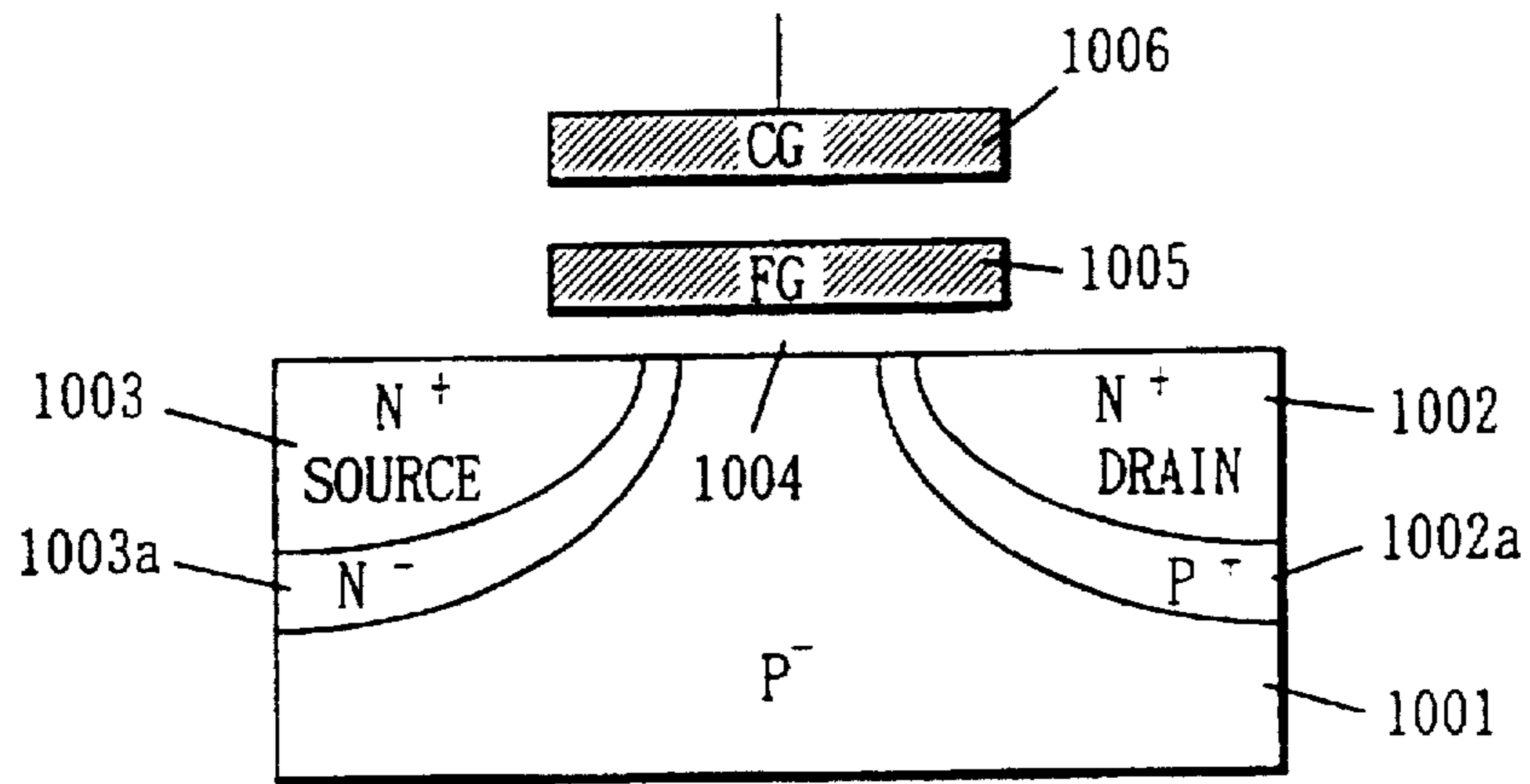
FIG. 128 PRIOR ART
