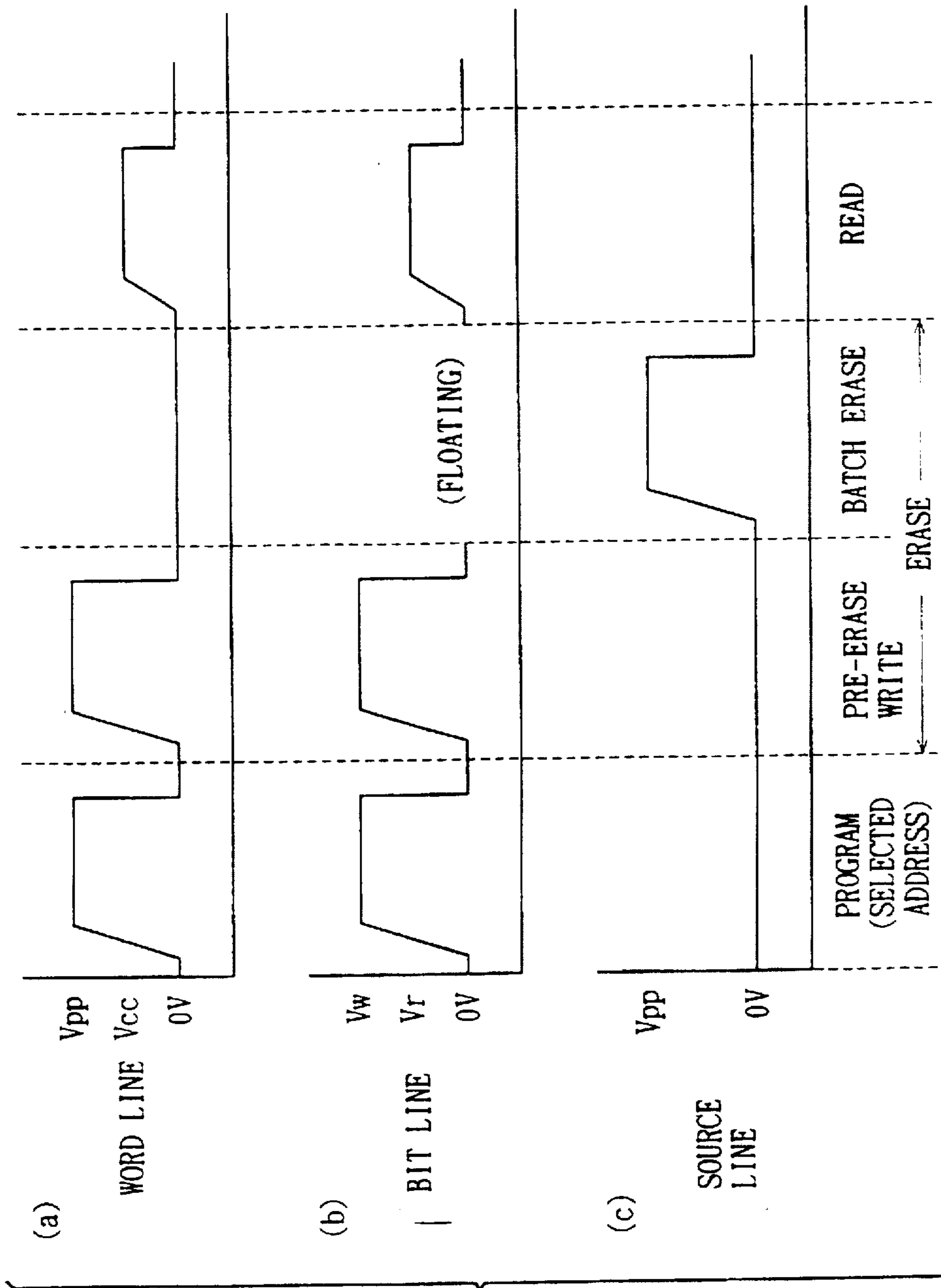
FIG. 138 PRIOR ART
