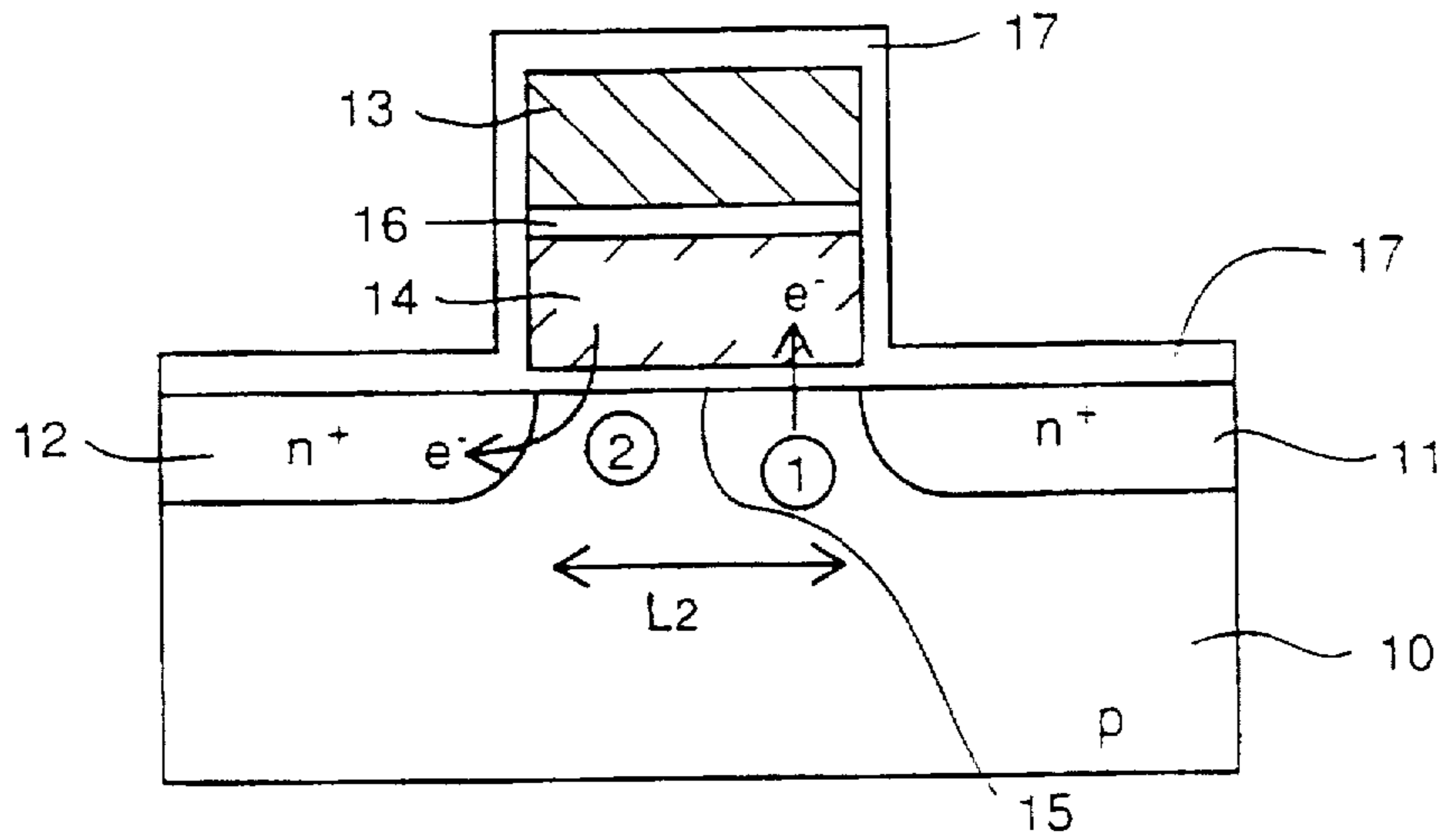
FIG. 151 PRIOR ART
