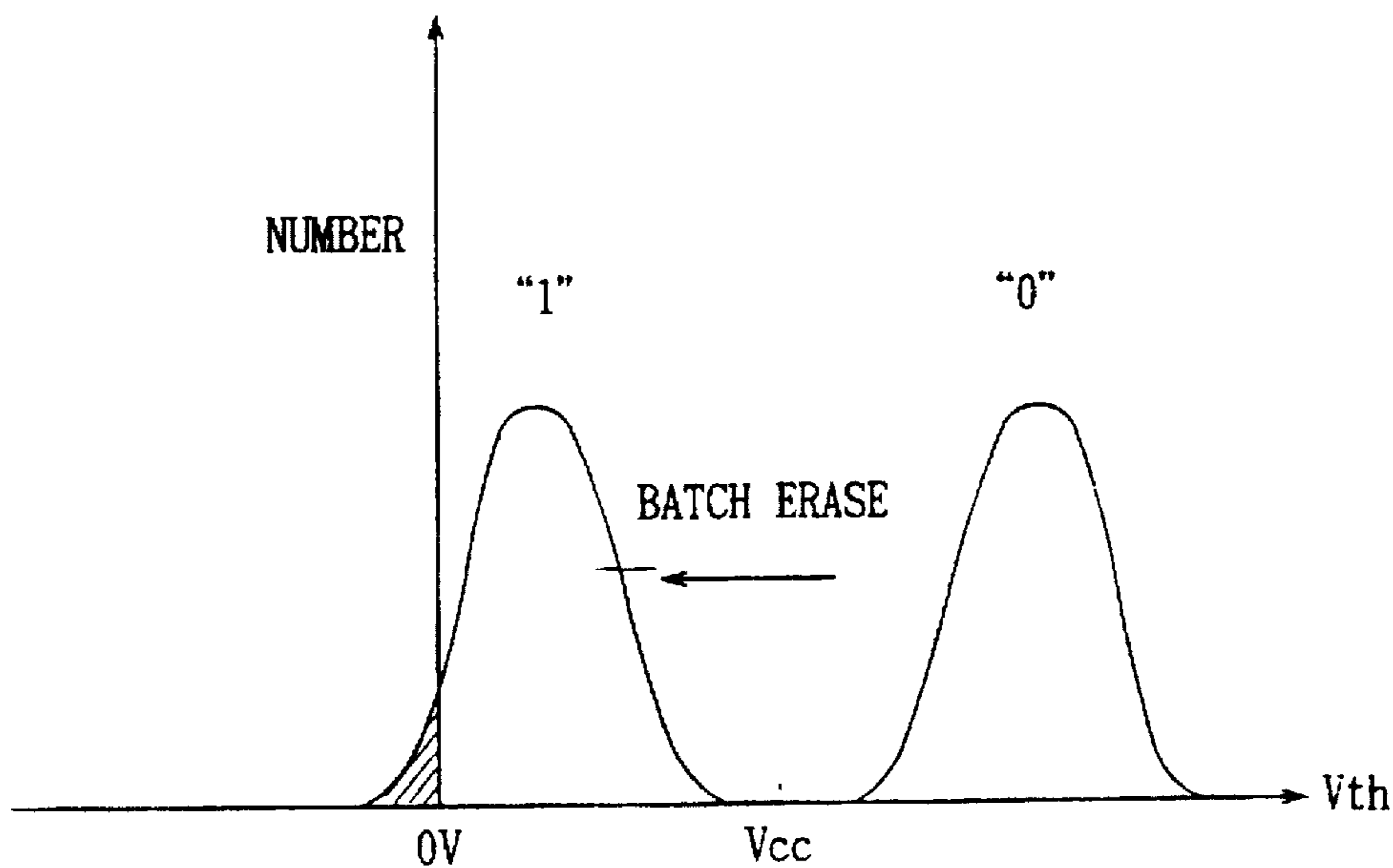
FIG. 142 PRIOR ART
