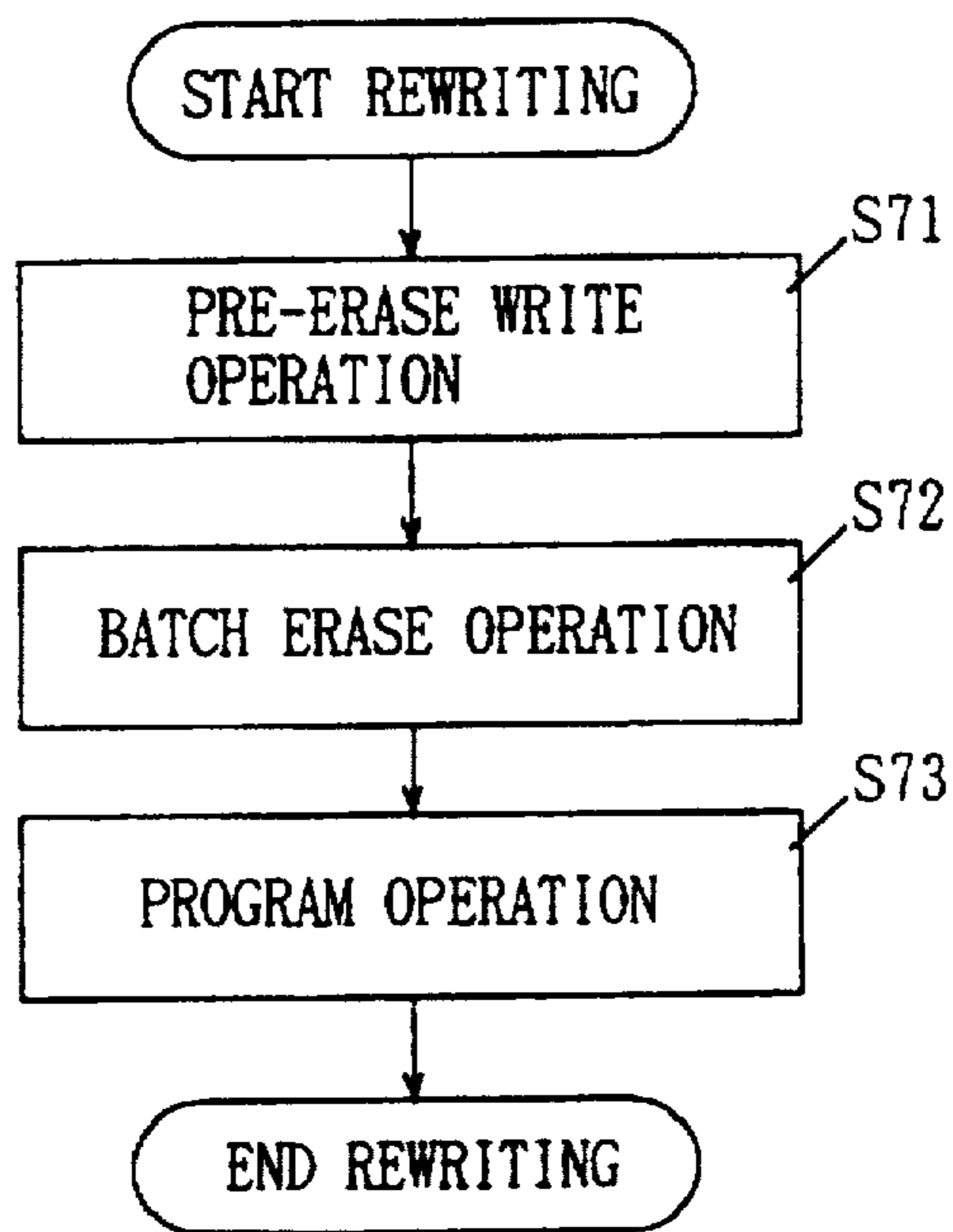
FIG. 141 PRIOR ART
