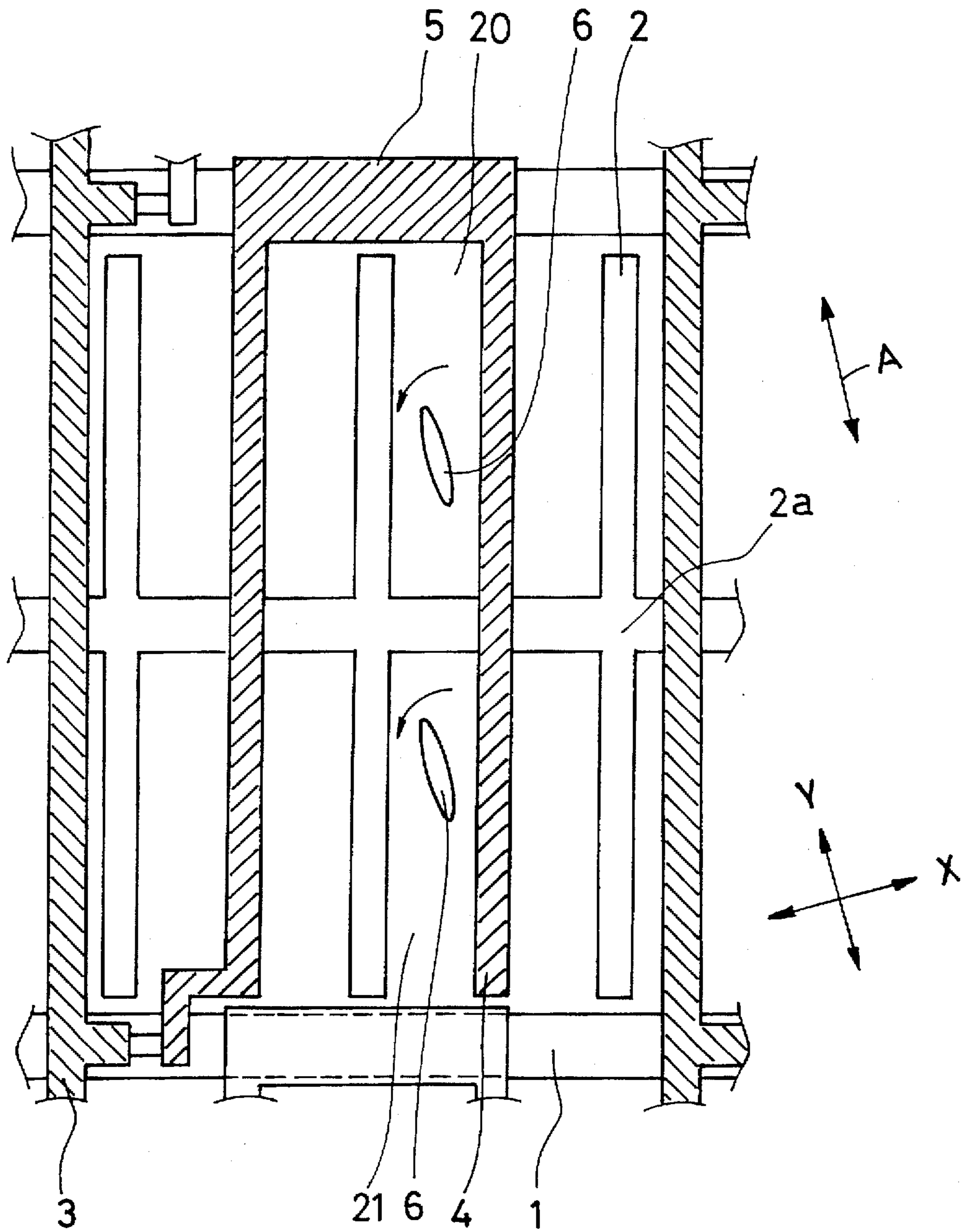
FIG. 6 (PRIOR ART)
