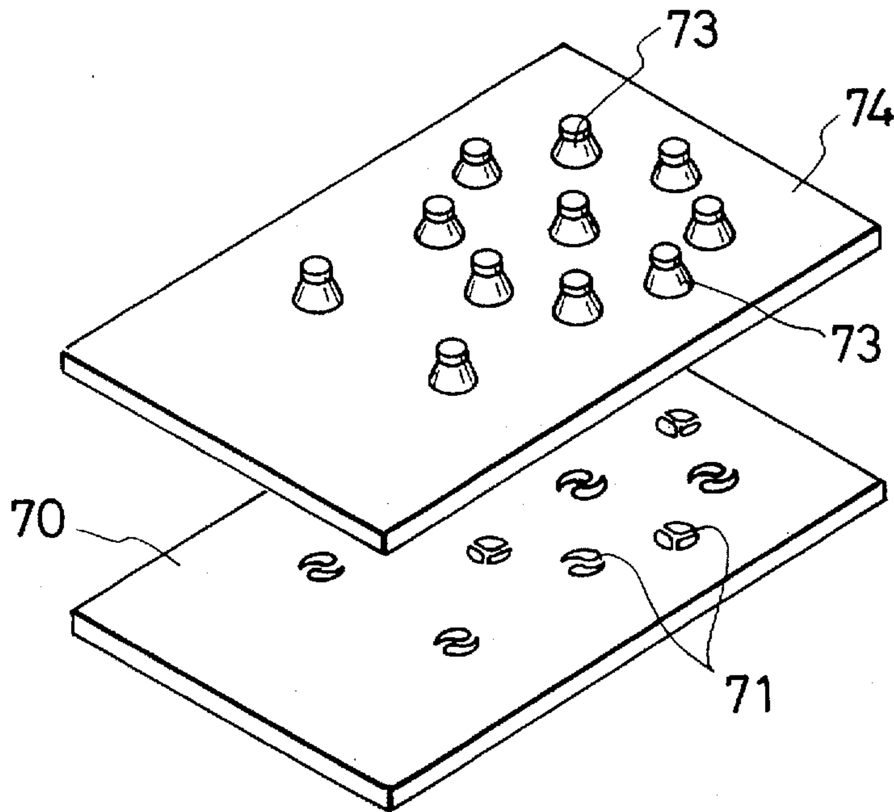
FIG. 2 PRIOR ART
