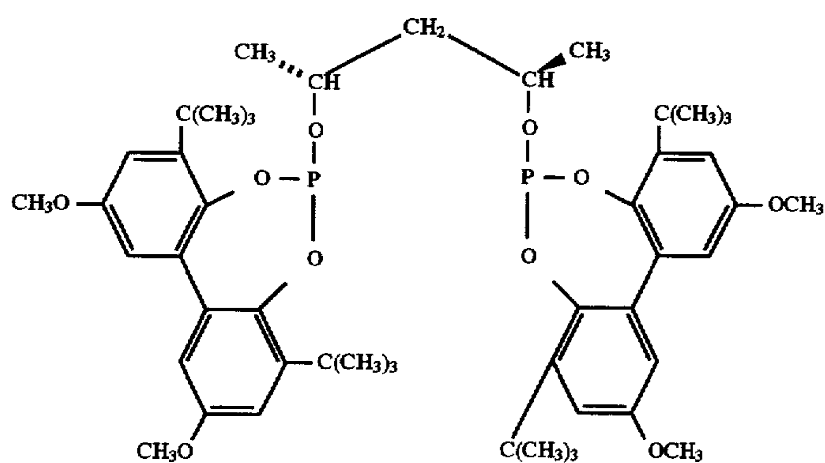
Ligand M
