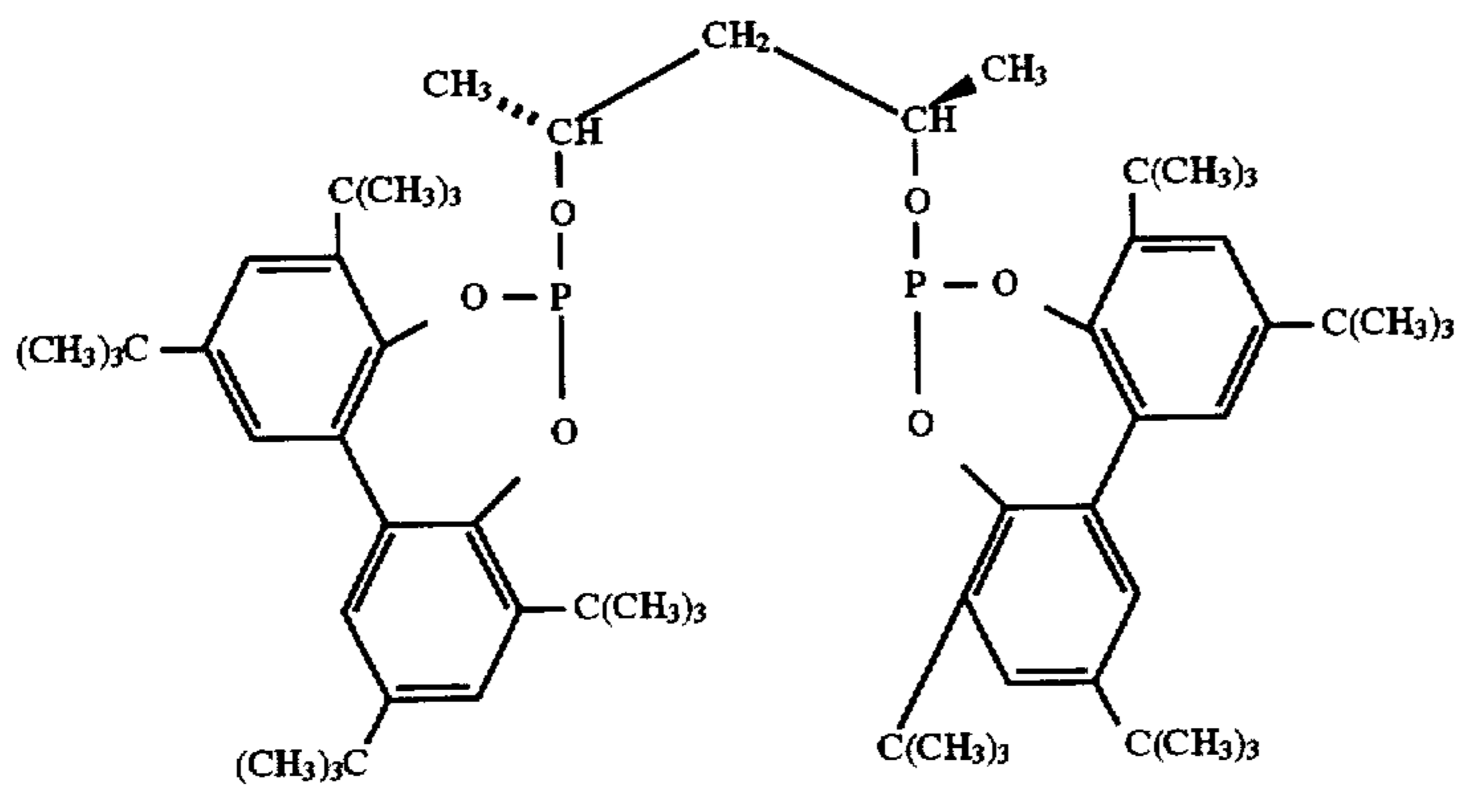
Ligand H
