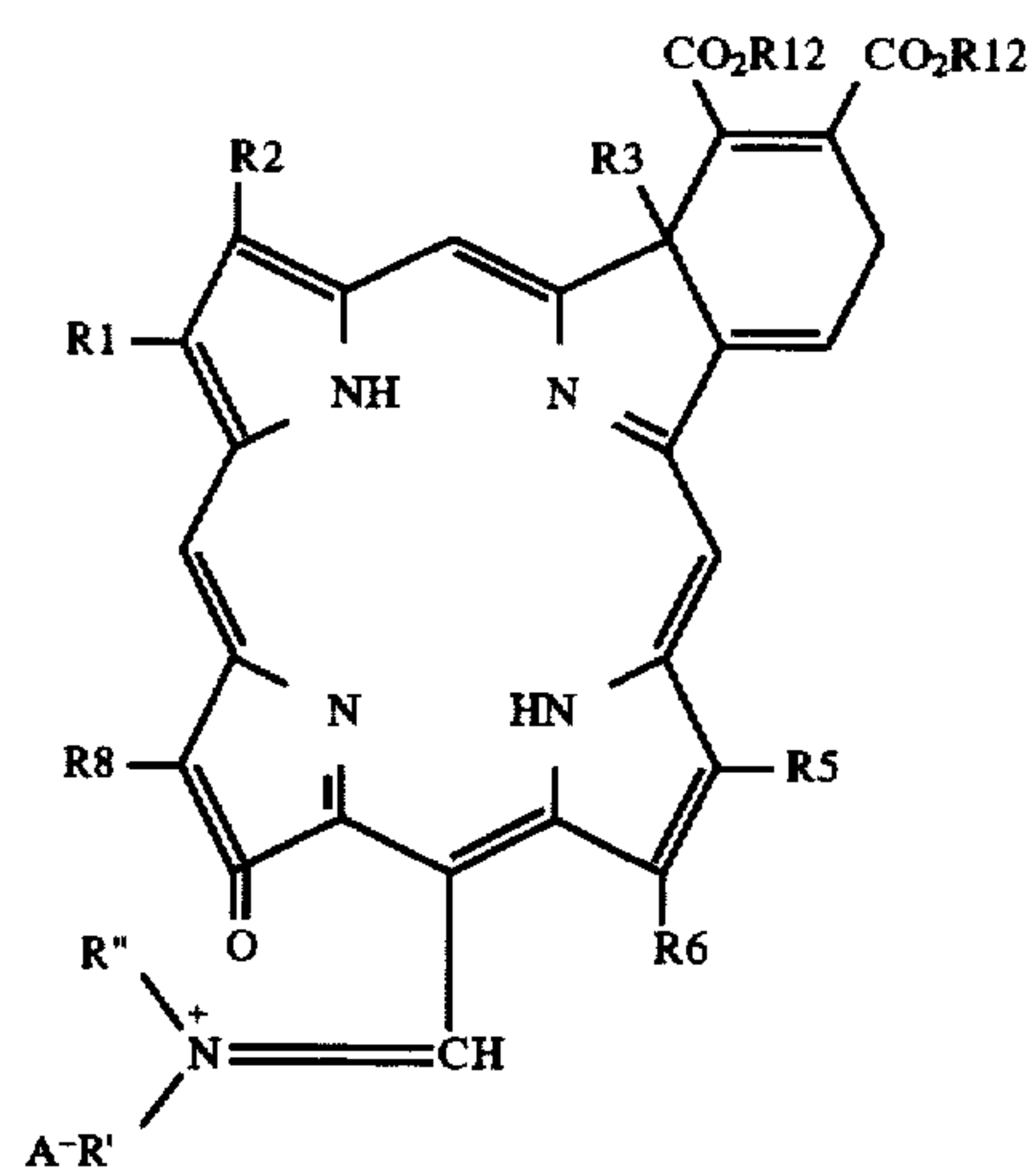
Bacteriochlorin Diels Alder Adduct Imine II
