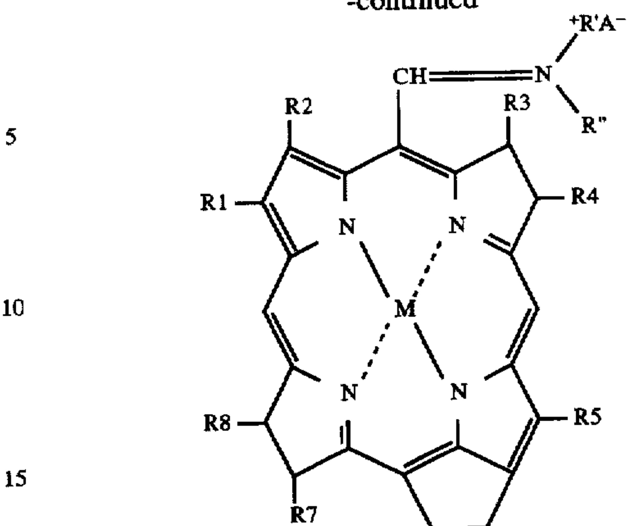
Bacteriochlorophyllimine II Metal Complex
