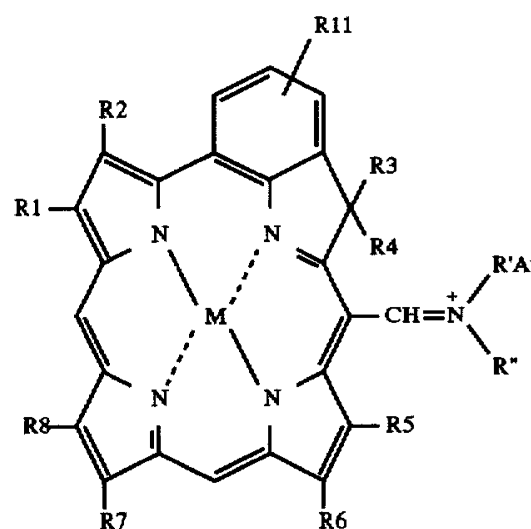
Benzochlorinimine Metal complex
