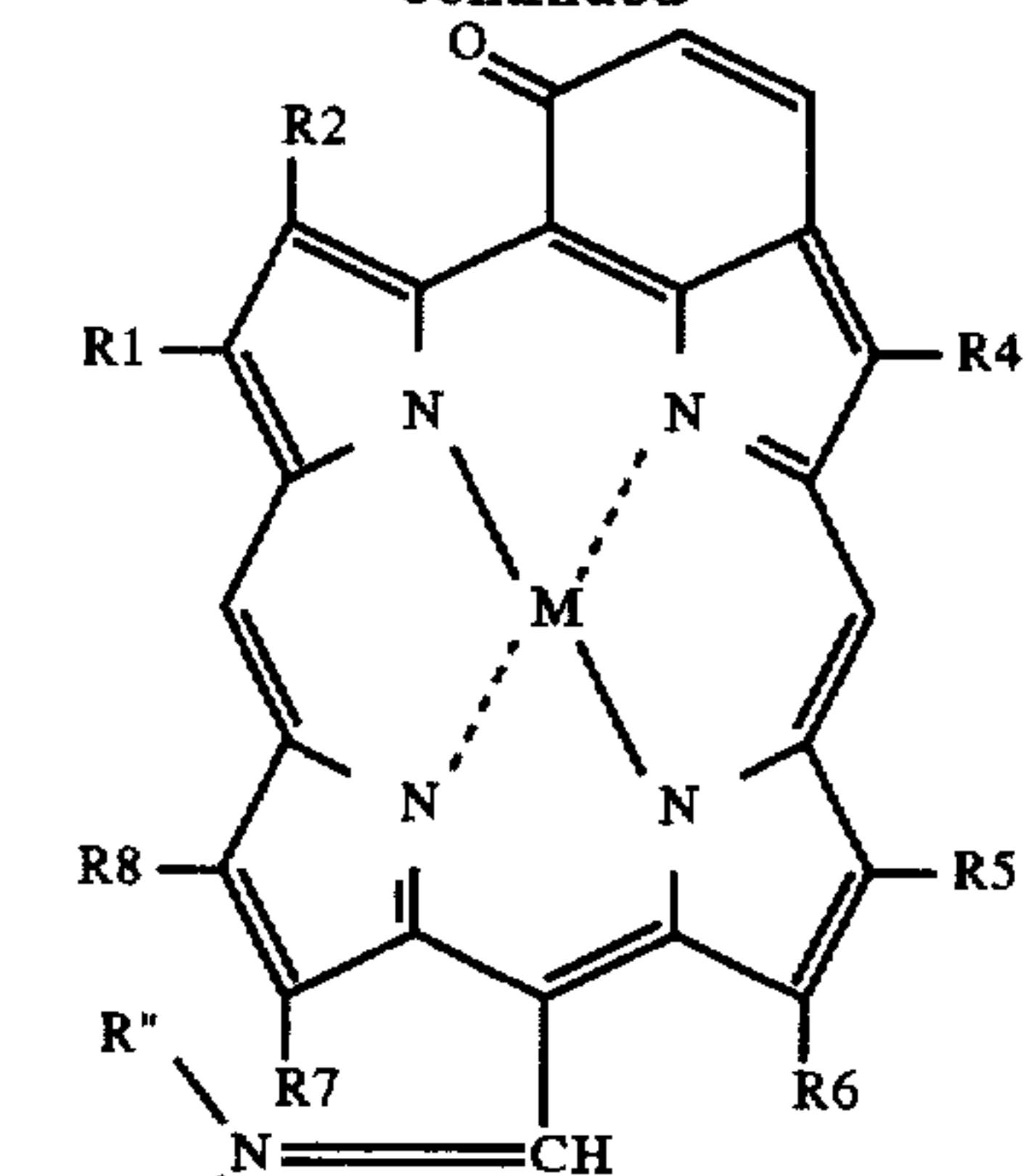
Verdininimine II Metal Complex
