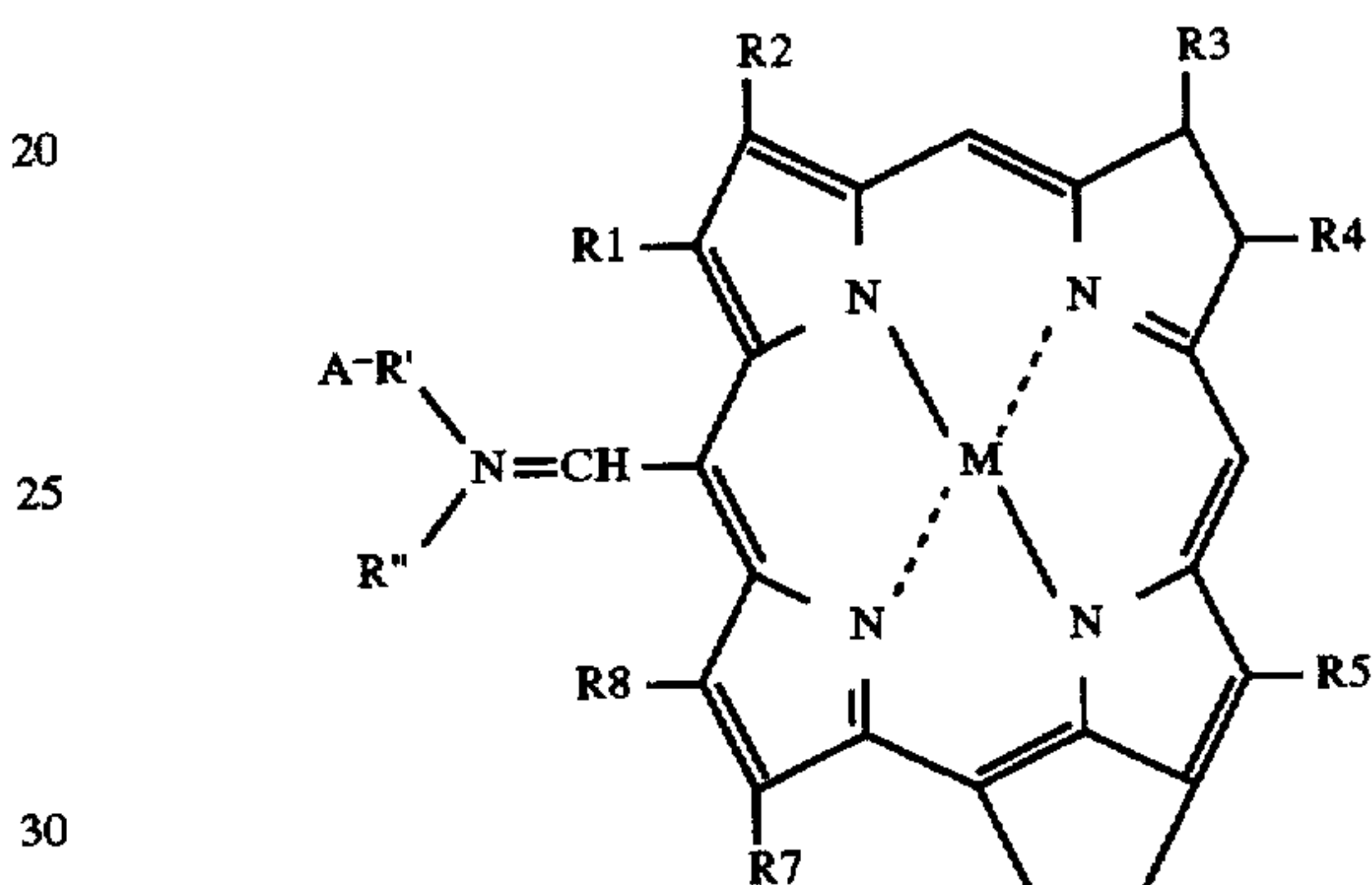
Bacteriochlorophyllimine III Metal Complex
