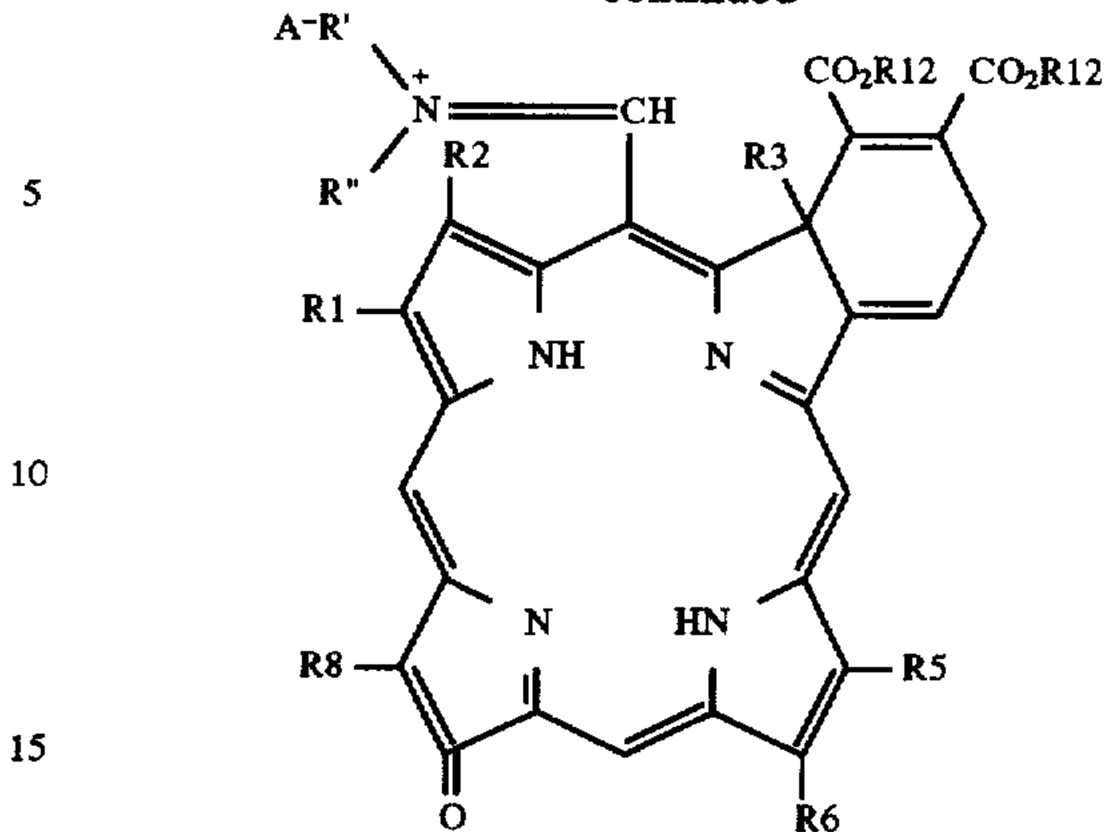
Bacteriochlorin Diels Alder Adduct Imine IV
