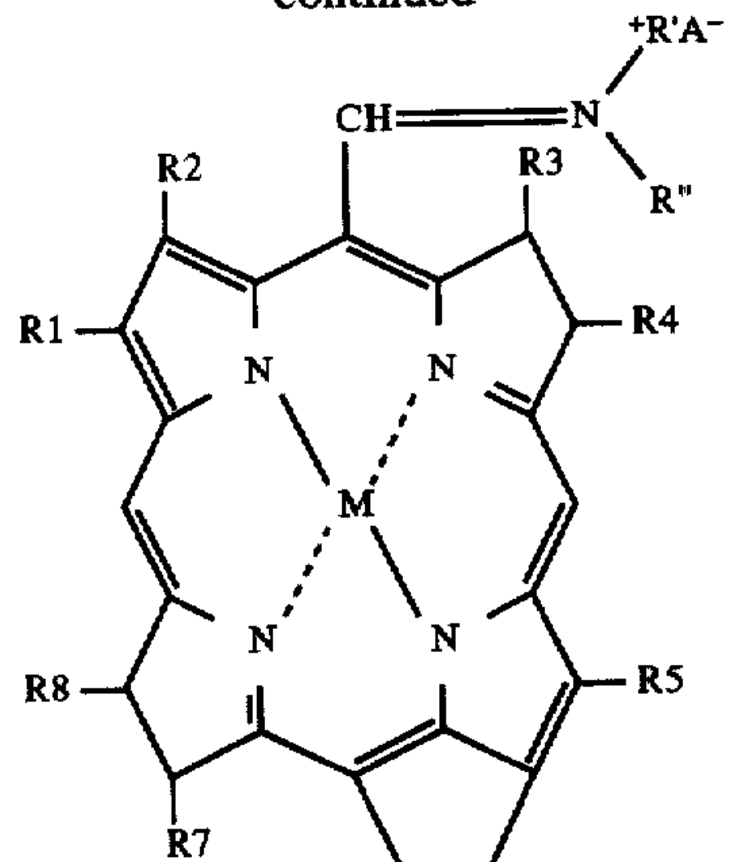
Bacteriochlorophyllimine II Metal Complex
