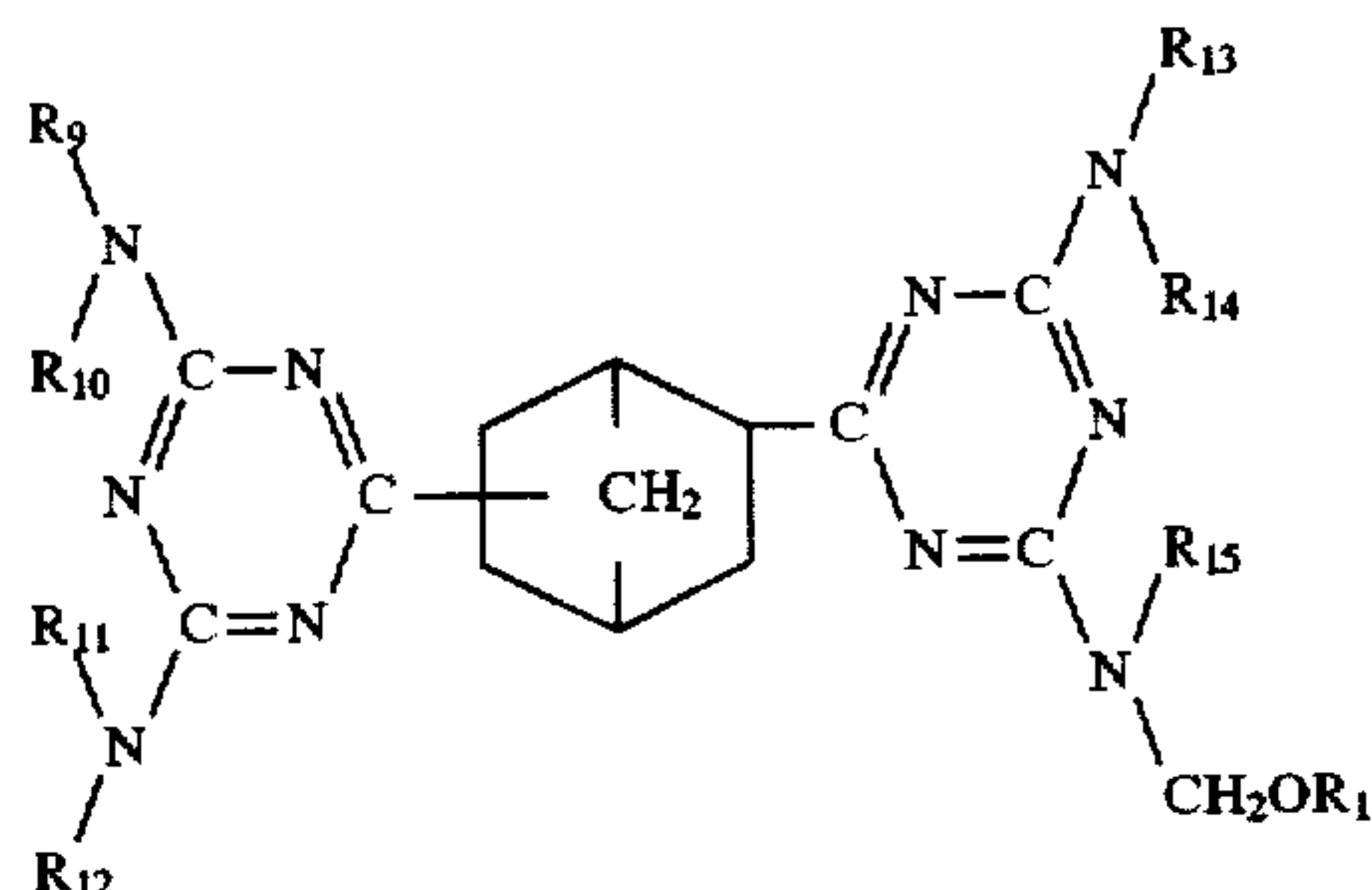
Formula (7)
