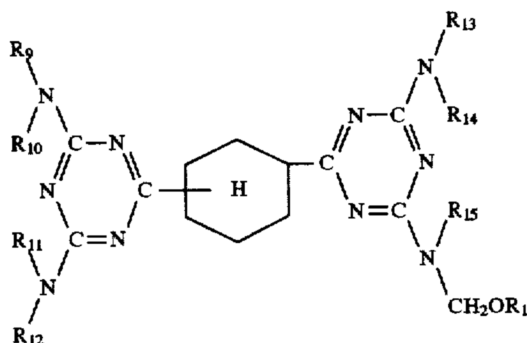
Formula (8)
