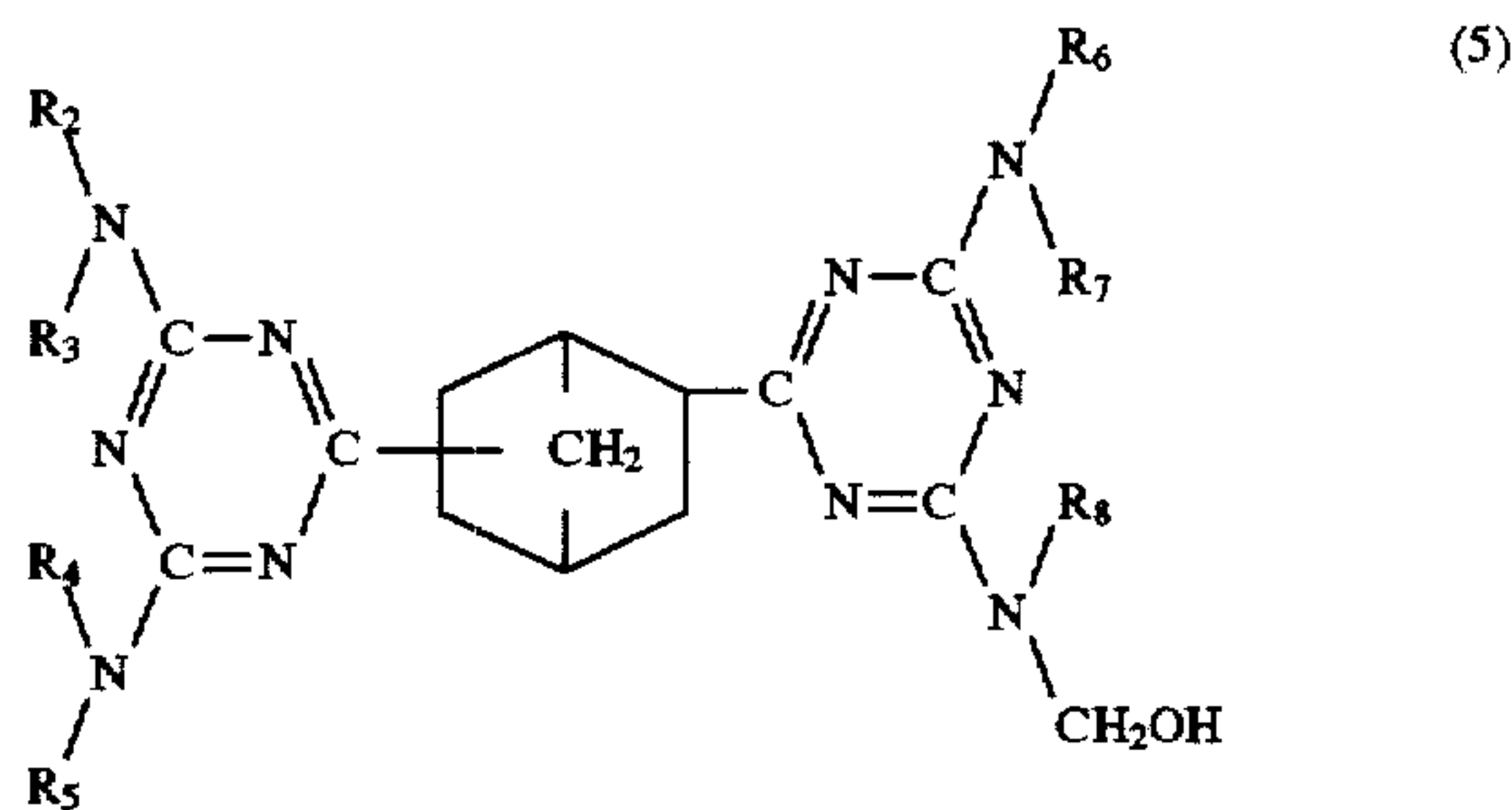
Formula (5)
