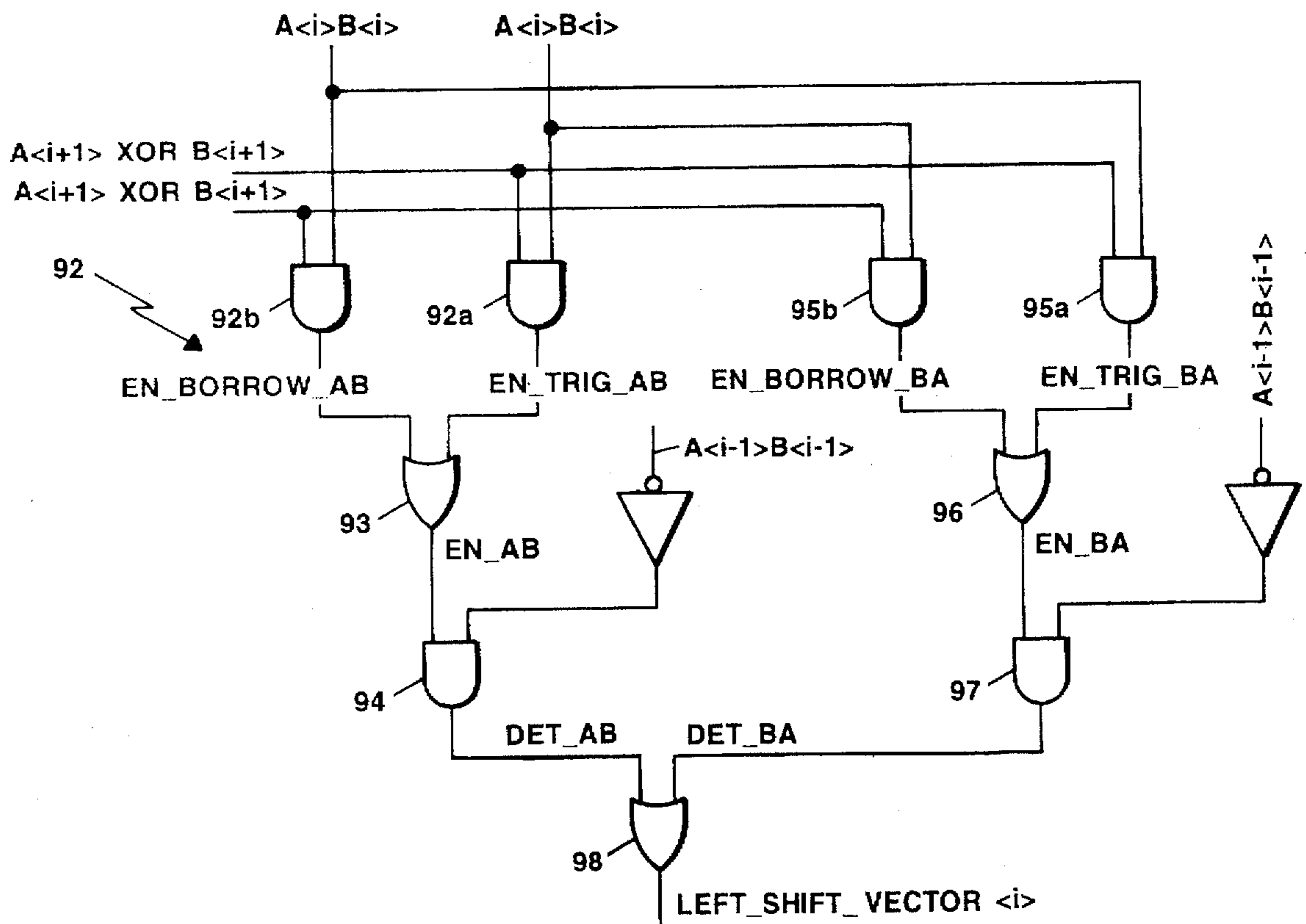
LOGIC FOR EXP_A = EXP_B (EDIFF=0)
