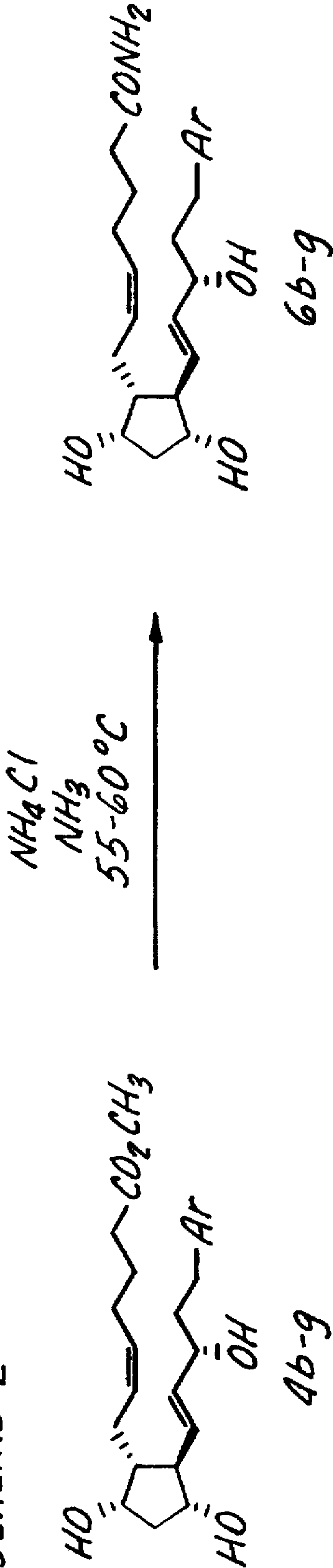
SCHEME 2
