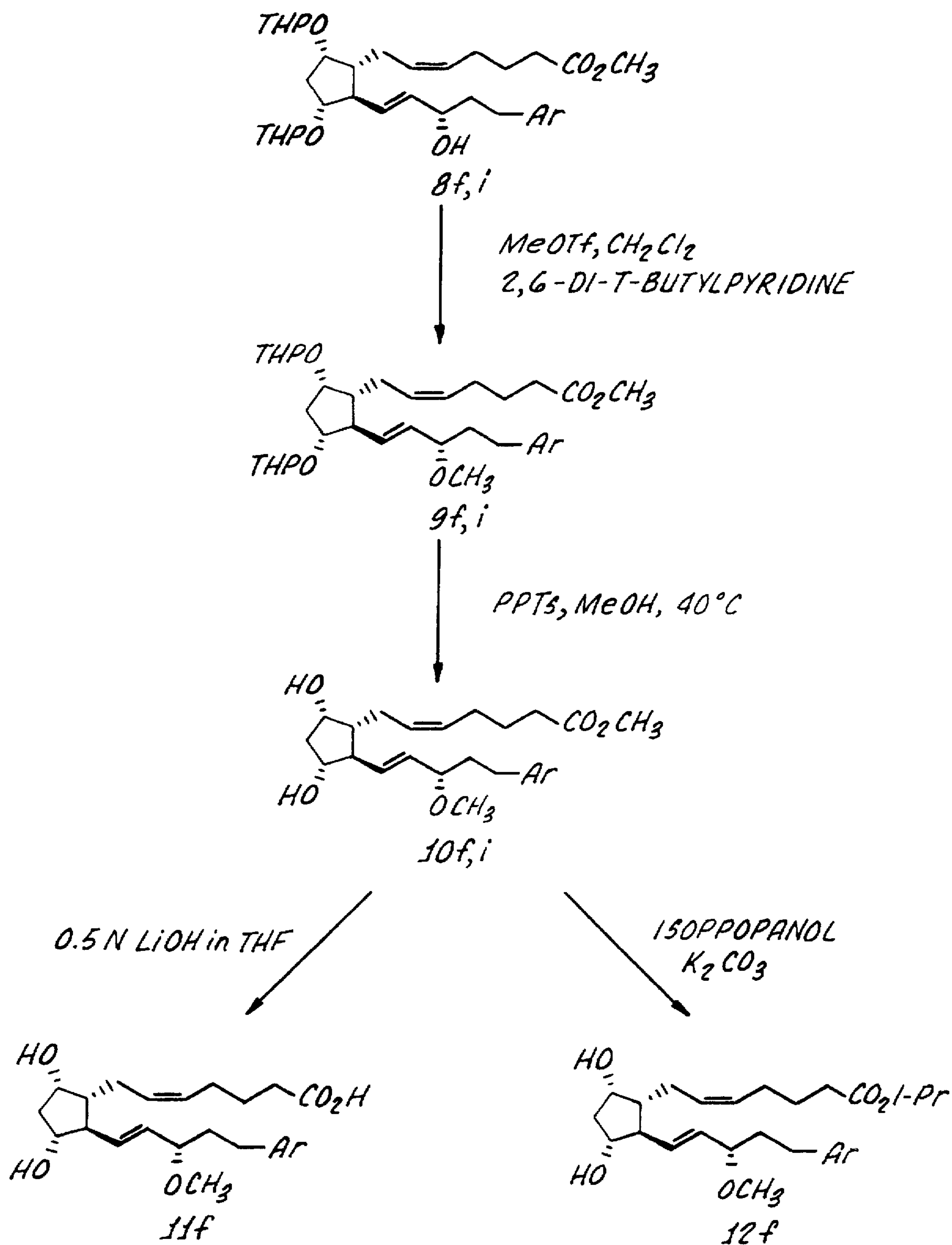
SCHEME 4
