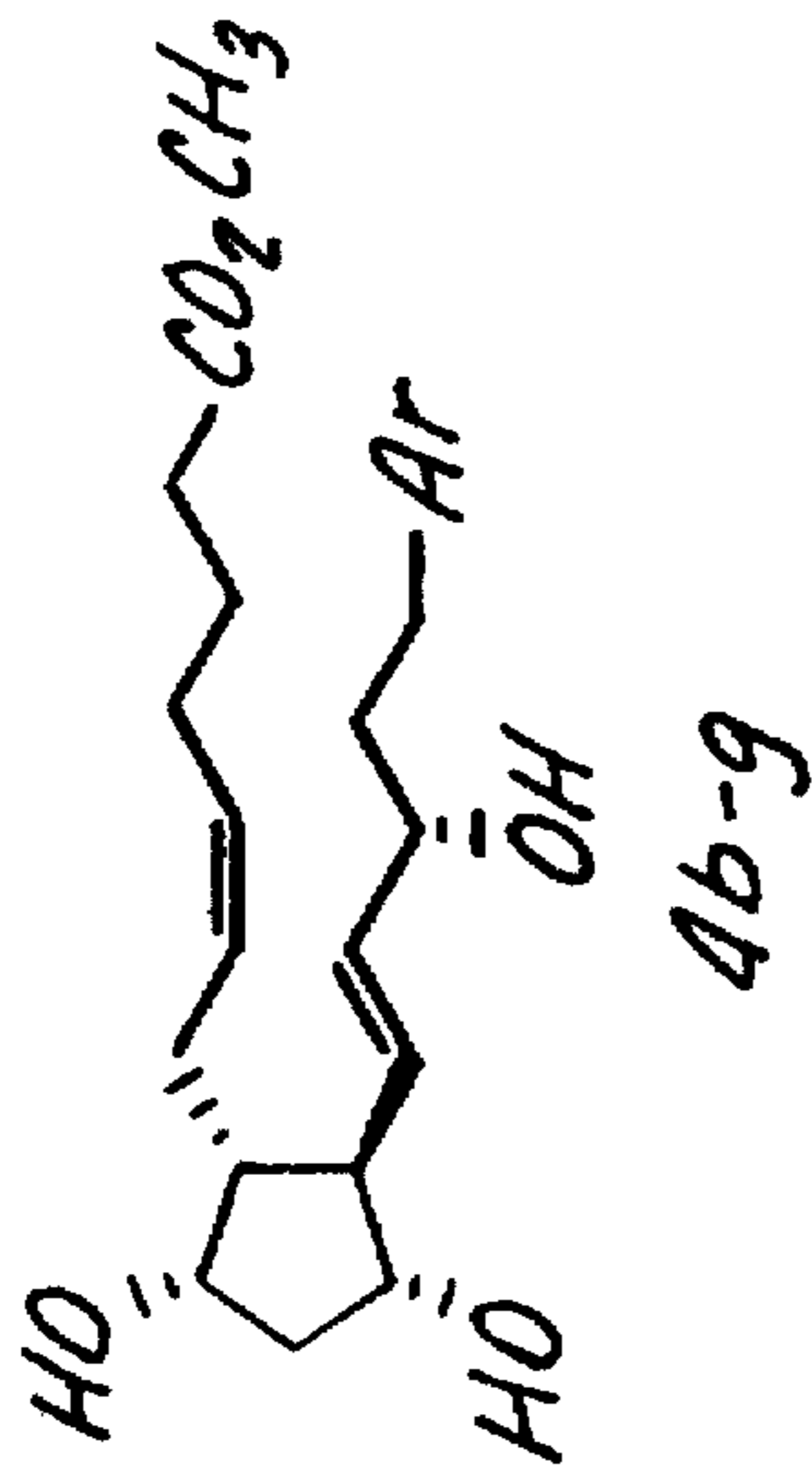
SCHEME 2
