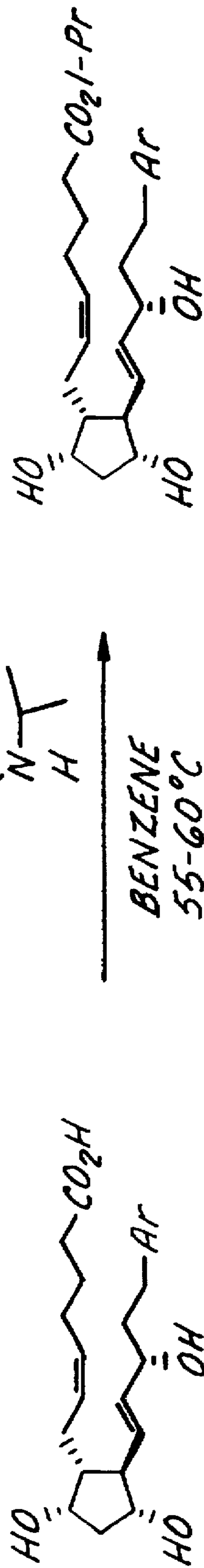
SCHEME 3
