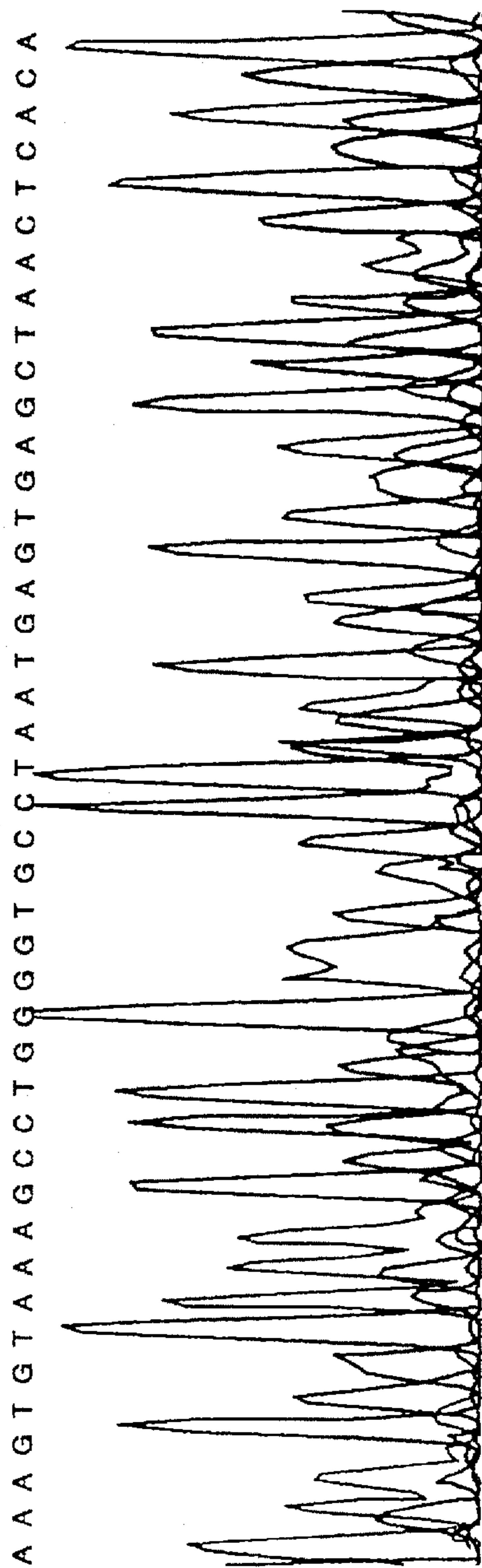
FIG. 8b. B. \Delta Taq Fluorescein-dUTP Cycle Sequencing Normalized Data
