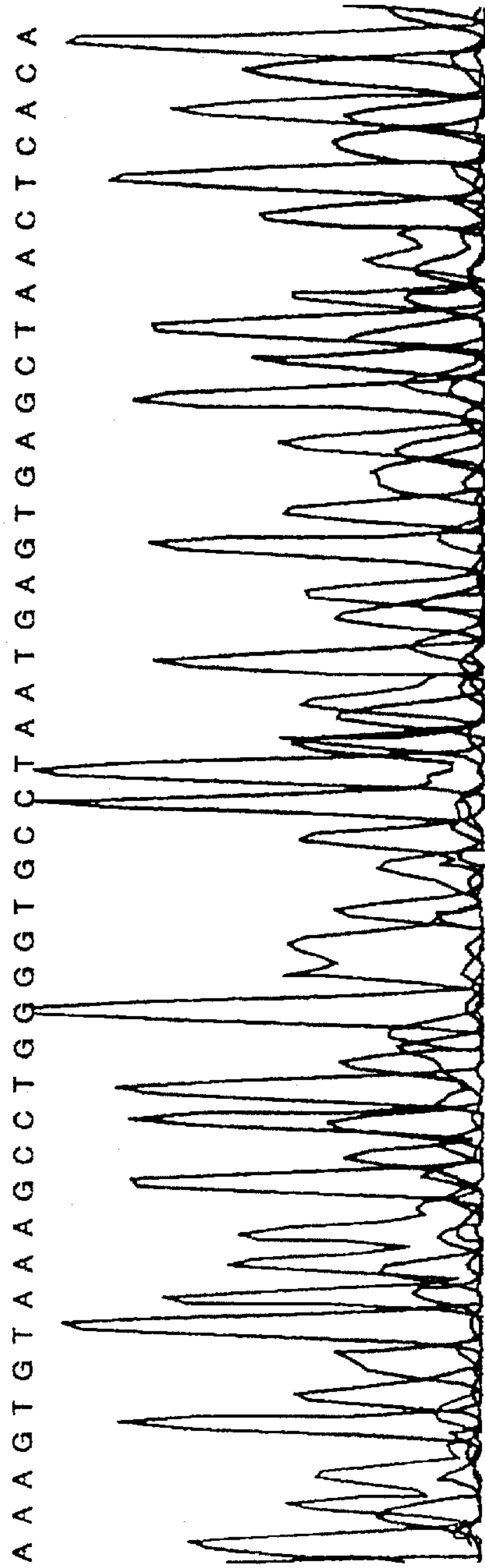
FIG. 8b. B. ΔTaq Fluorescein-dUTP Cycle Sequencing Normalized Data
