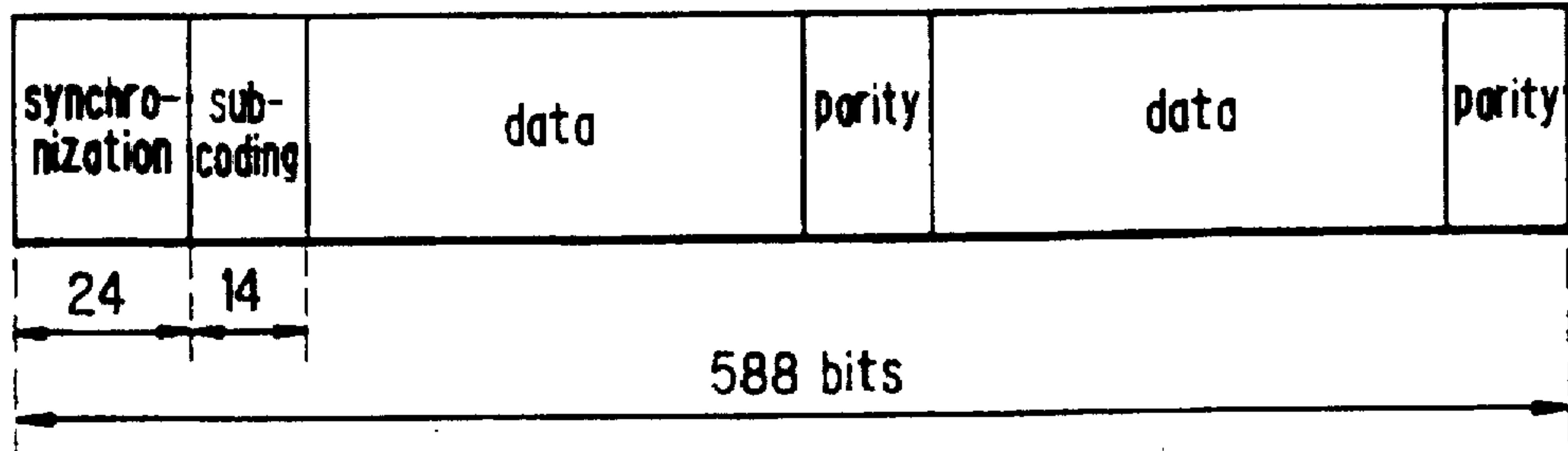
FIG. 8 (RELATED ART)
