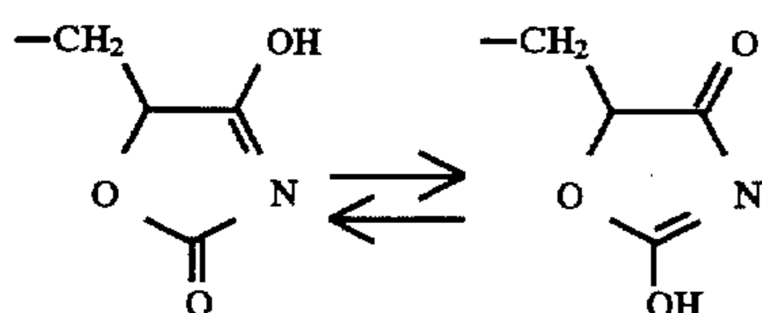
Scheme \gamma
