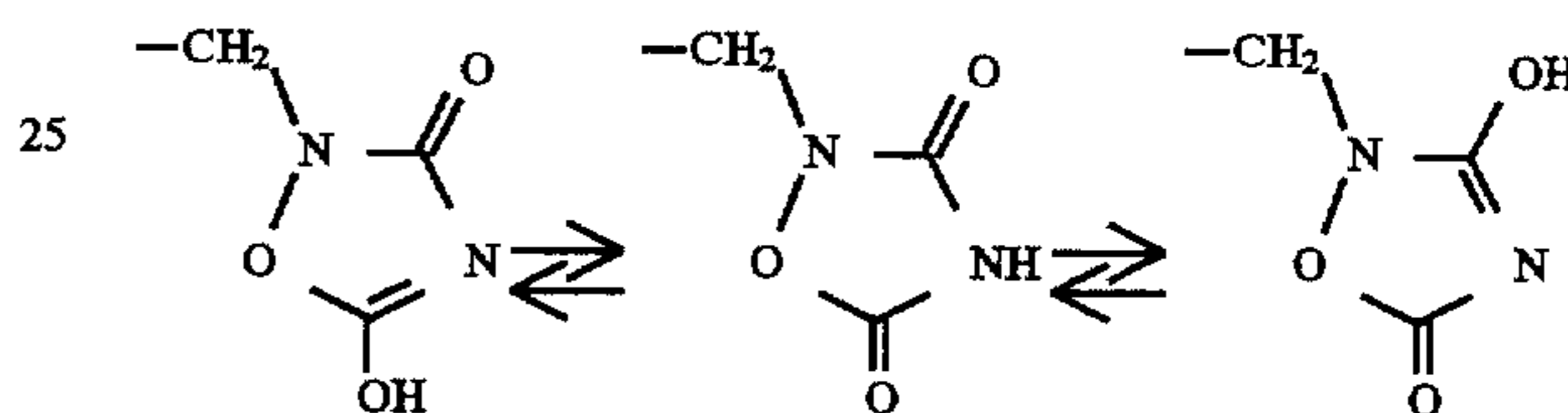
Scheme \delta
