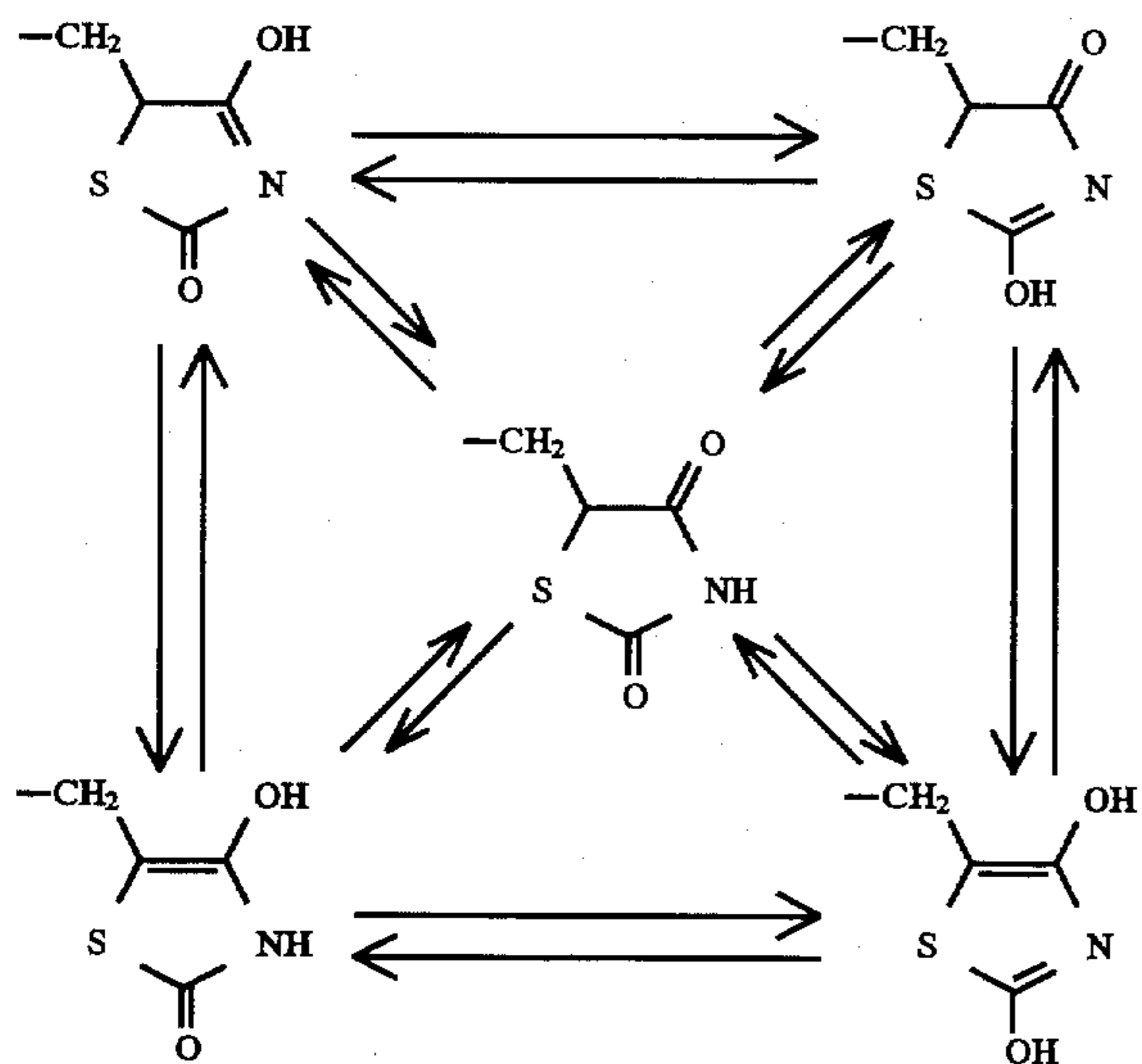
Scheme \alpha
