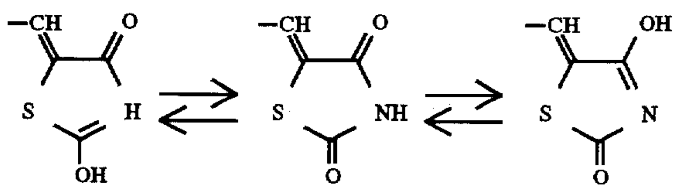
Scheme \beta
