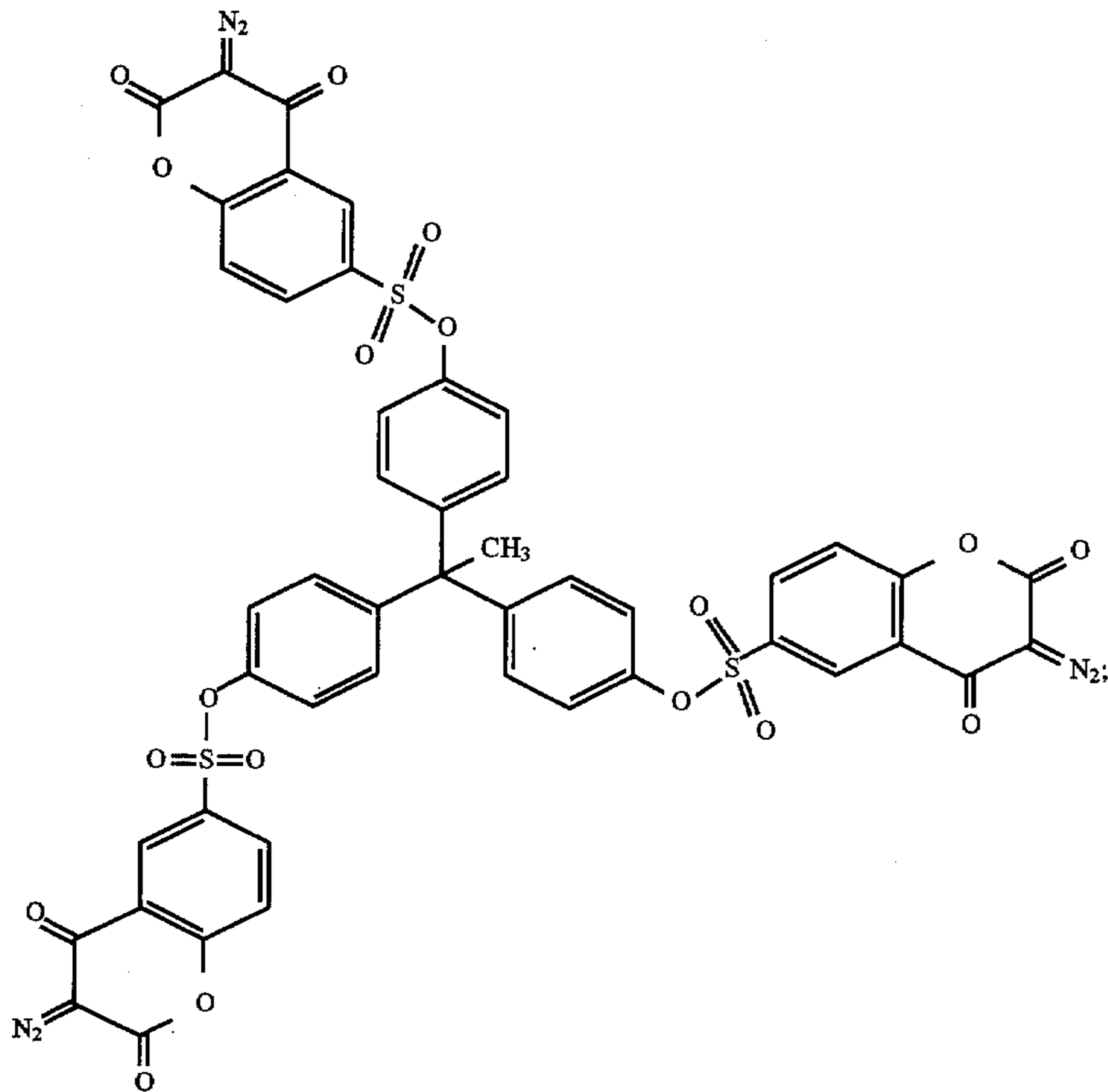
30 4,4'-bis(3-diazo-4-oxo-3,4-dihydrocoumarin-6-sulfonyloxy)benzophenone having the formula:
