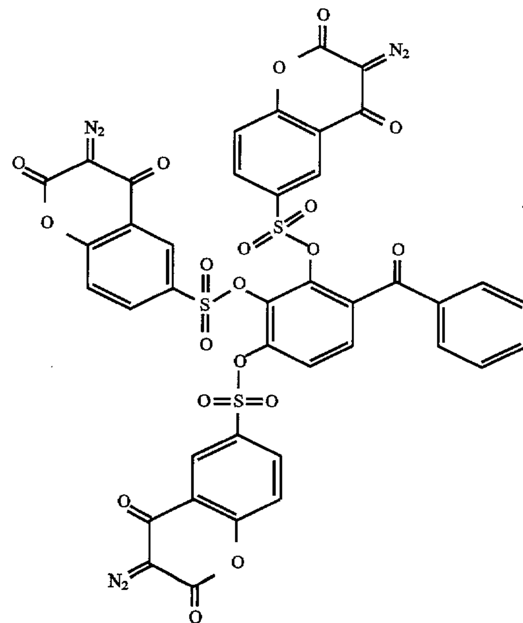
55 4,8-bis(3-diazo-4-oxo-3,4-dihydrocoumarin-6-sulfonyloxymethyl)tricyclo[5.2.1.0. 2,6 ]decane having the formula:
