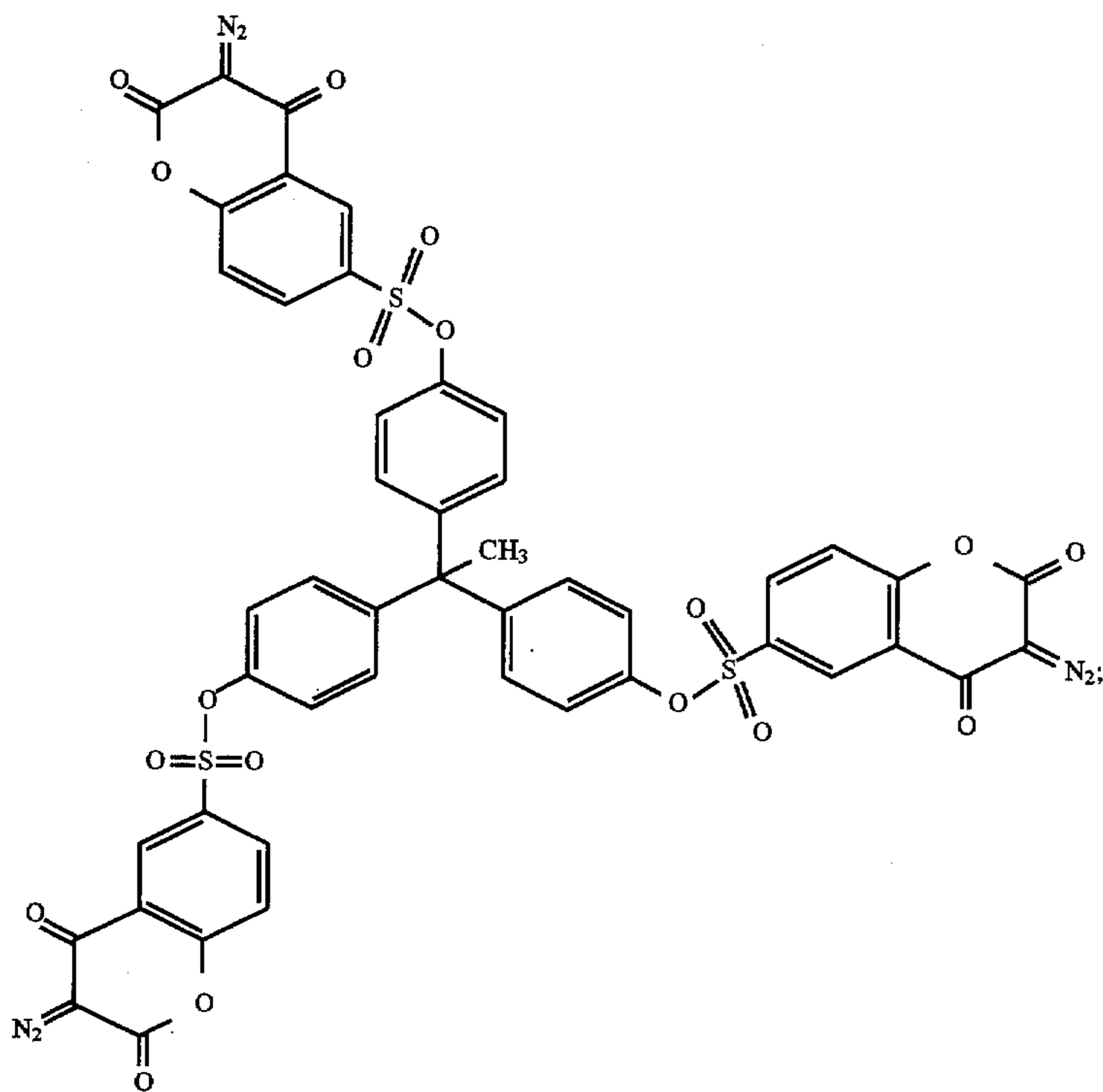
4,4'-bis(3-diazo-4-oxo-3,4-dihydrocoumarin-6-sulfonyloxy)benzophenone having the formula:
