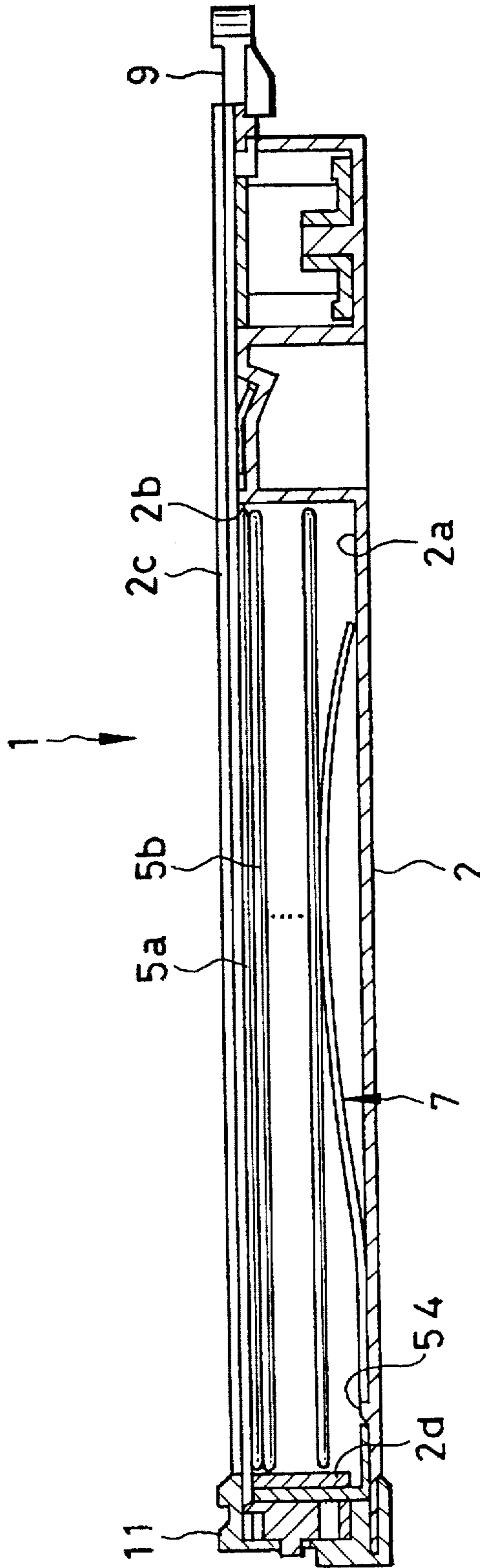
FIG. 21 (PRIOR ART)
