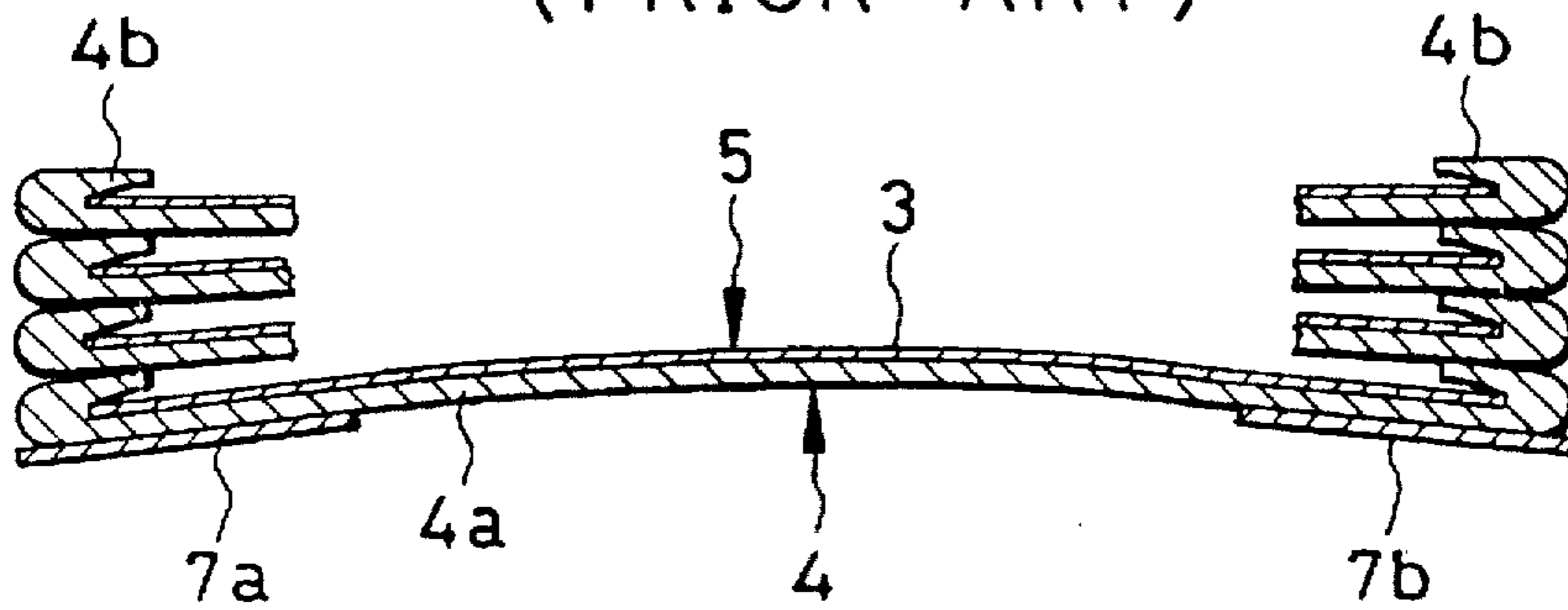
FIG. 25 (PRIOR ART)
