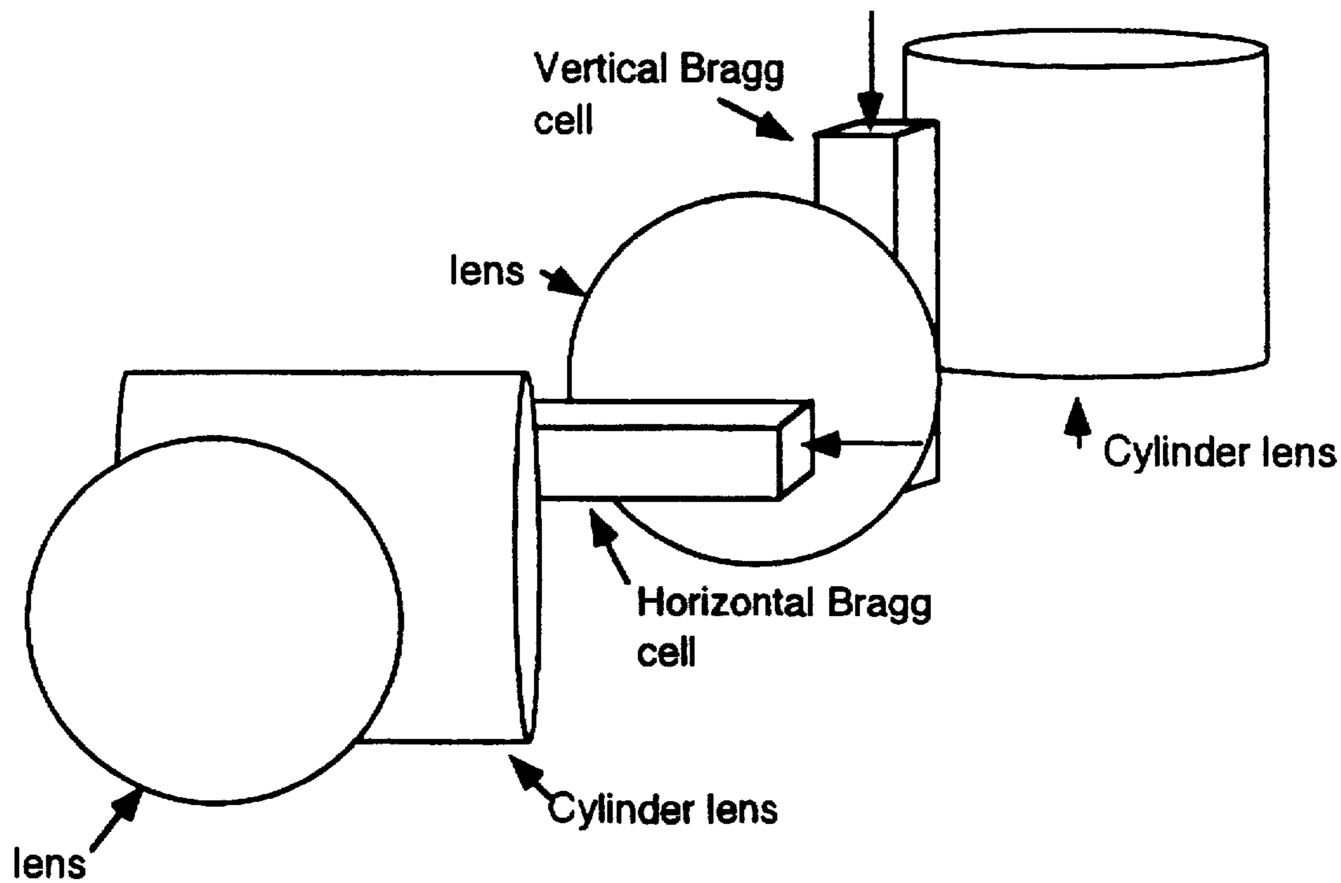
Fig 36 One dimensional cell replacement for a two dimensional Bragg cell
