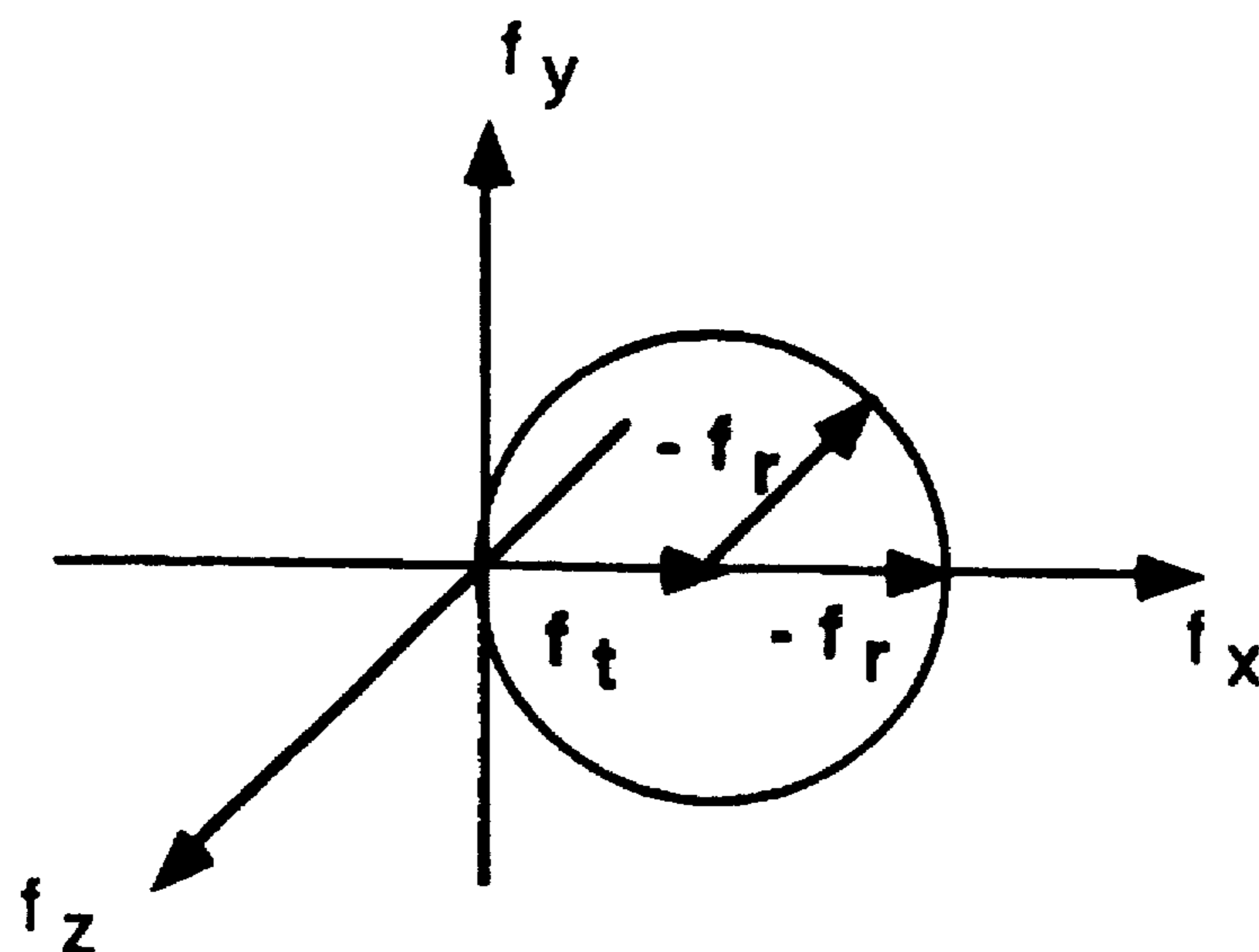
Figure 32 The Trajectory of Samples in Frequency Space for a fixed Transmitter and Target with a Moving Receiver or Multiple Receivers
