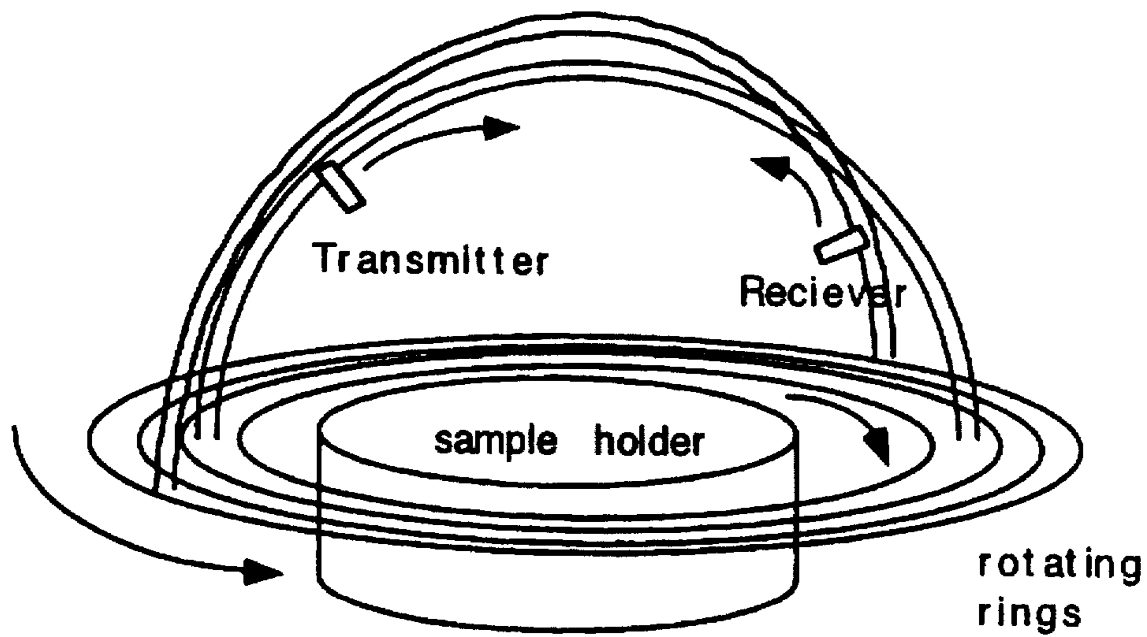
Figure 30 An Alternate Synthetic Aperture Microscope
