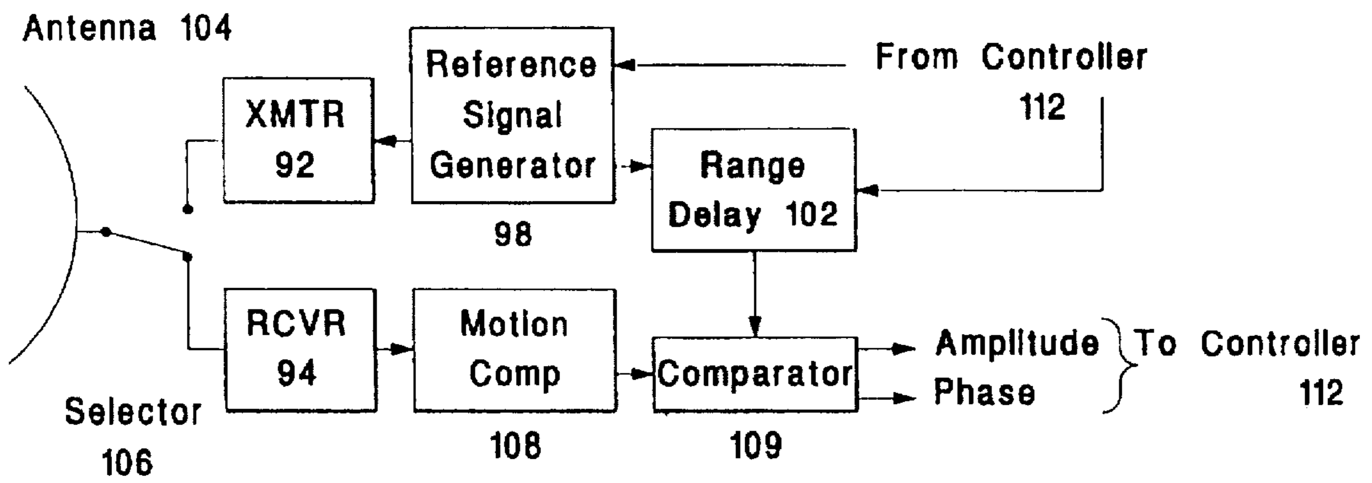
SAR System 91
