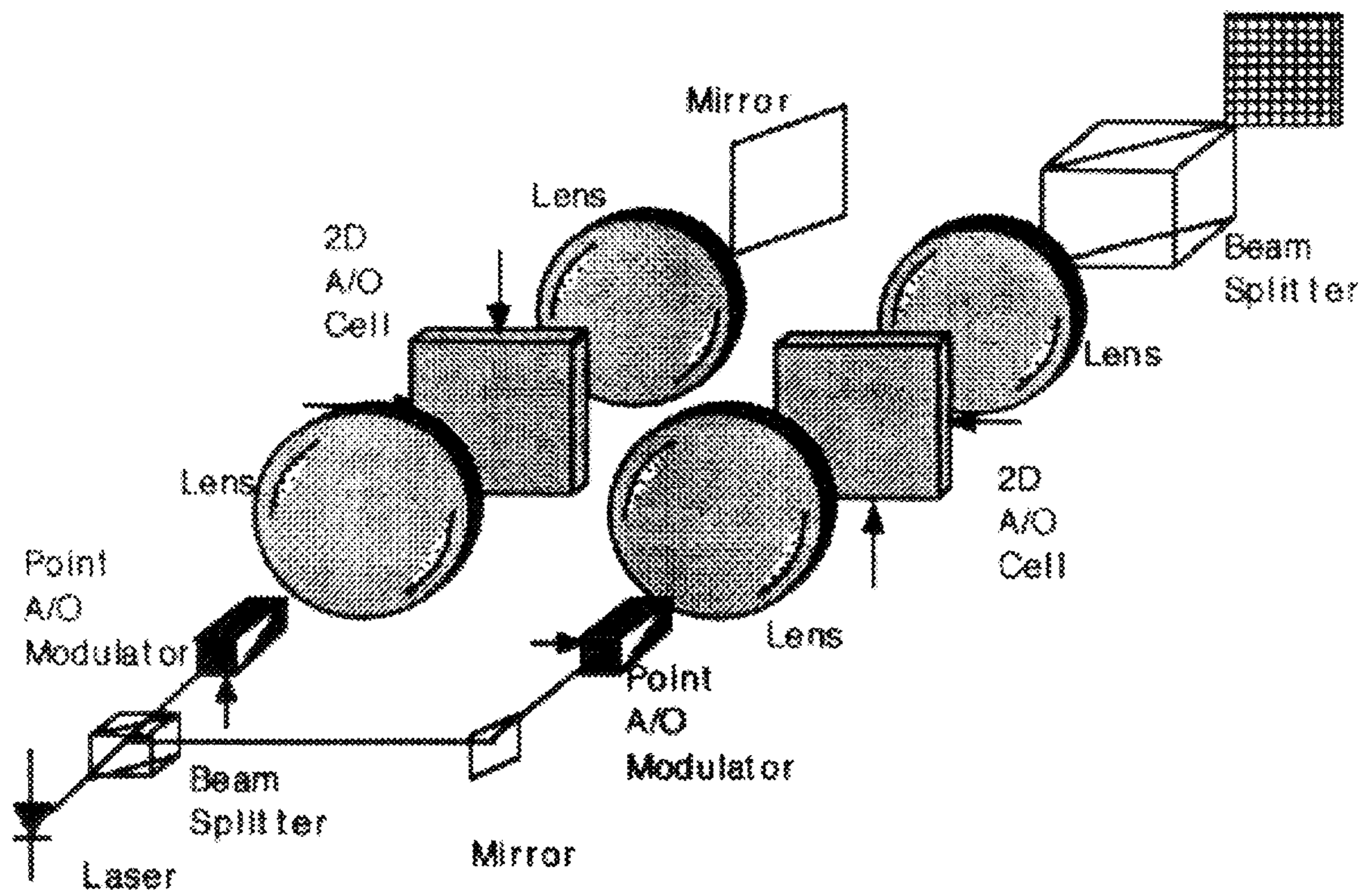
Figure 39 Symmetrical Mach Zehnder ImSyn
