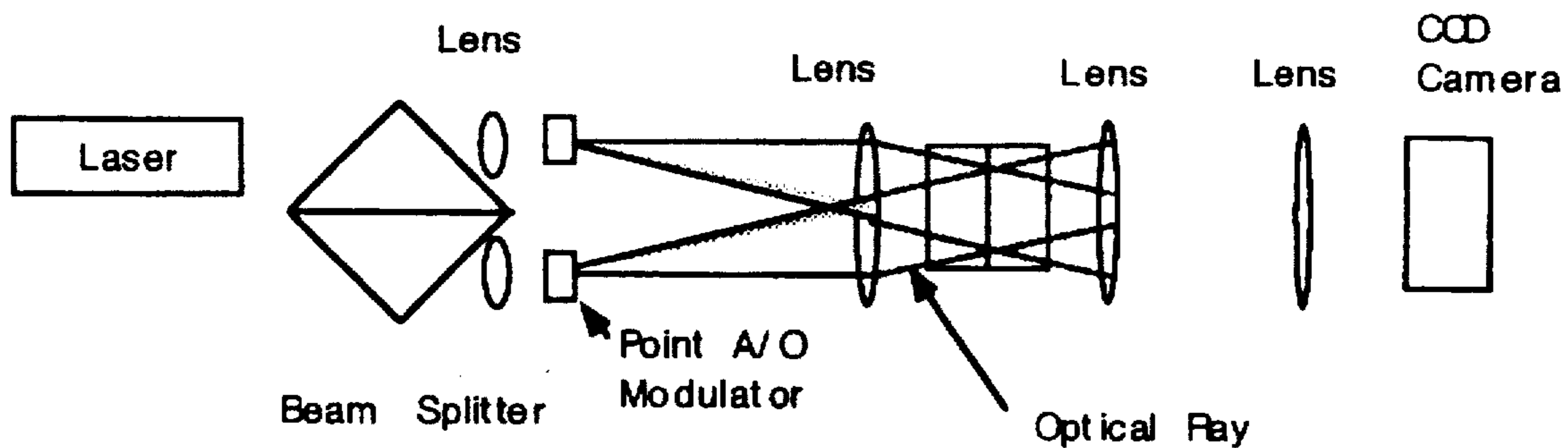
Figure 38 Example of a Common Path ImSyn
