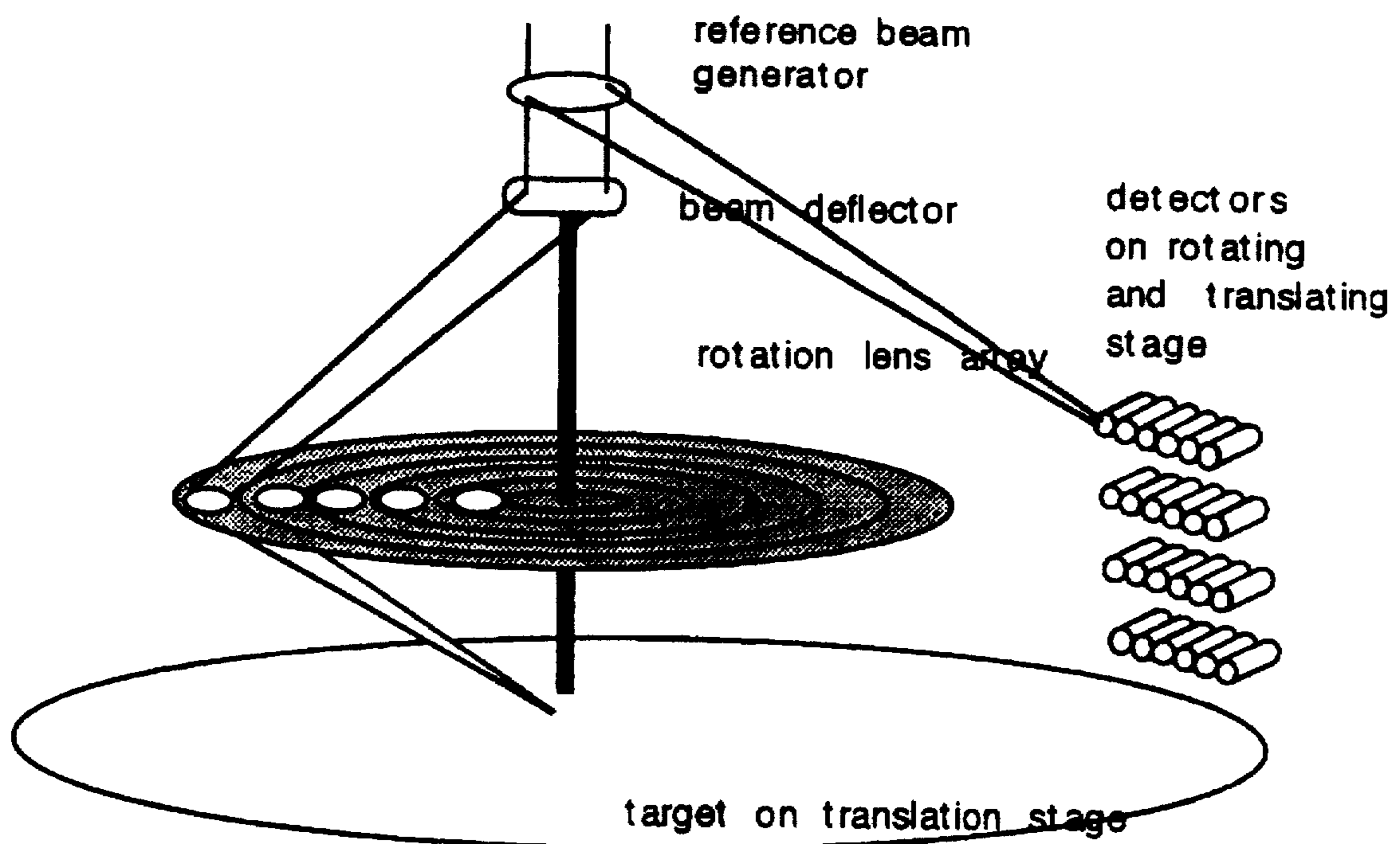
Figure 29 Synthetic Aperture Microscope with Translating Sample
