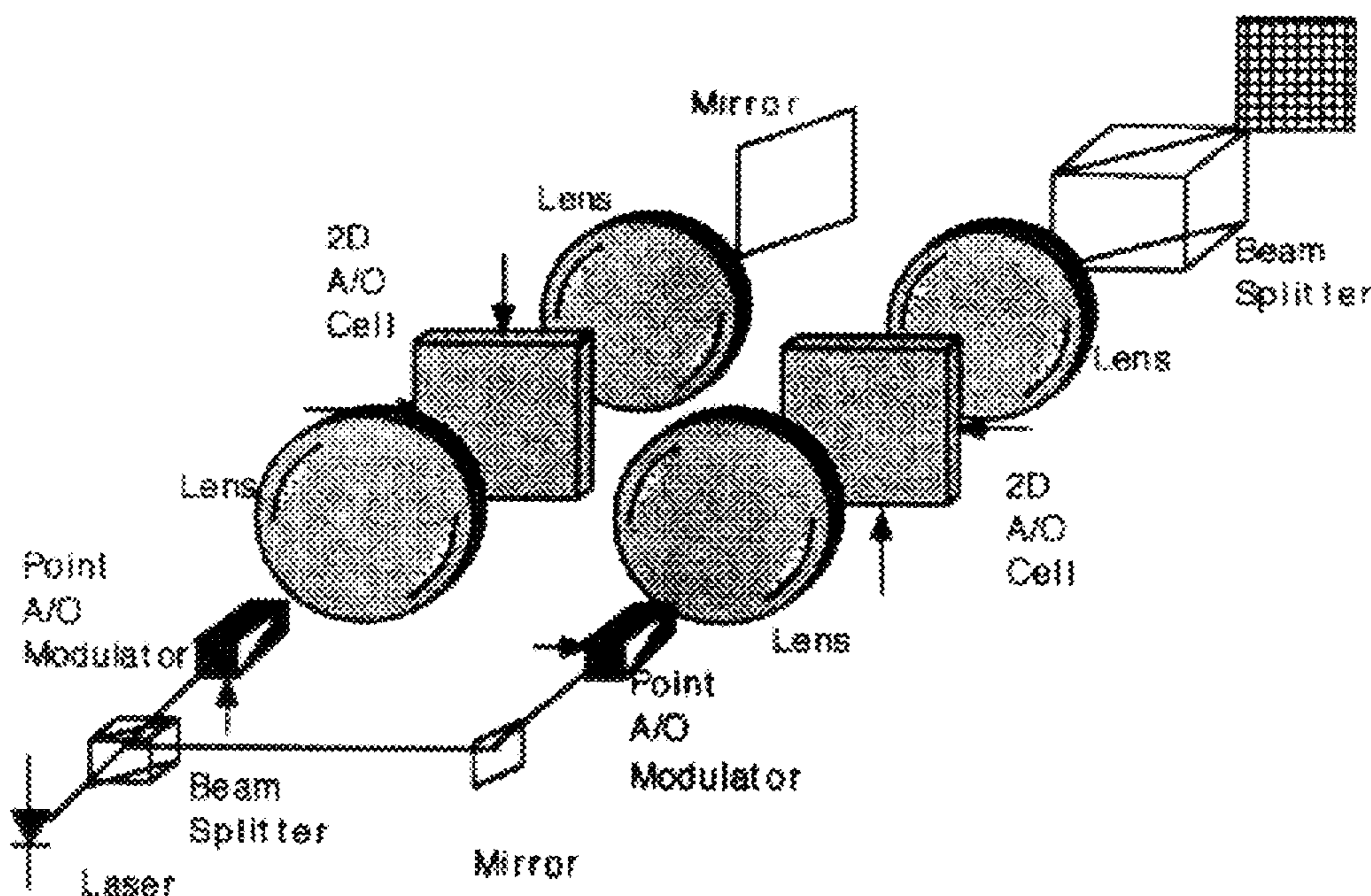
Symmetrical Mach Zehnder ImSyn
