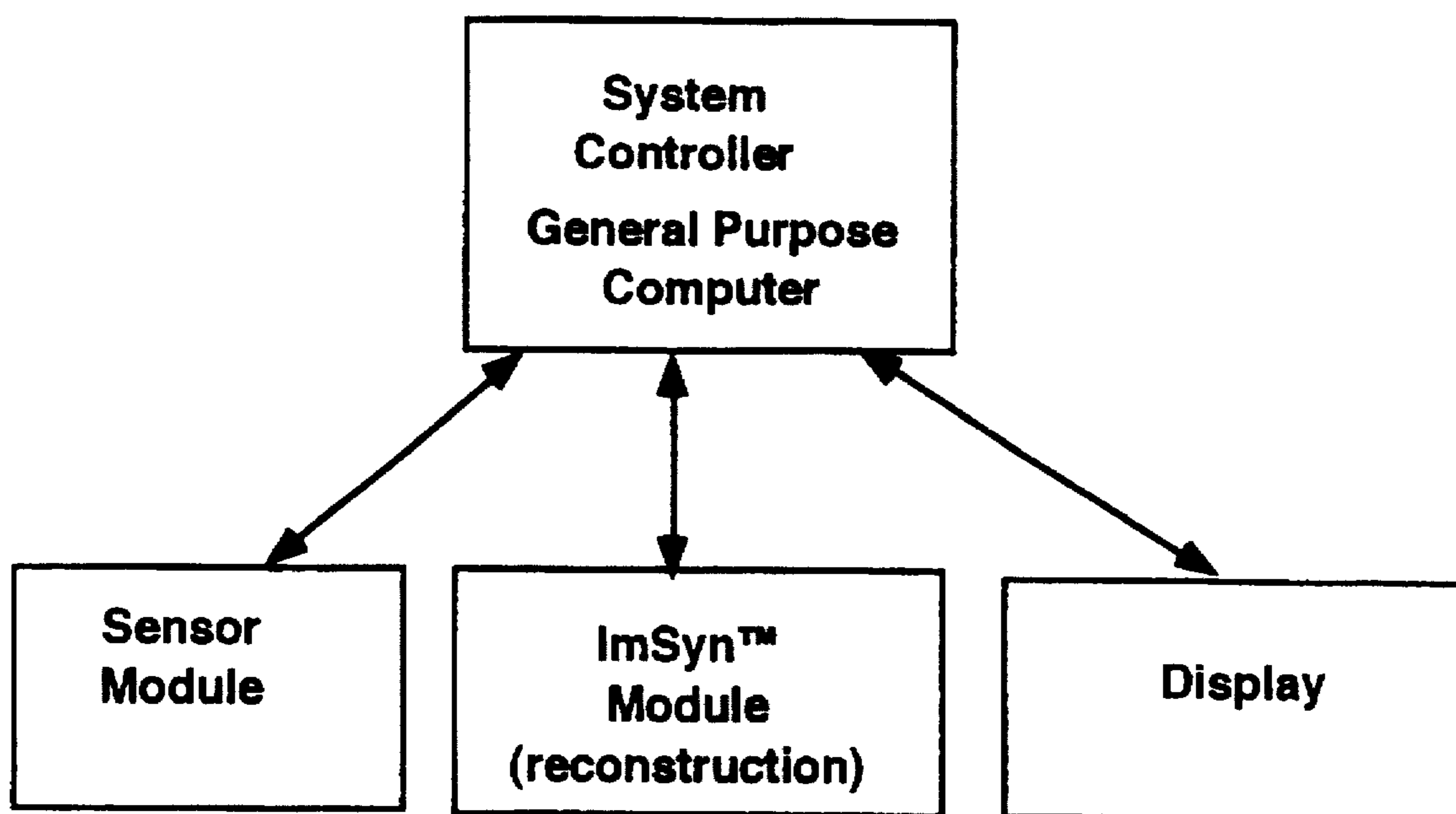
Figure 27 The Synthetic Aperture Microscope
