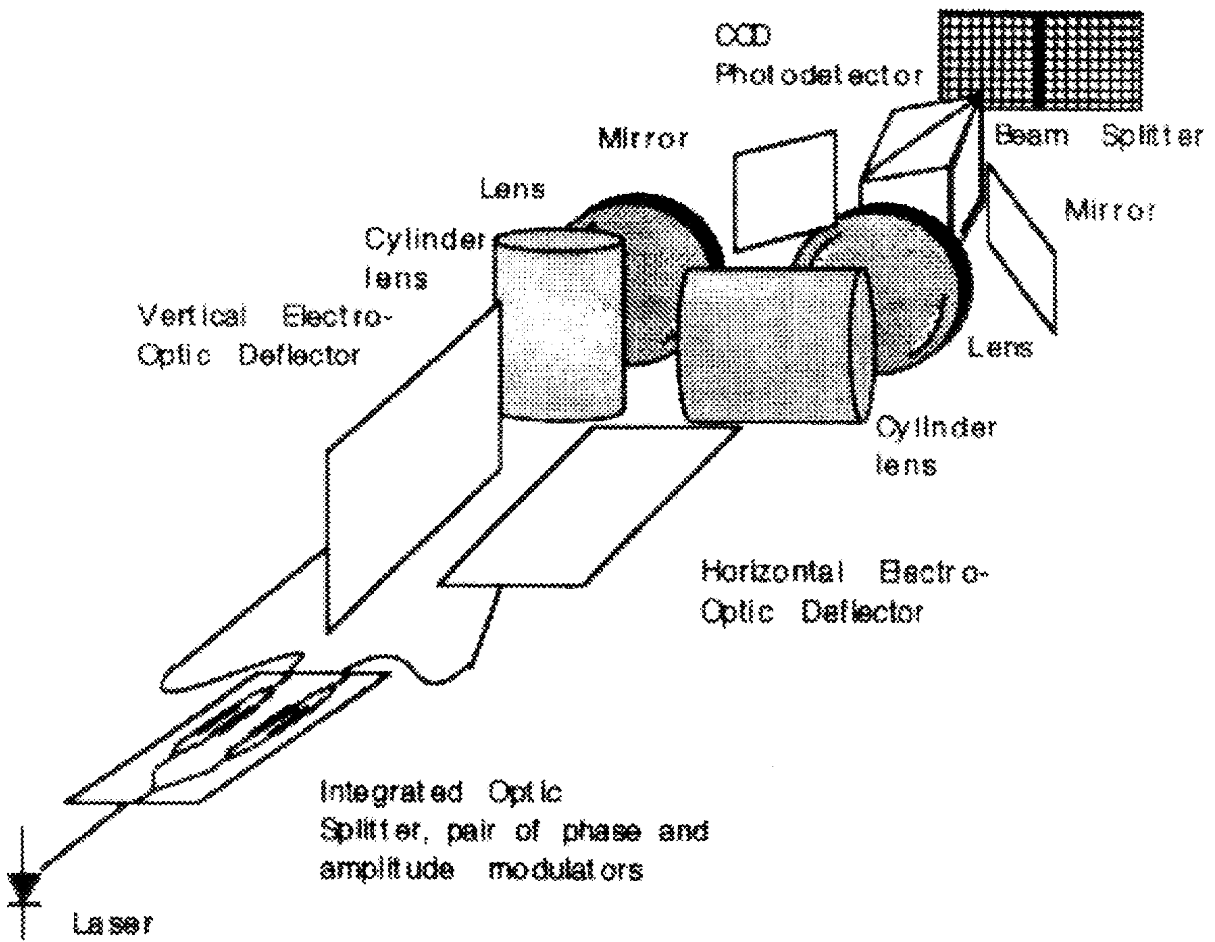
Figure 41 Electro-optic random access ImSyn
