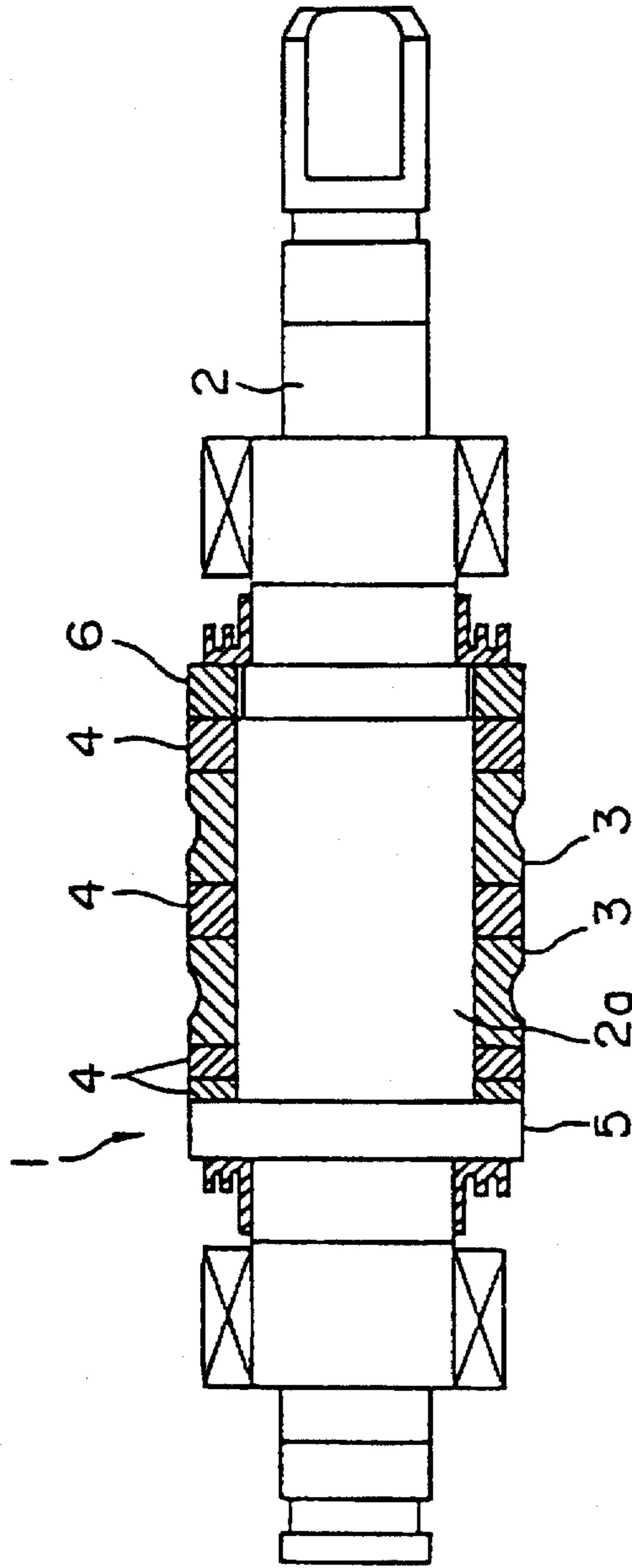
FIG. 2 Prior Art
