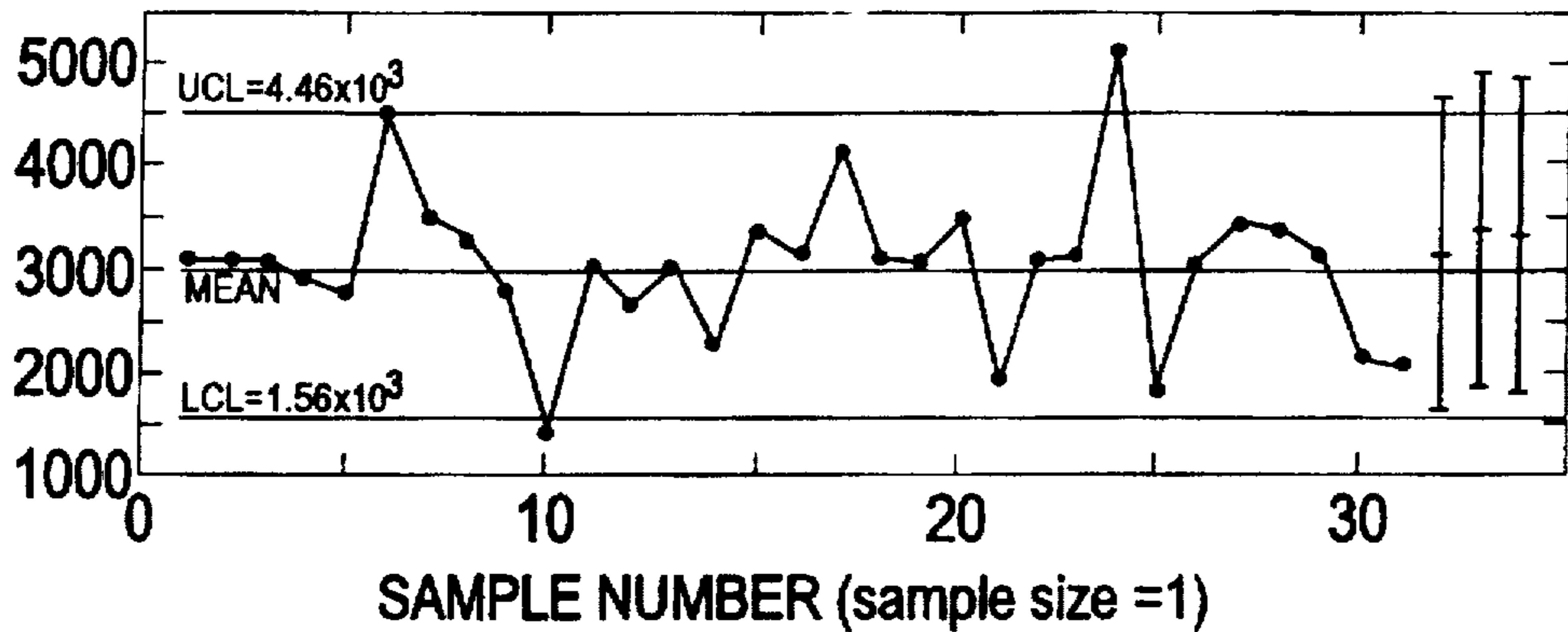
ABC XR CHARTS: RIE PROCESS
