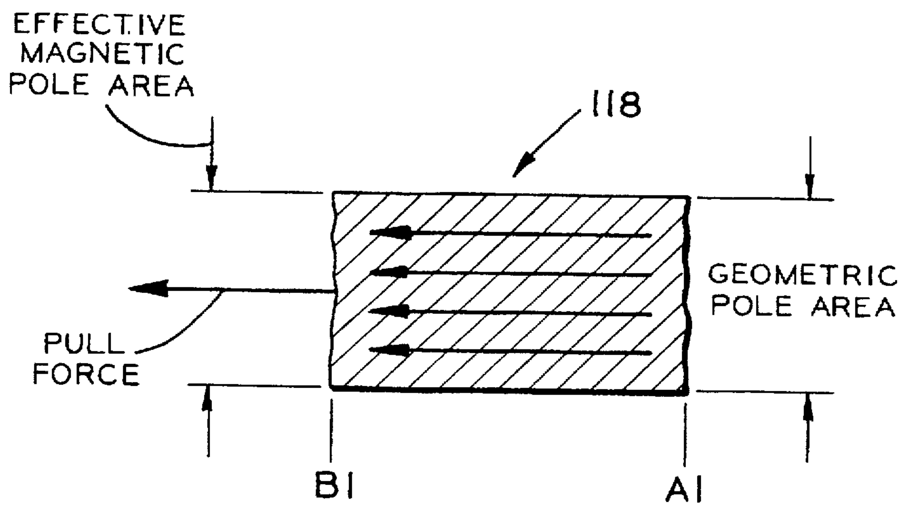
FIG. 4 (PRIOR ART)
