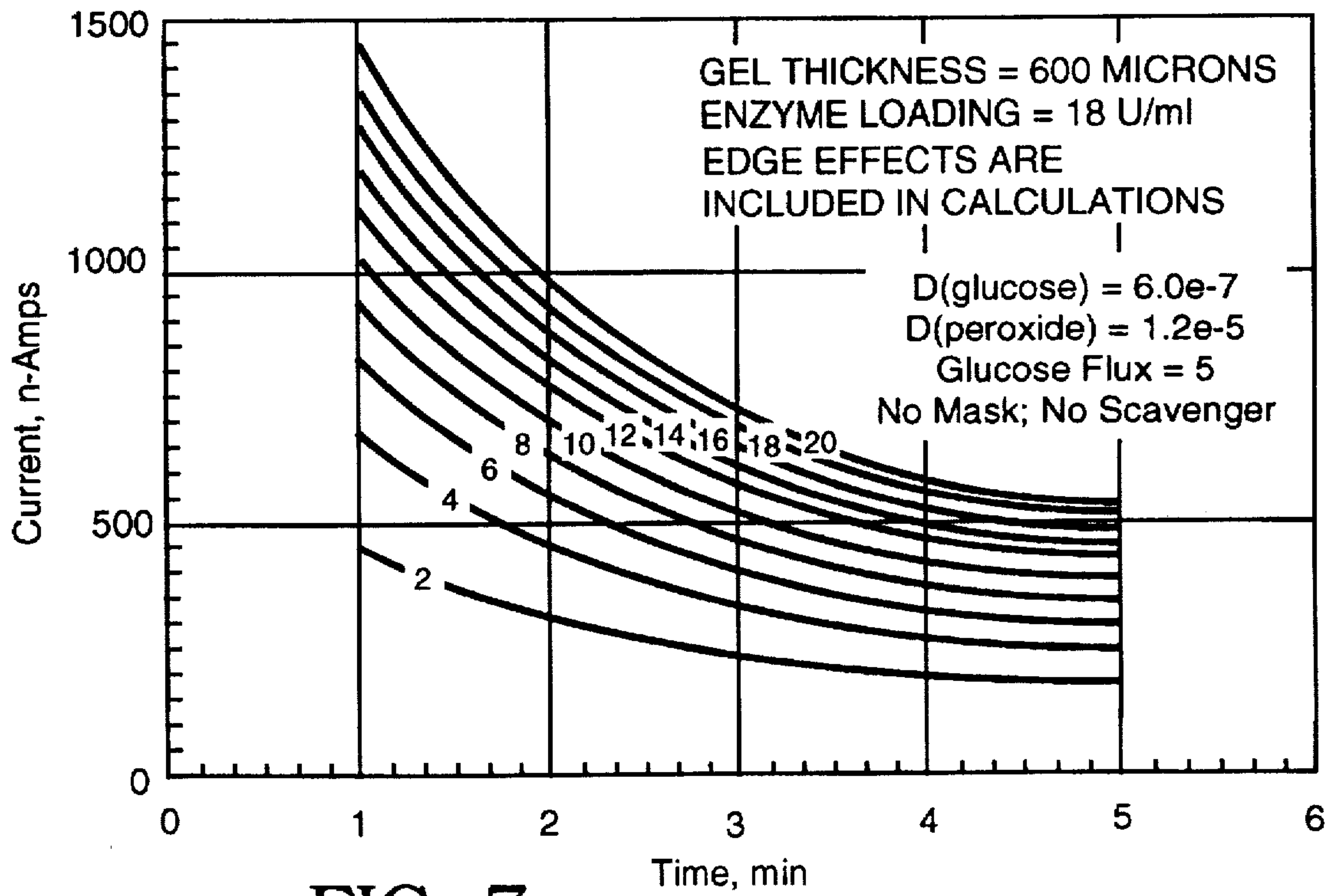
CURRENT FOR DIFFERENT INTERVALS AS A FUNCTION OF TIME
