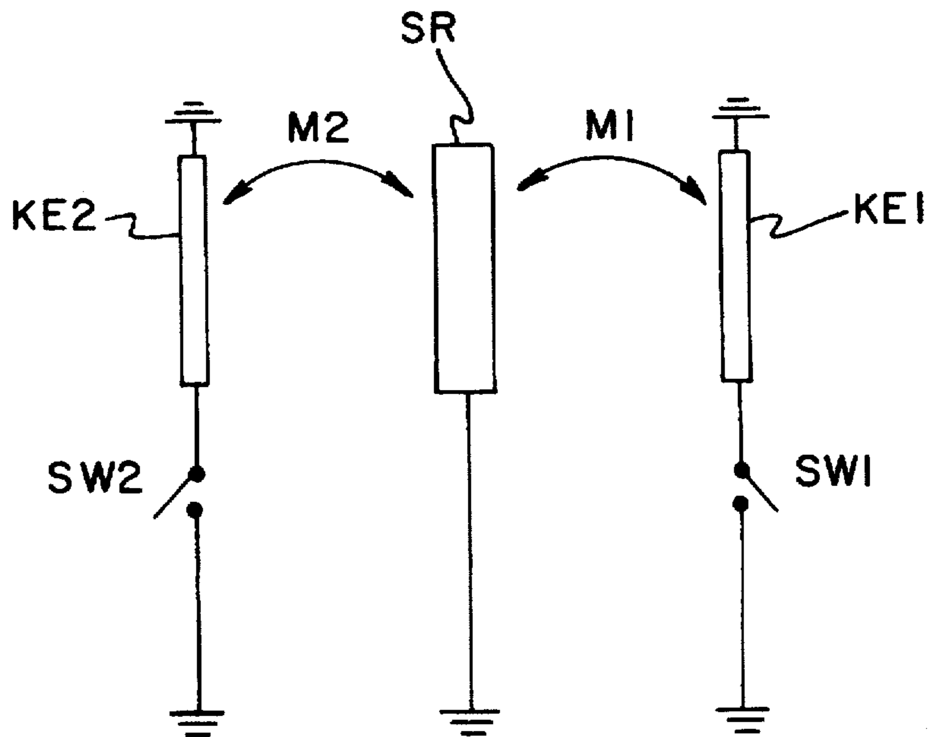
FIG. 2 (PRIOR ART)
