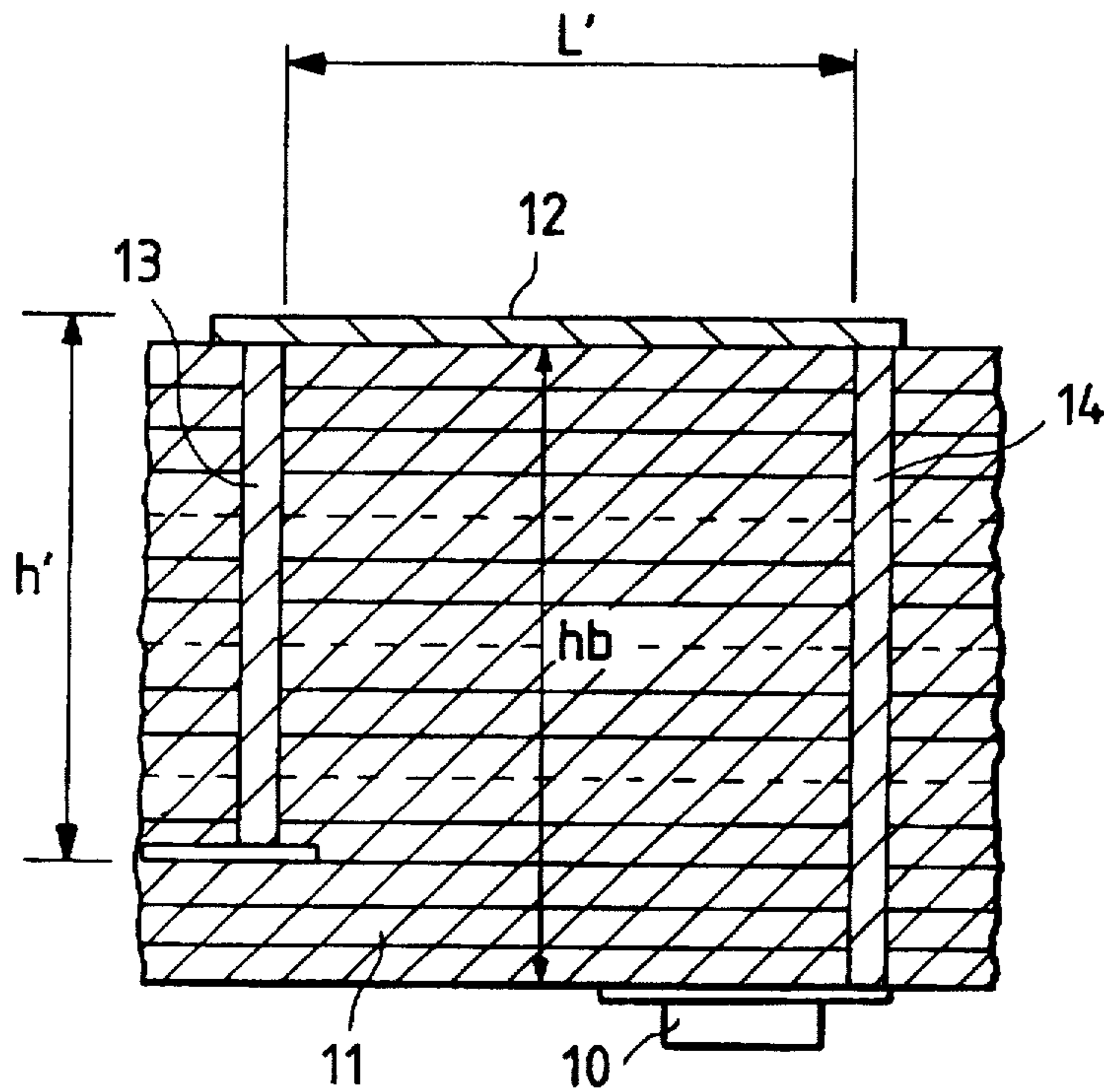
FIG. 10 PRIOR ART
