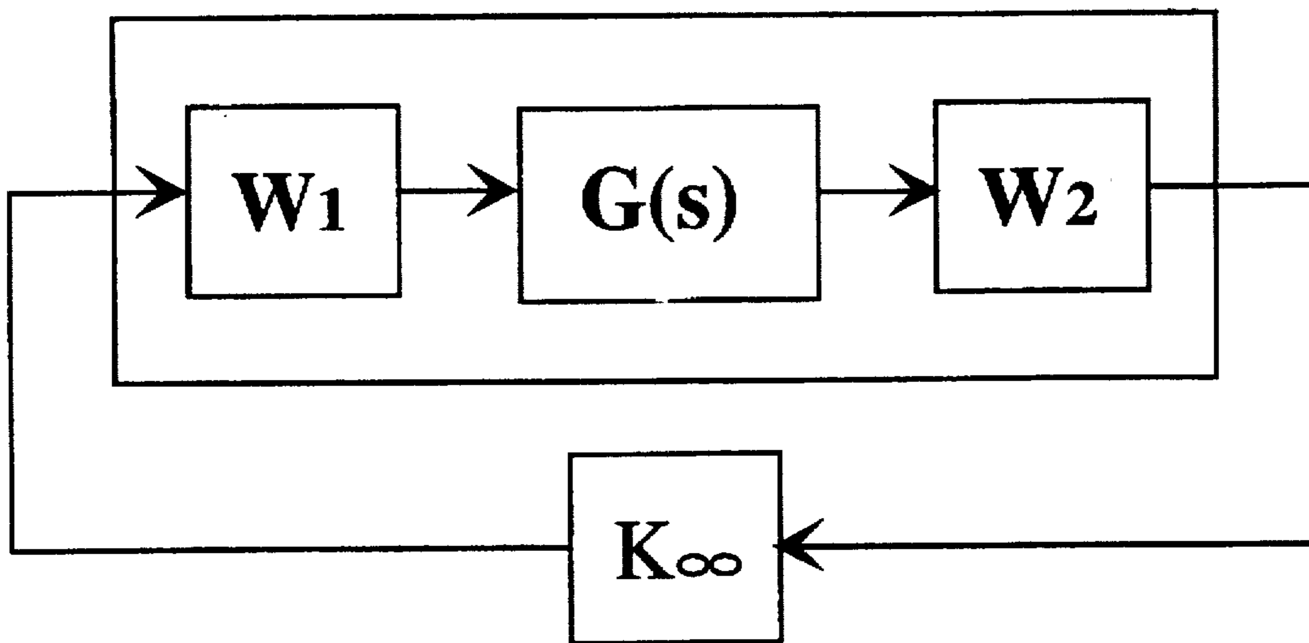
I/O FILTER H-INFINITY SYNTHESIS
