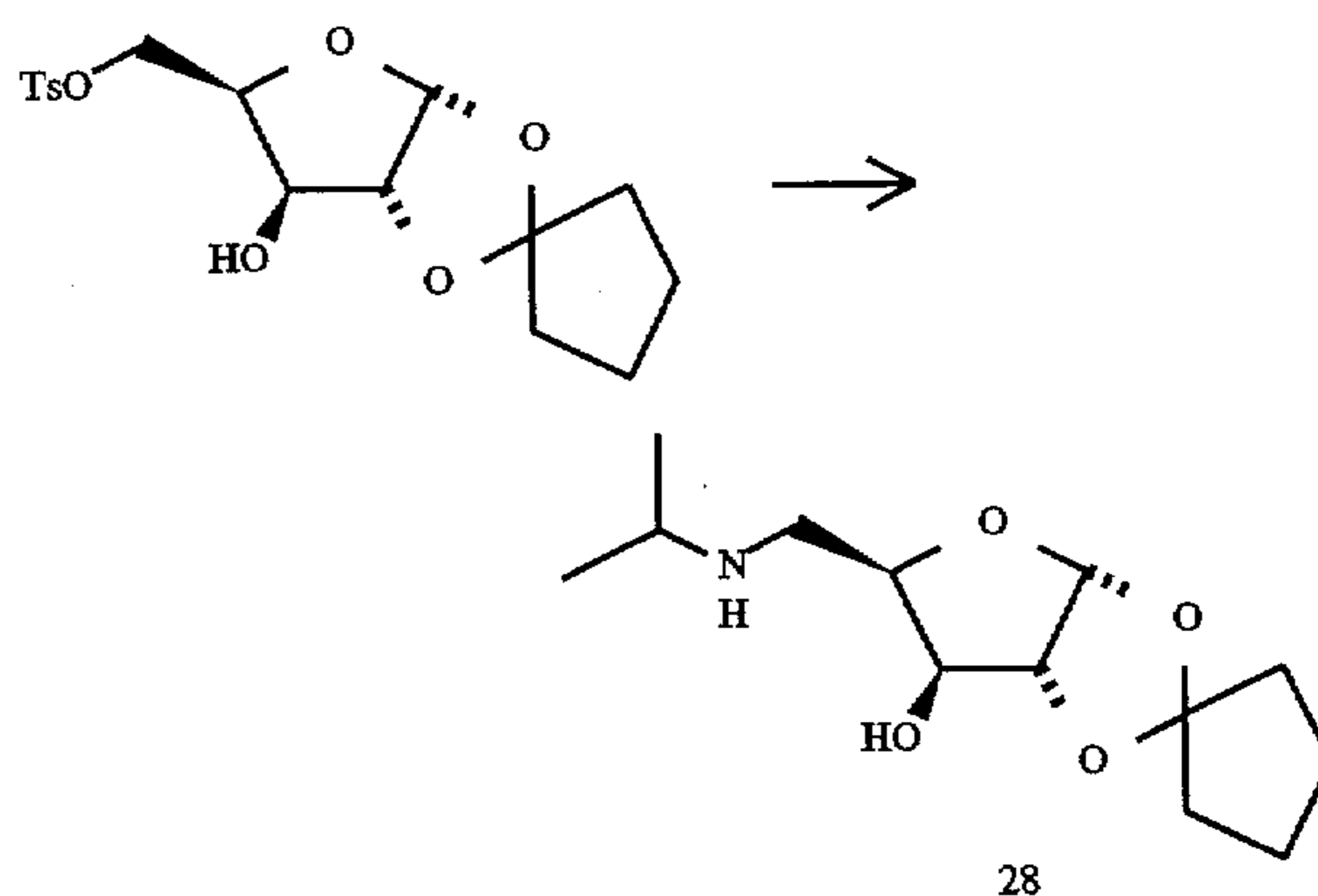
1,2-O-dicyclopentylidene-5'-isopropylamine-D-xylofuranose (28)
