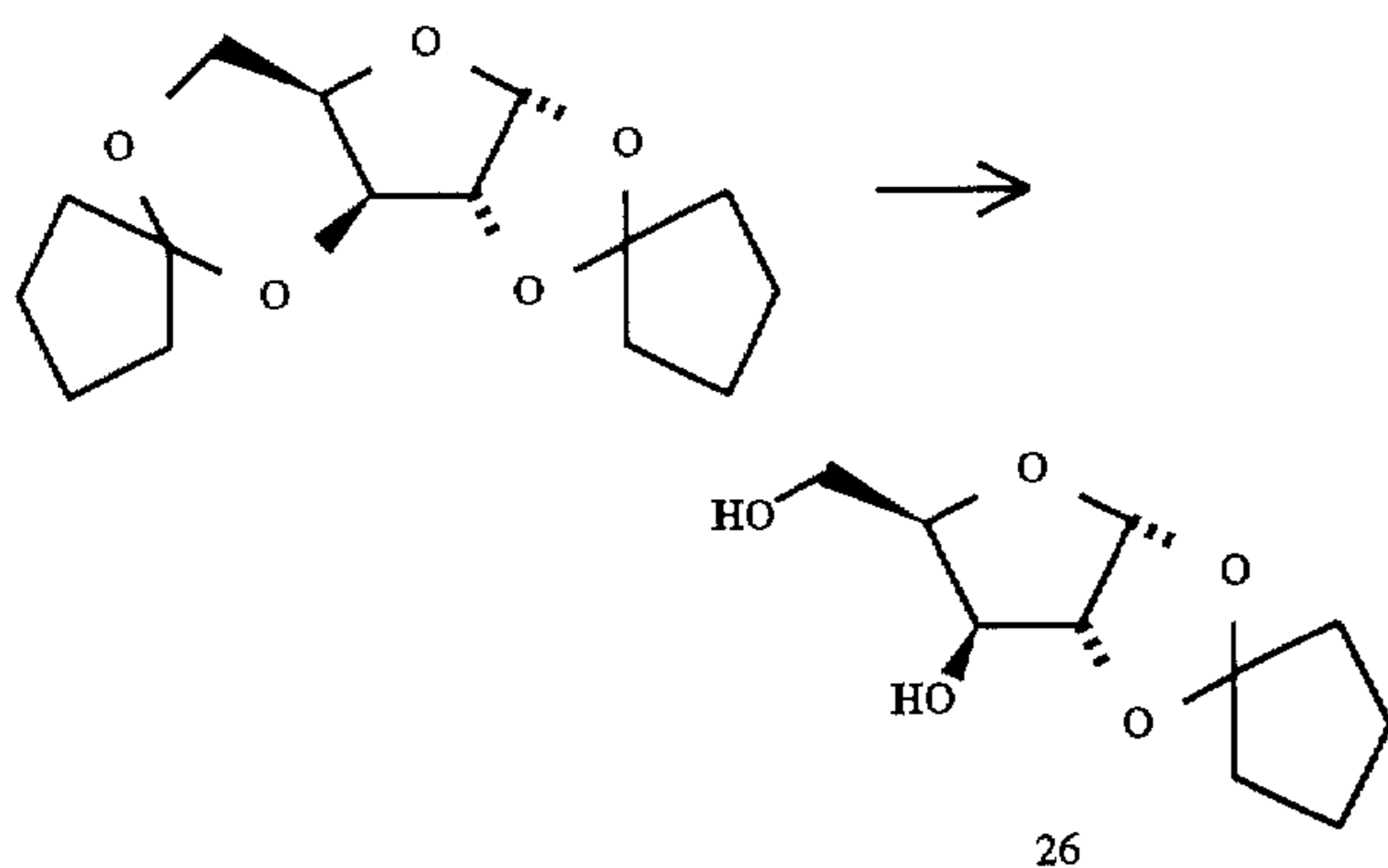
1,2-O-cyclopentylidene-D-xylofuranose (26)
