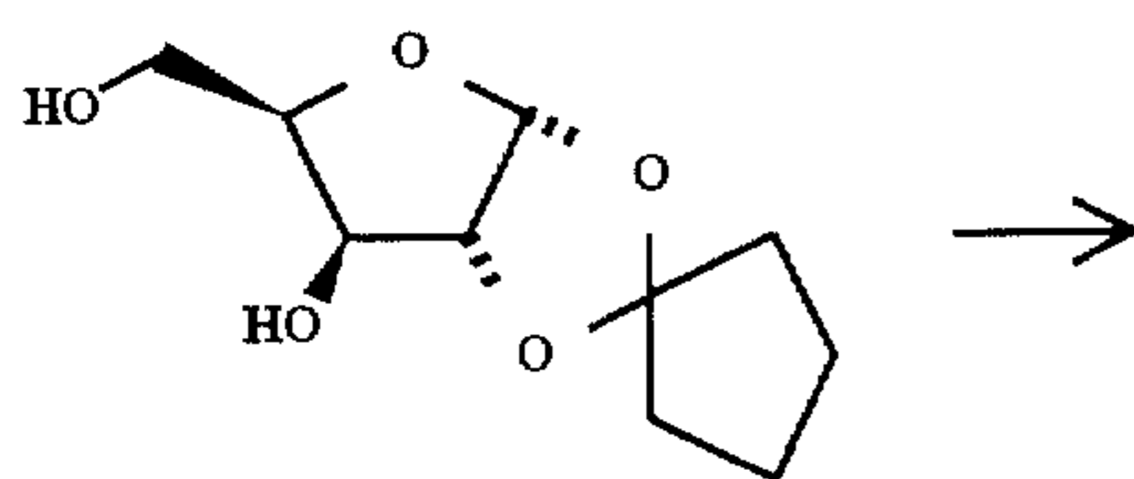
1,2-O-cyclopentylidene-5'-O-tosyl-D-xylofuranose (27)
