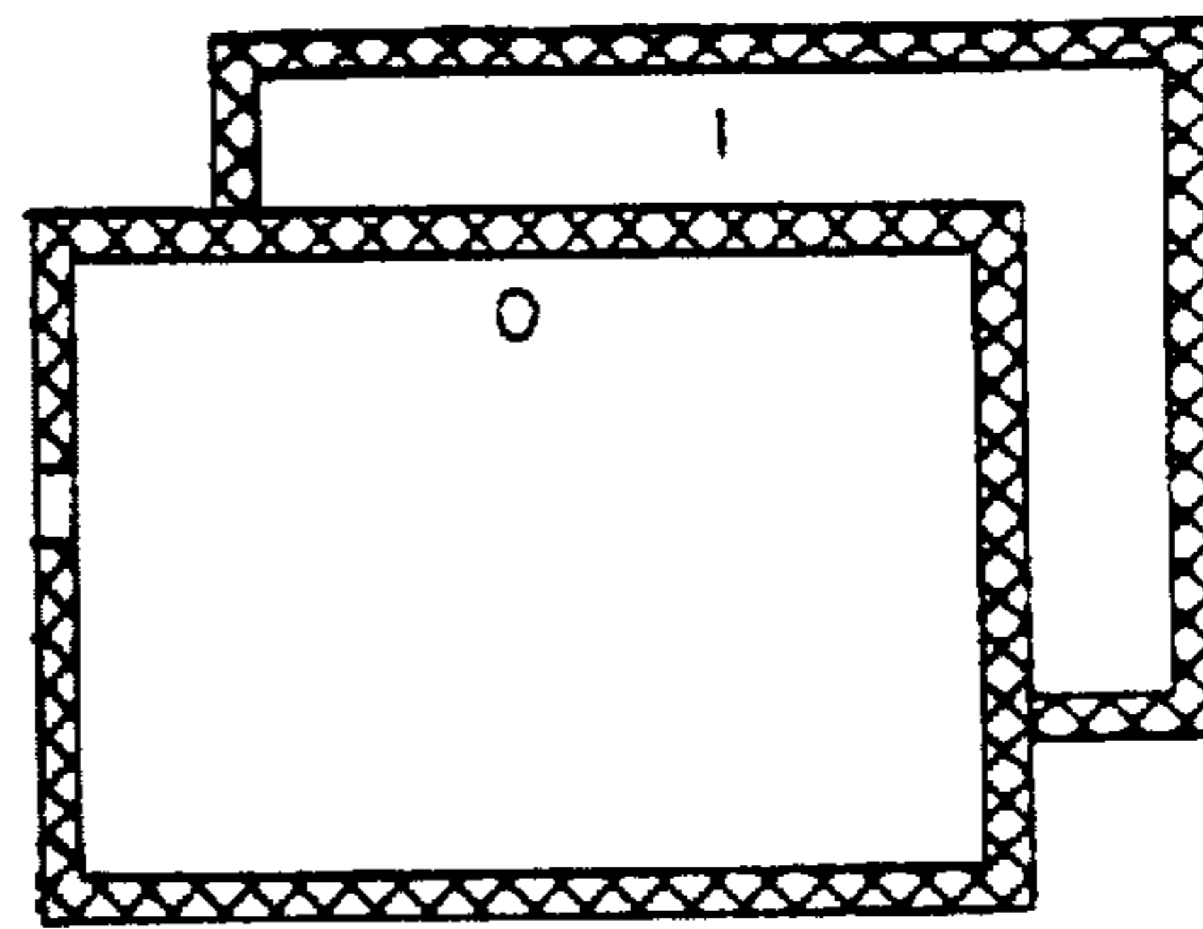
CONDITIONAL STRUCTURE
