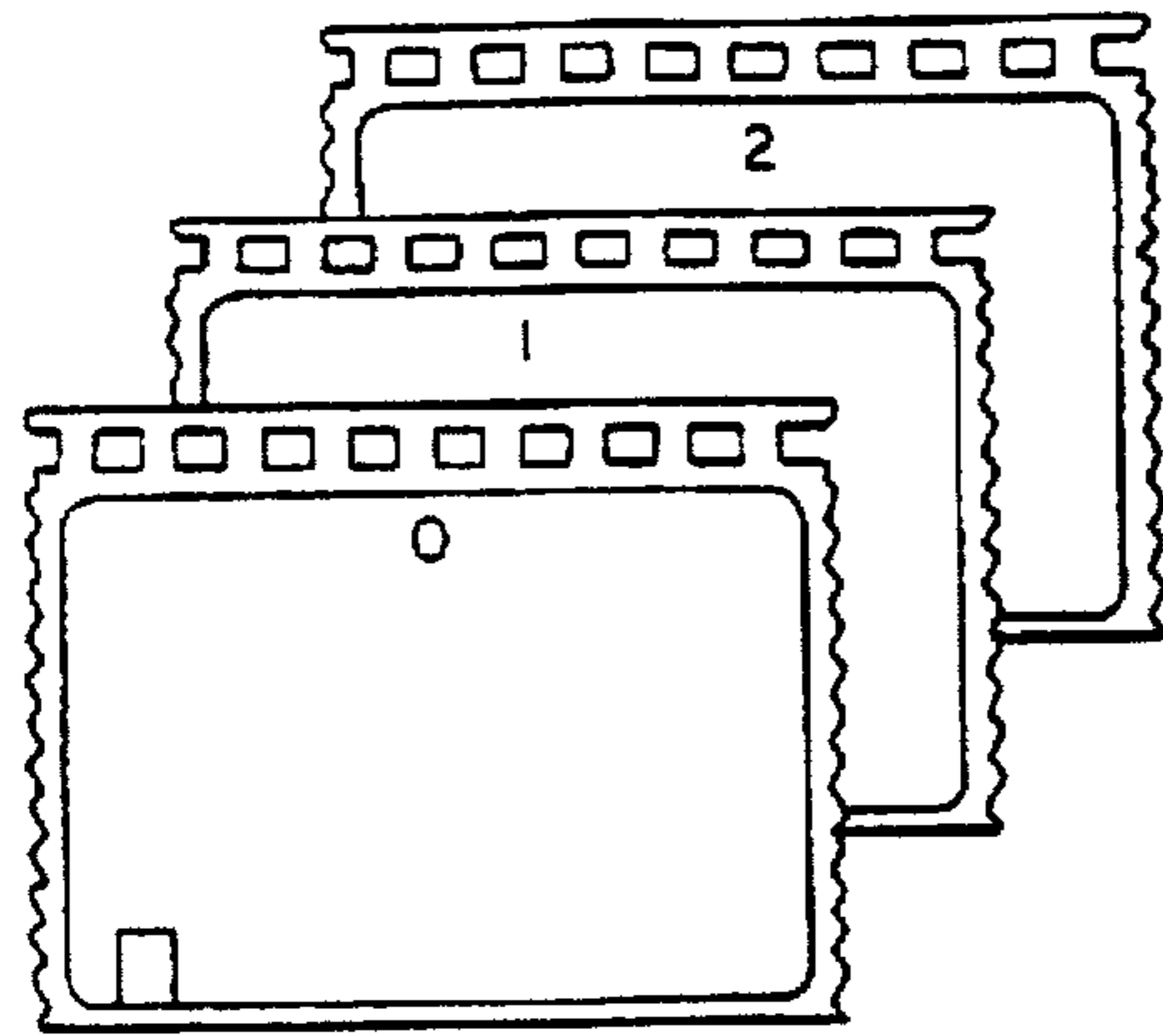
SEQUENCE STRUCTURE
