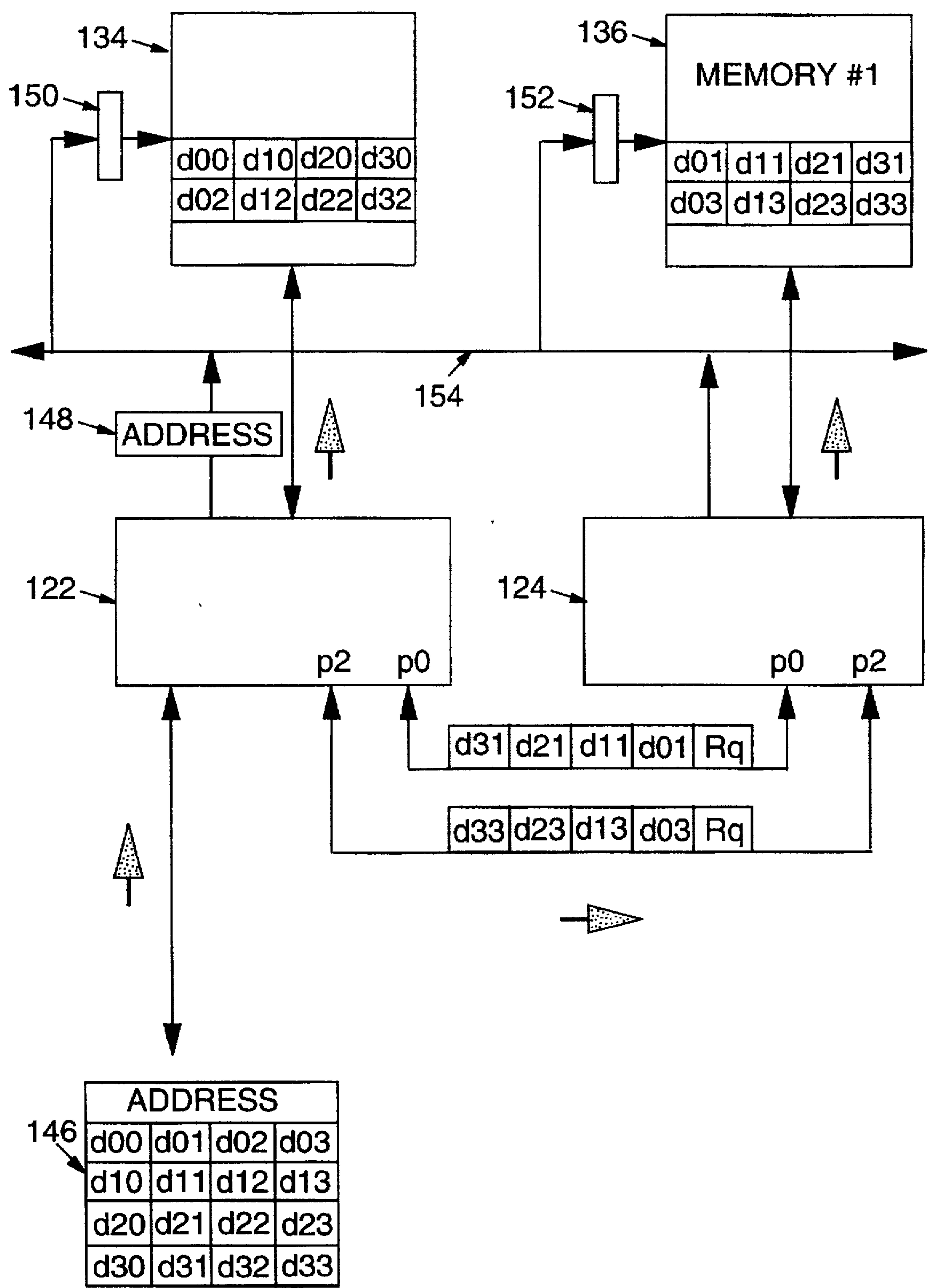
BURST WRITE OPERATION (two MIU's)
