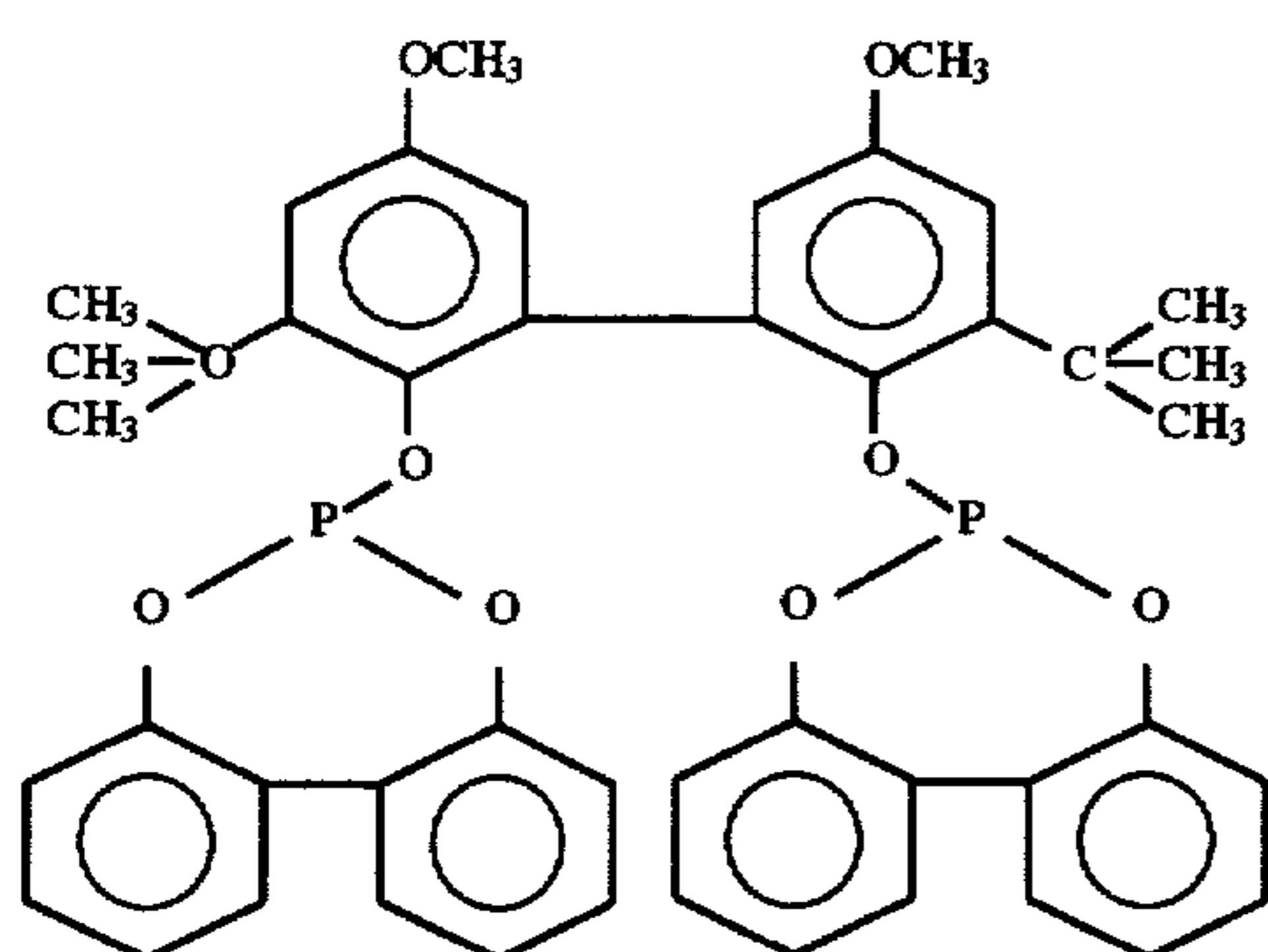
6,6'-[[3,3',5,5'-tetrakis(1,1-dimethylpropyl)-[1,1'-biphenyl]-2,2'-diyl]bis(oxy)]bis-dibenzo[d,f][1,3,2] dioxaphosphepin having the formula:
