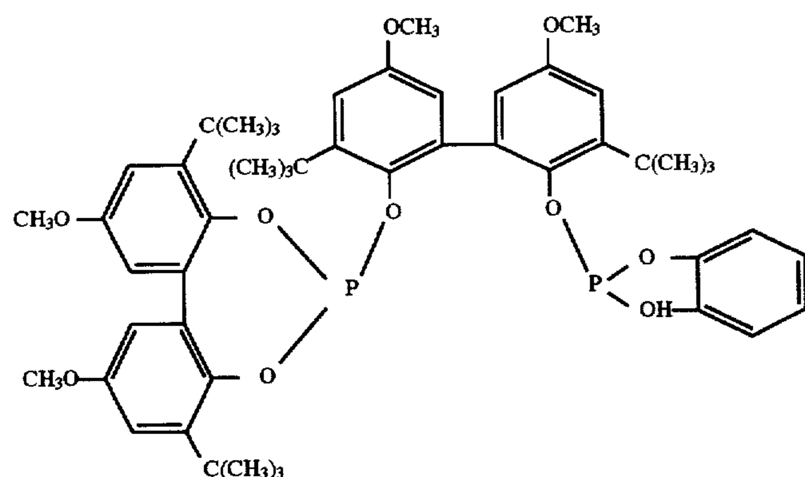
Ligand M
