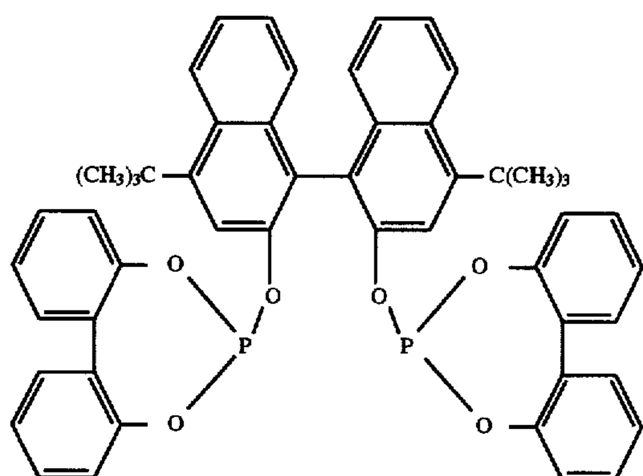
6,6'-[[3,3'-bis(1,1-dimethylethyl)-5,5'-dimethoxy-[1,1'-biphenyl]-2,2'-diyl]bis(oxy)]bis-dibenzo [d,f][1,3,2] dioxaphosphepin having the formula:
