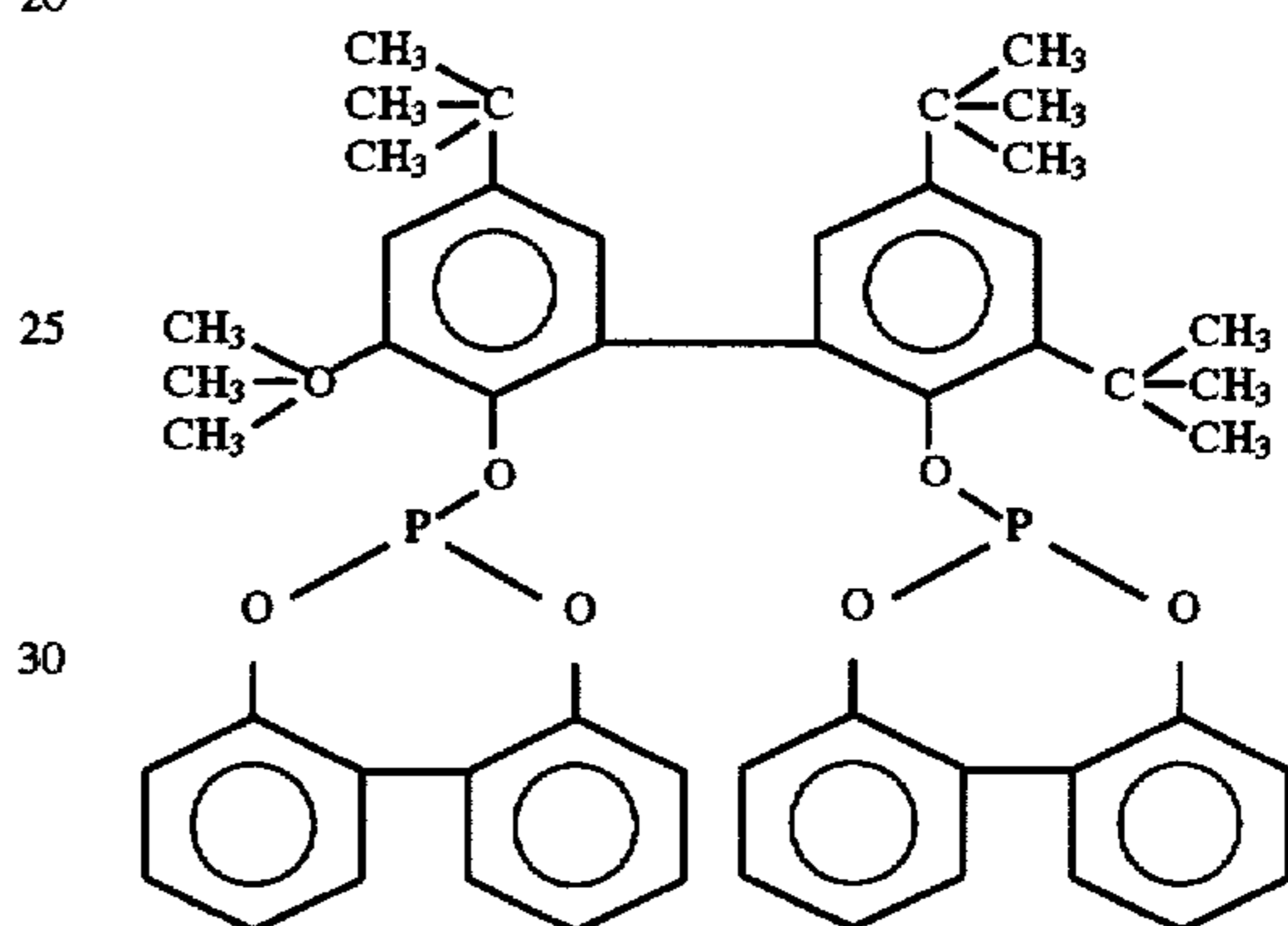
(2R,4R)-di[2,2'-(3,3',5,5'-tetrakis-tert-amyl-1,1'-biphenyl)]-2,4-pentylidiphosphite having the formula:
