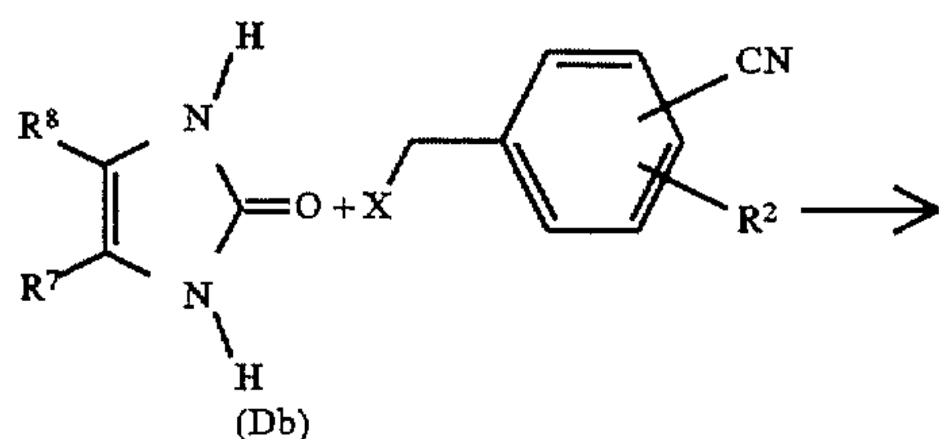
Reaction Scheme 3
