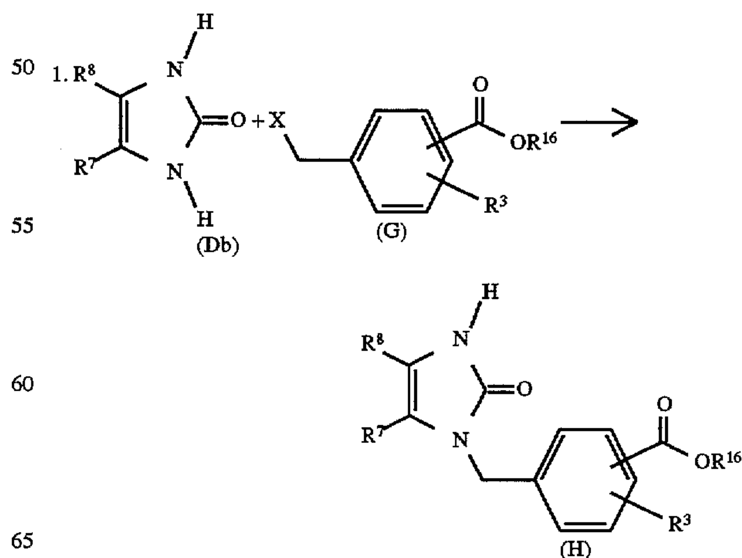
Reaction Scheme 4
