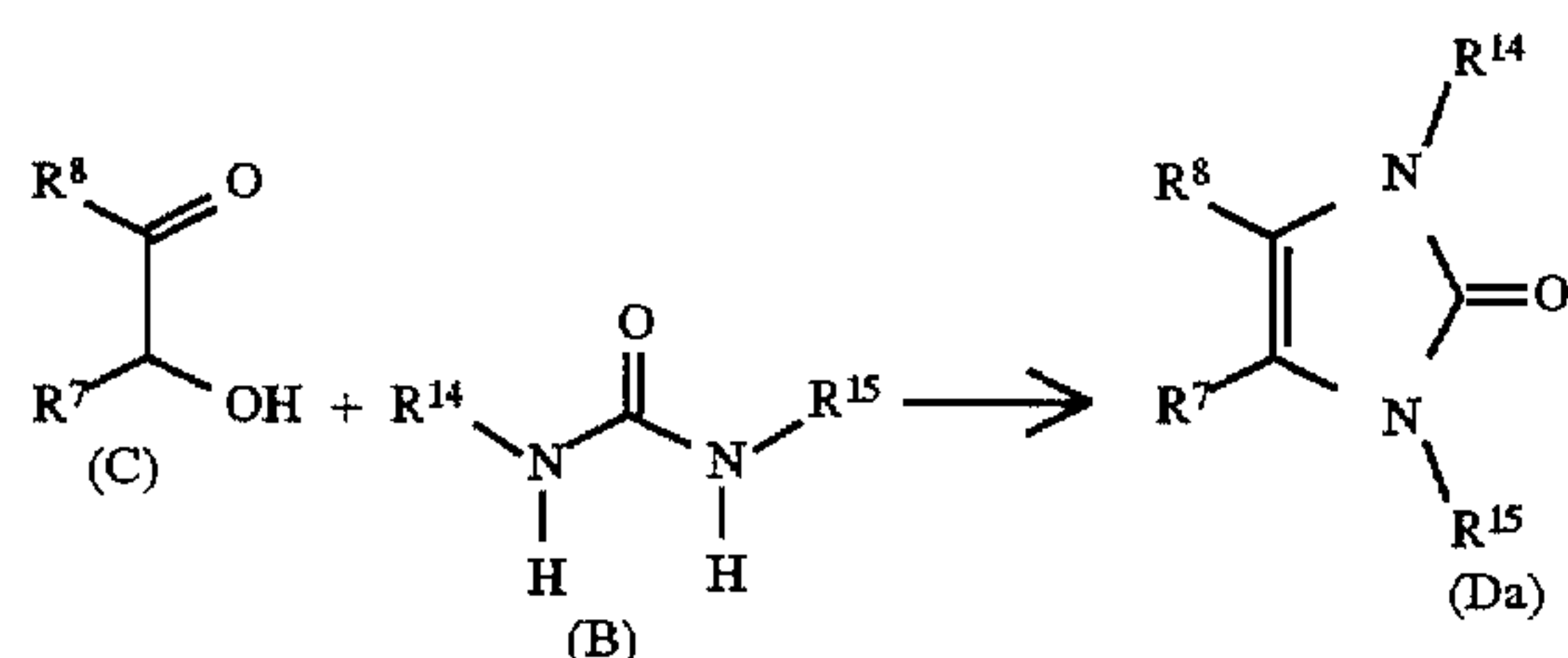
Reaction Scheme 2
