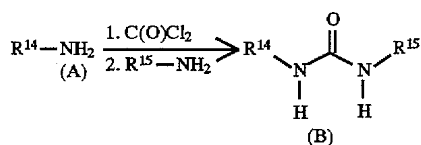
Reaction Scheme 1
