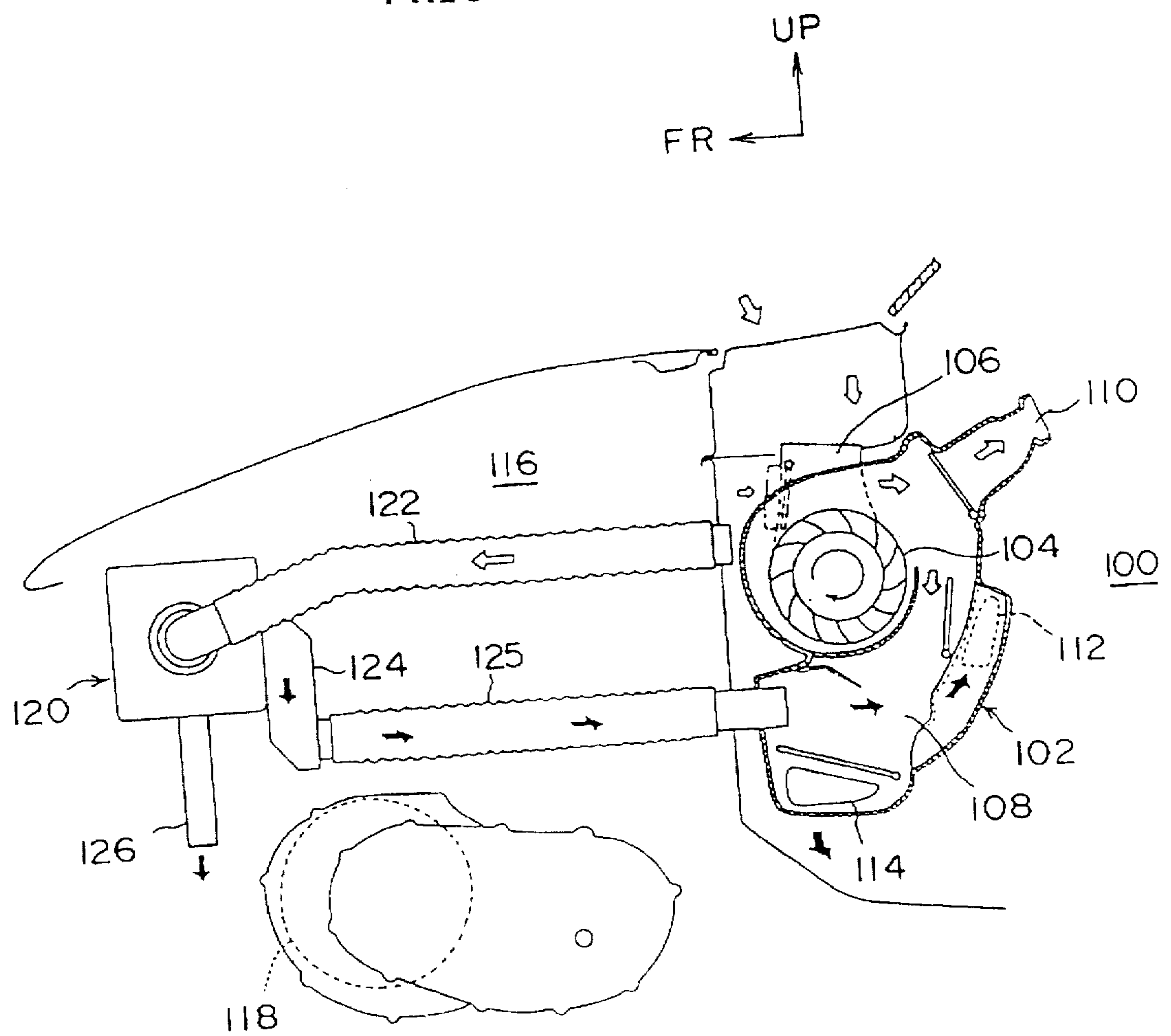
FIG. 7 PRIOR ART
