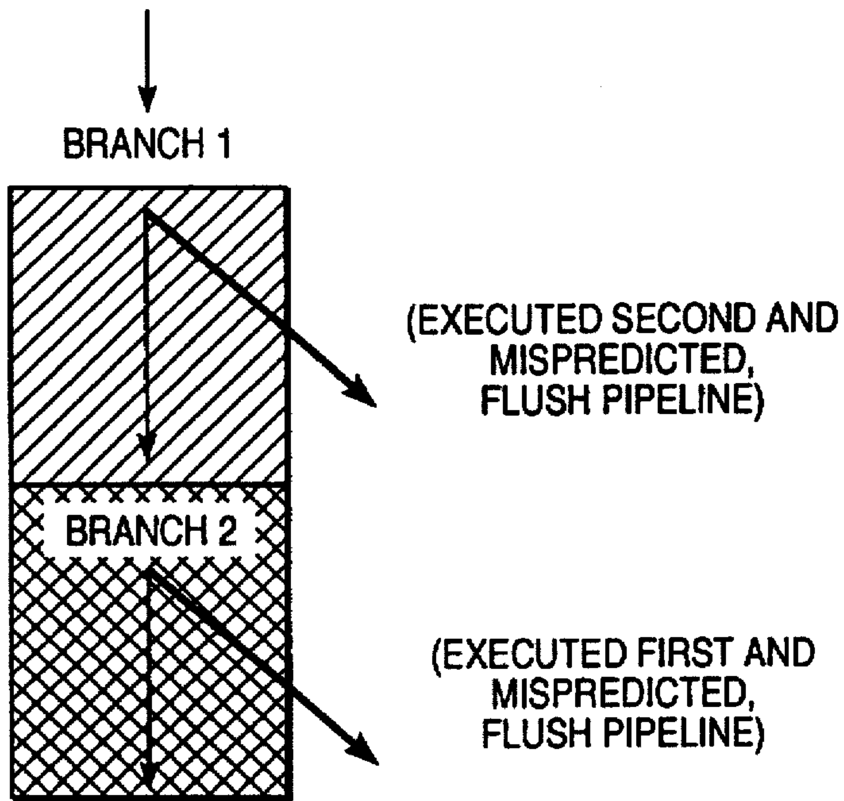
FIG 7C
