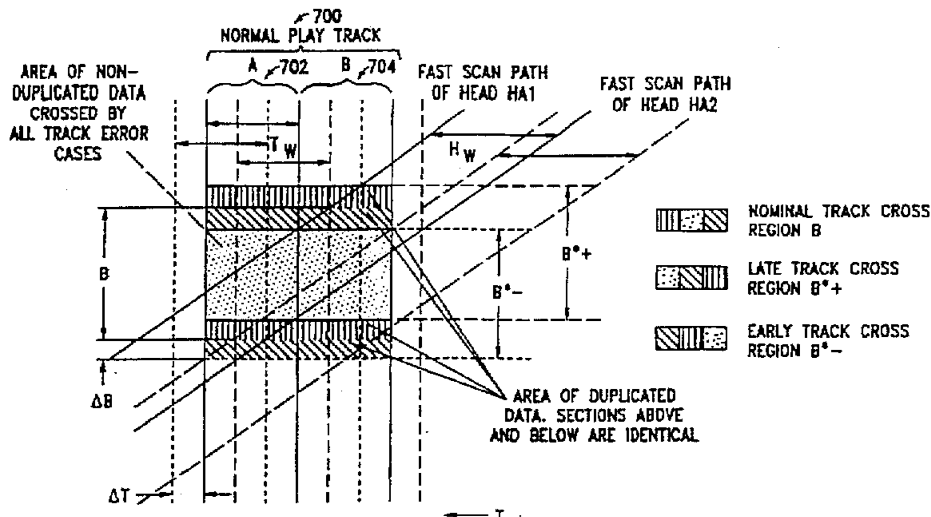
EFFECT OF TRACK ERRORS ON TRICK PLAY DATA RECOVERY
