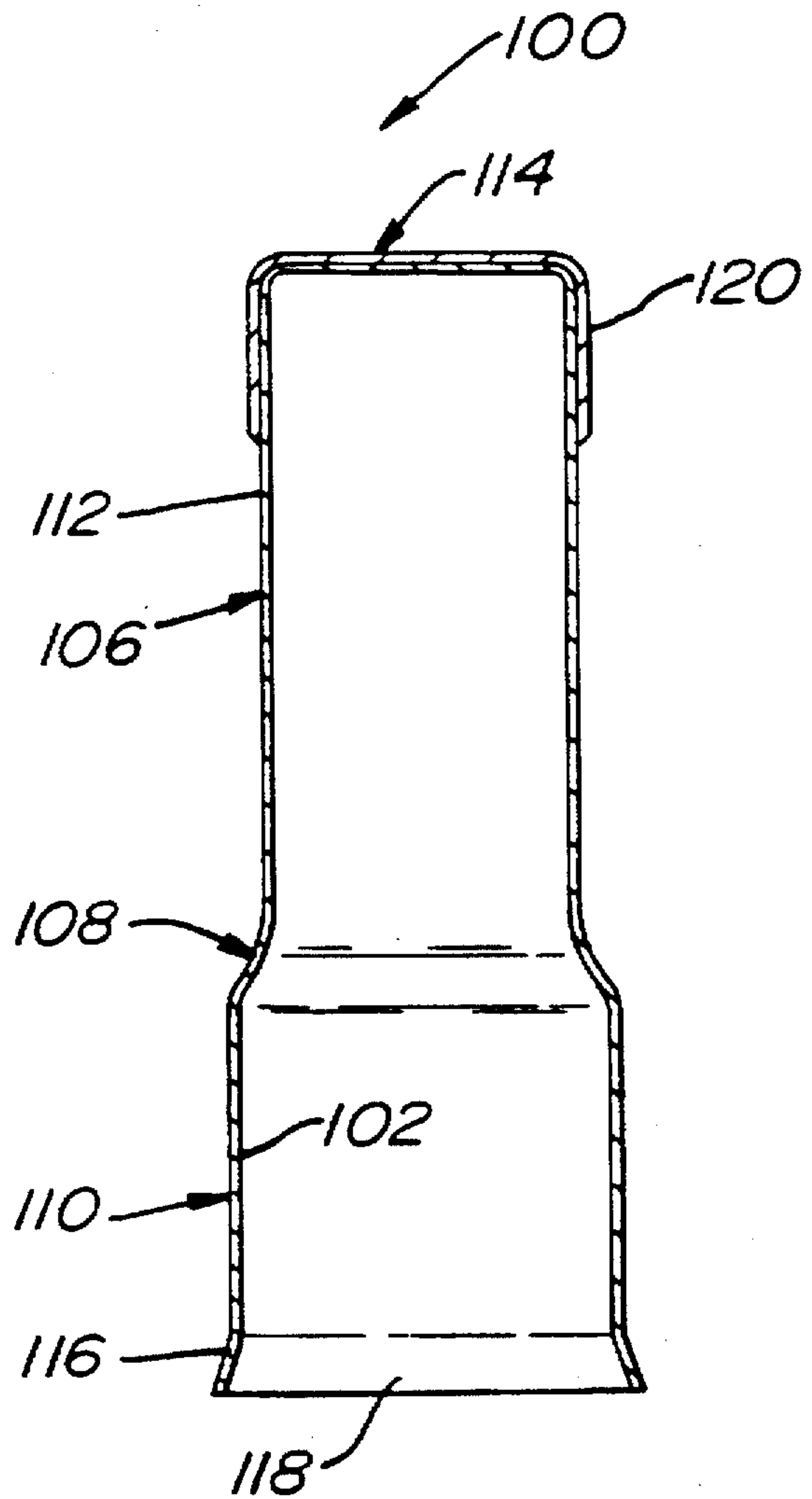
FIG. 2 PRIOR ART
