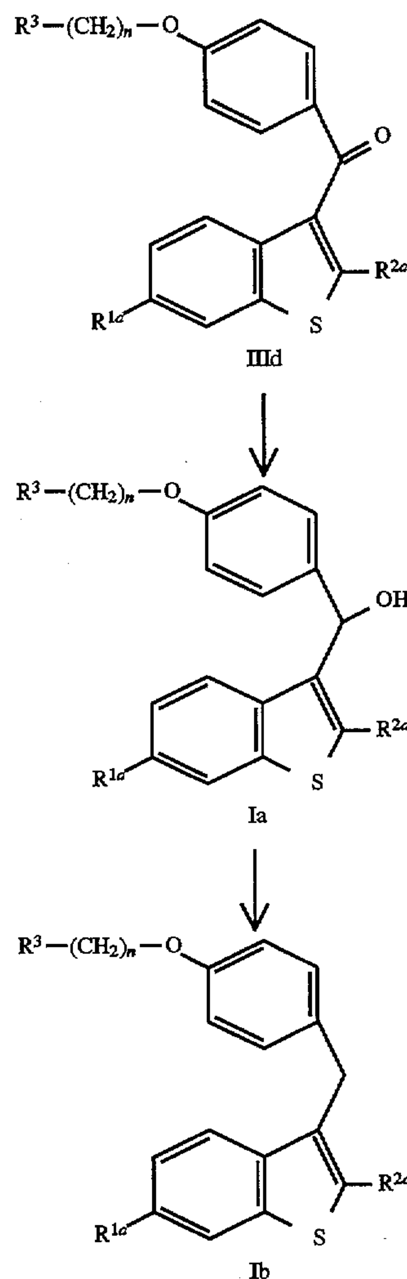
Scheme II
