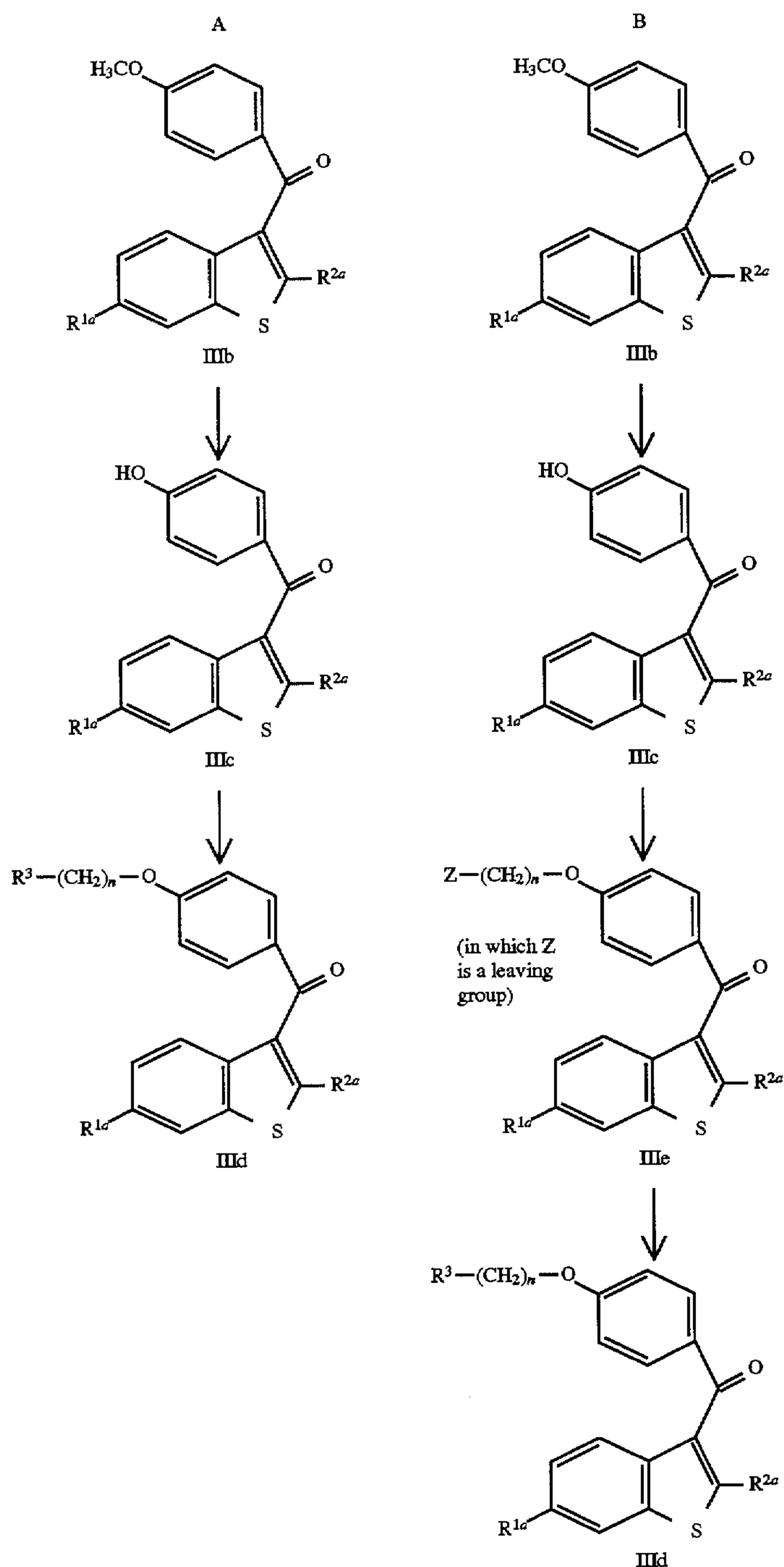
Scheme I
