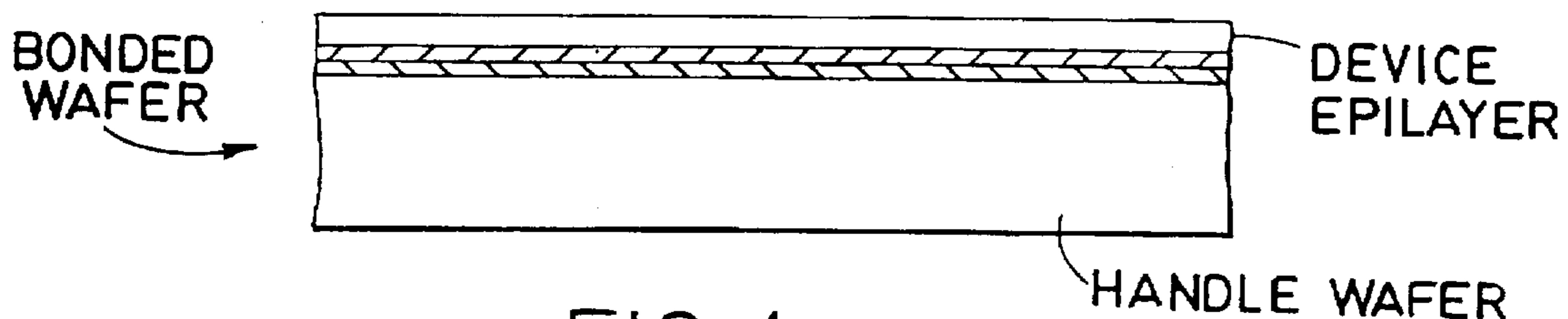
FIG. 1c (PRIOR ART)
