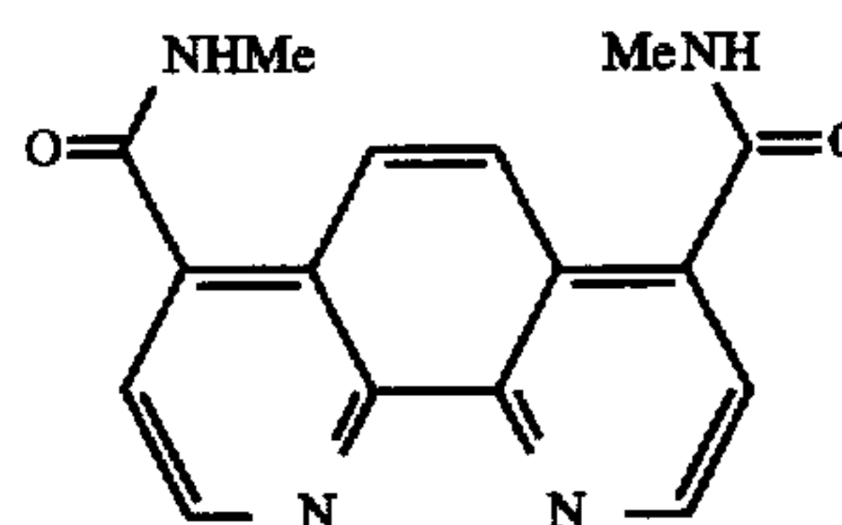
4,7-di-N-methylcarboxamido-1,10-phenanthroline
