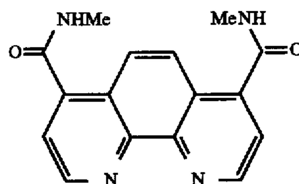
4,7-di-N-methylcarboxamido-1,10-phenanthroline
