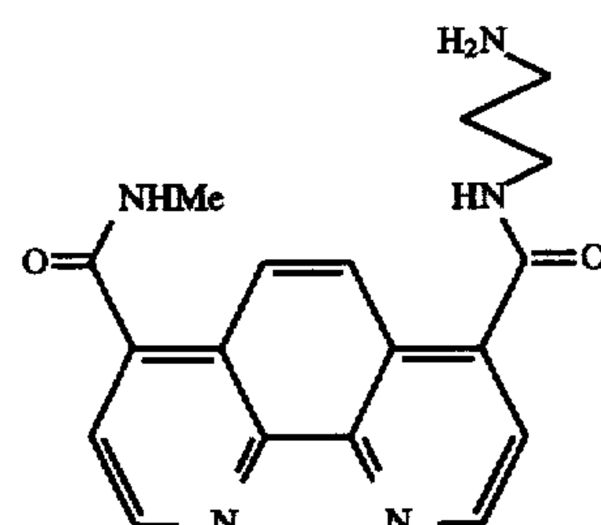
4-N-(3-aminopropyl)carboxamido-7-N-methylcarboxamido-1,10-phenanthroline
