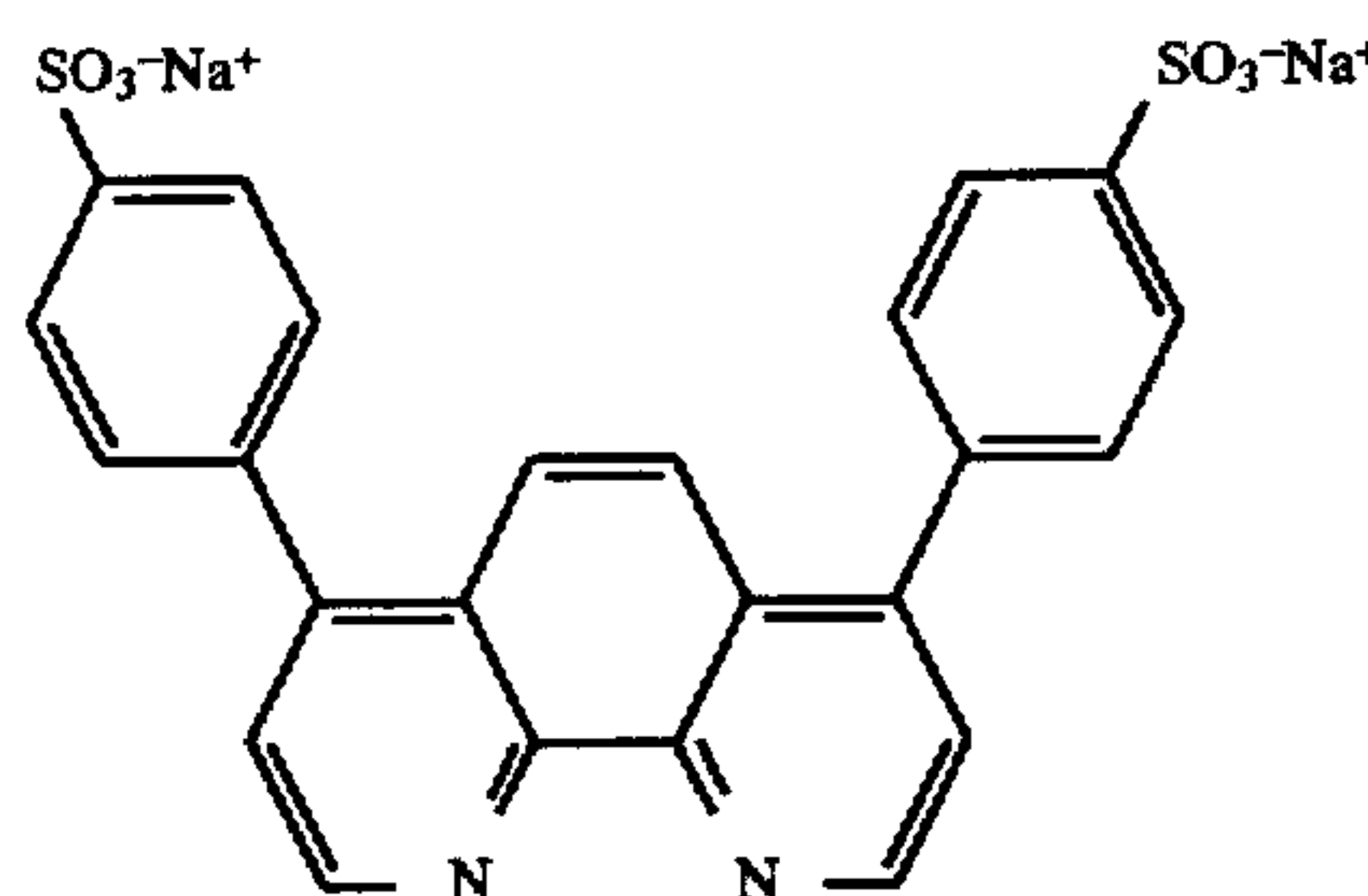
Bathophenanthroline
