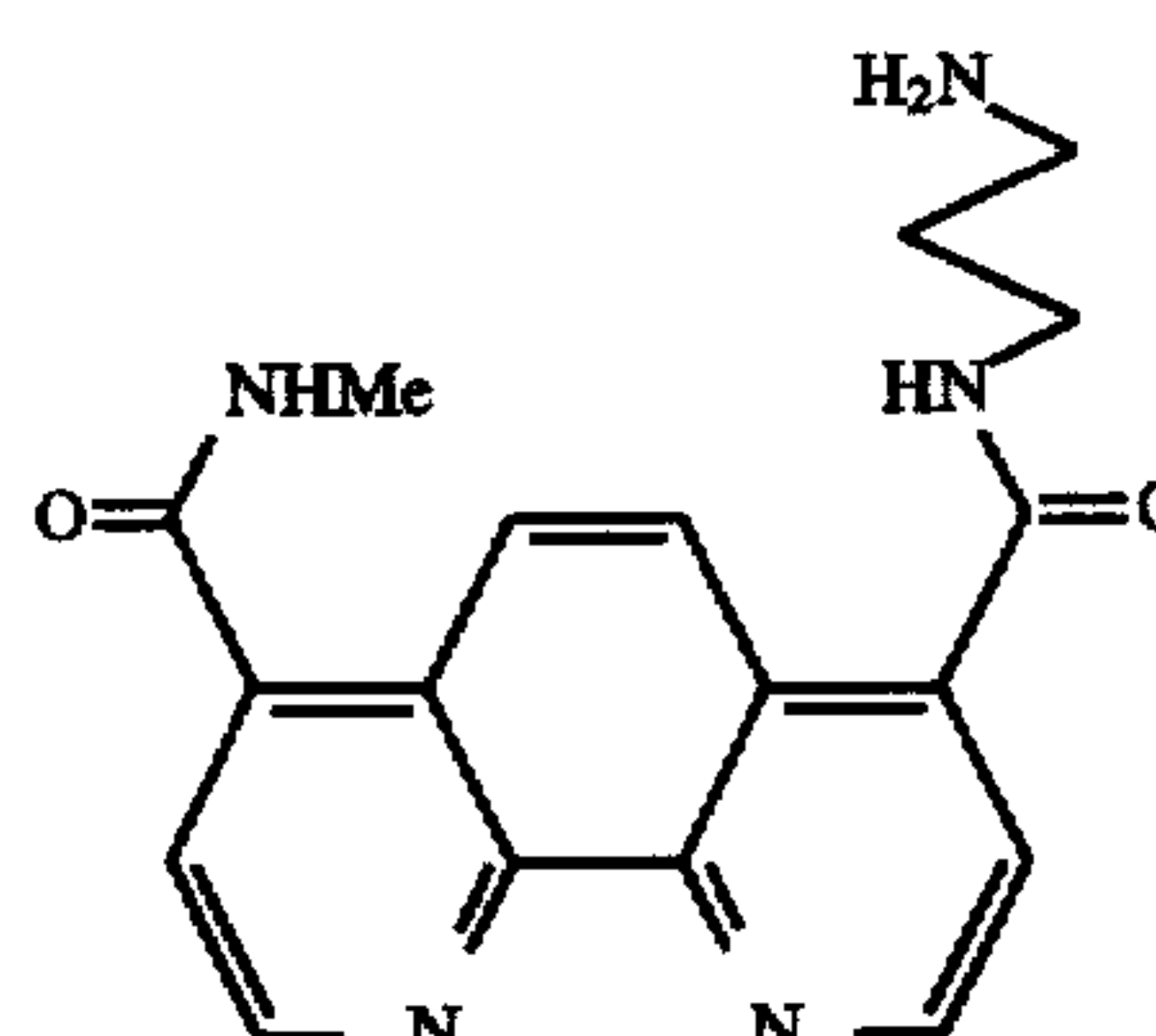
4-N-(3-aminopropyl)carboxamido-7-N-methylcarboxamido-1,10-phenanthroline
