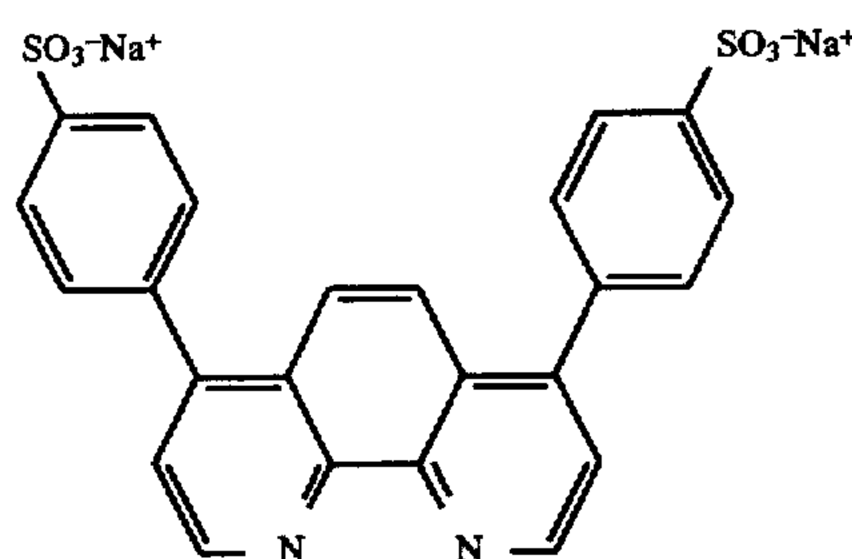
Bathophenanthroline
