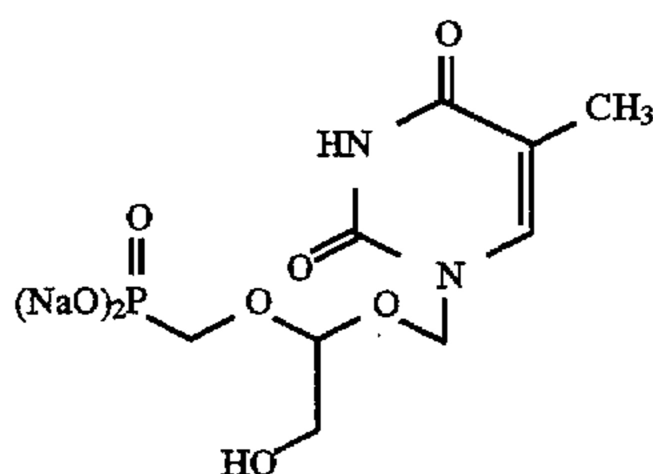
9-[(2-Hydroxy-1-phosphonomethoxyethoxymethyl)thymine disodium salt
