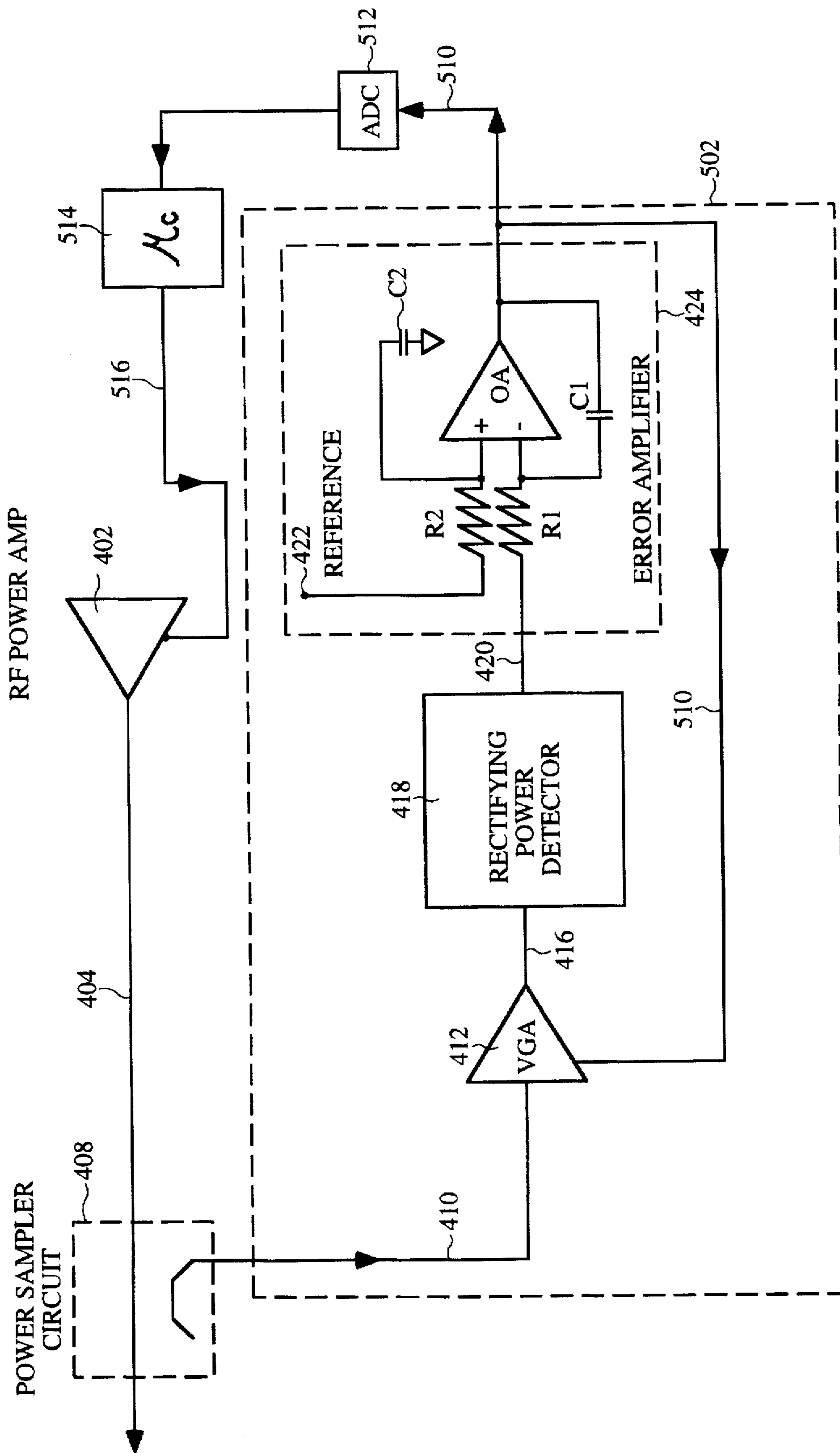
FIG. 6 POWER SENSOR
