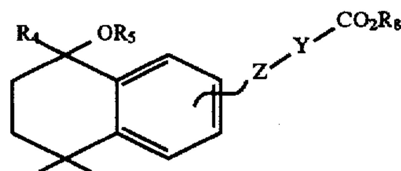
Formula 1A
