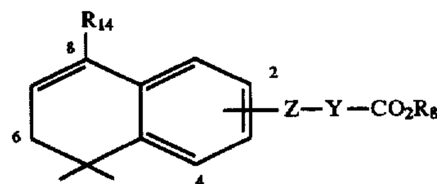
Formula 6A
