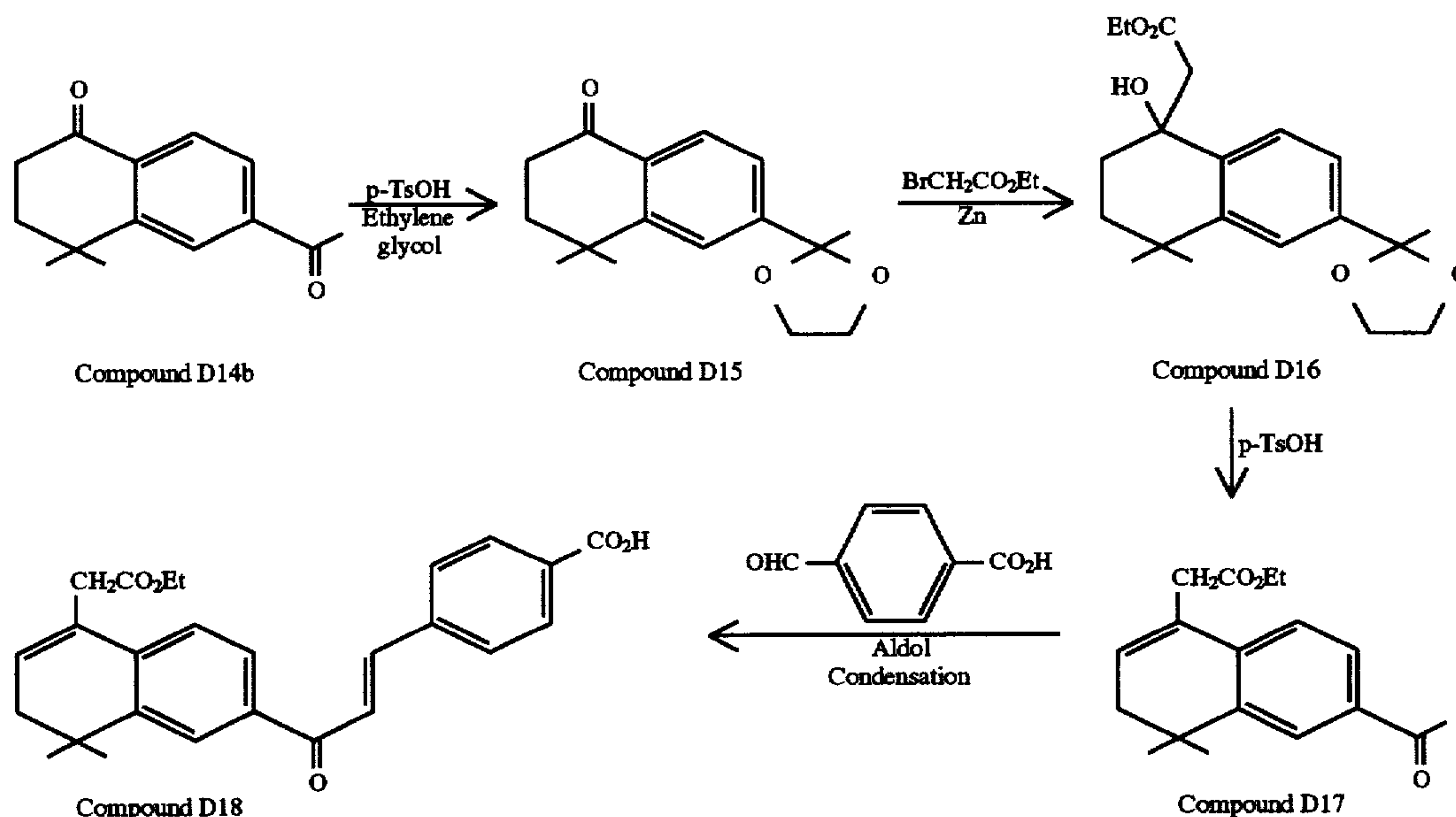
Reaction Scheme 11
