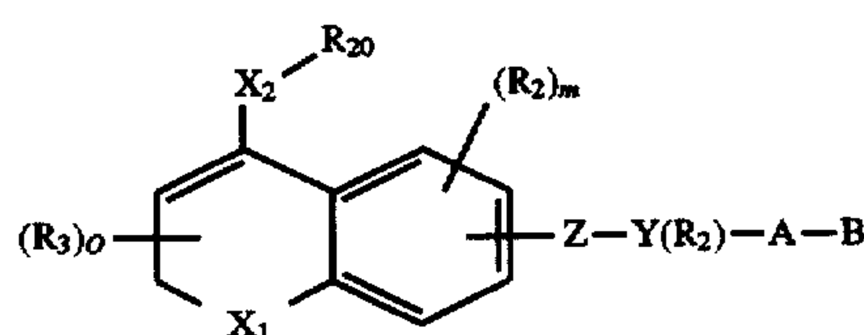
Formula 5
