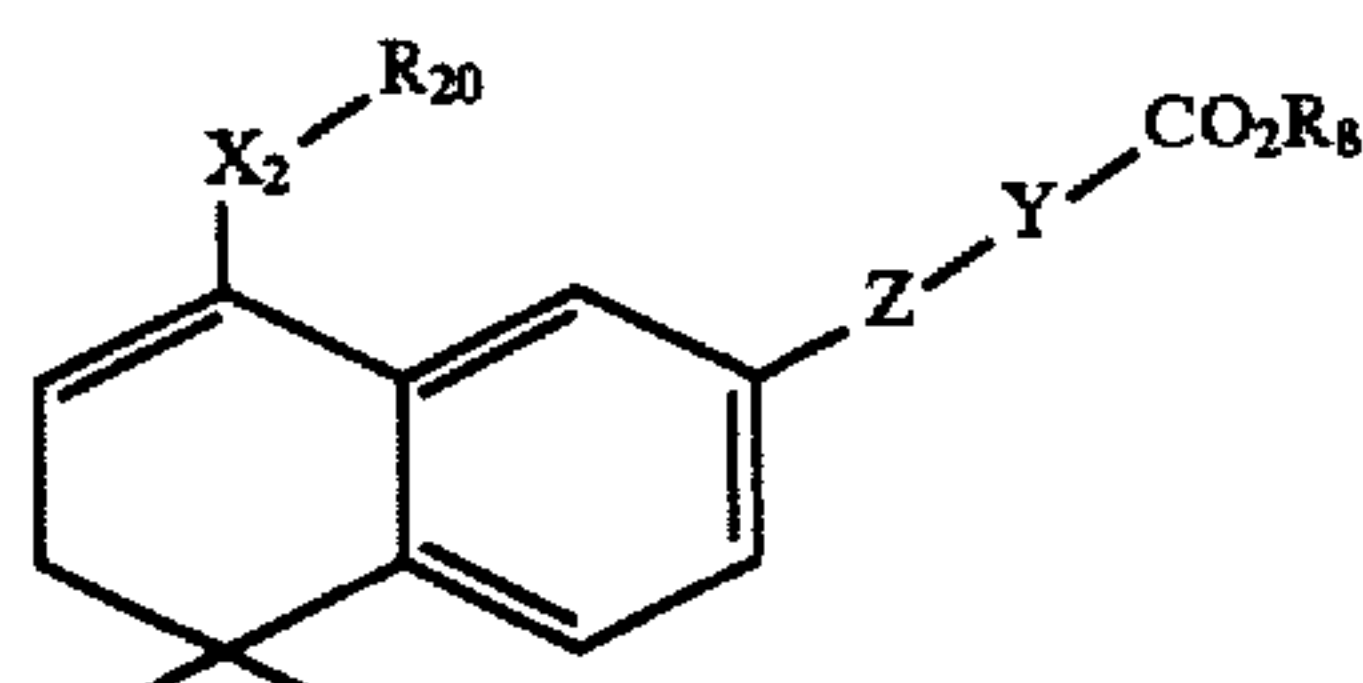
Formula 5A
