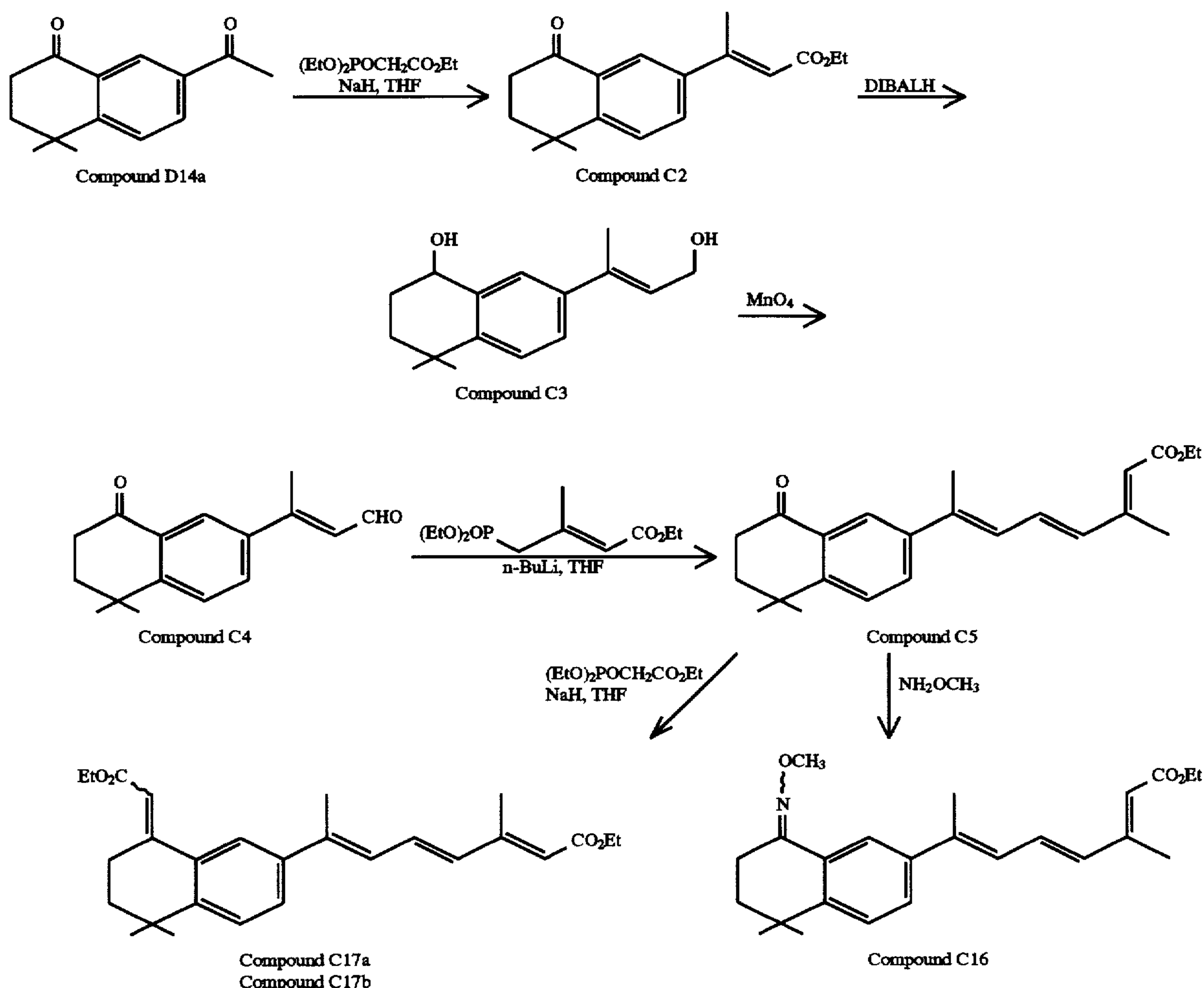
Reaction Scheme 7
