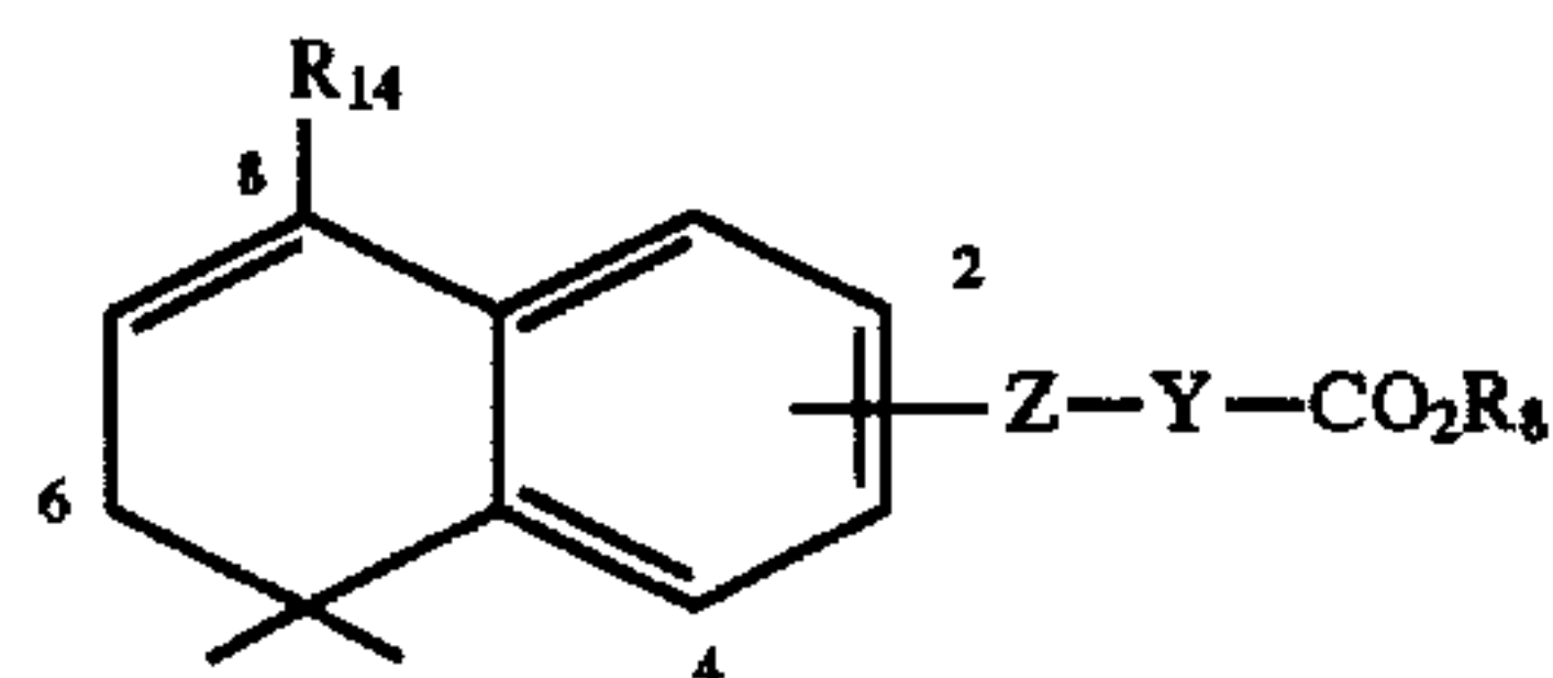
Formula 6A
