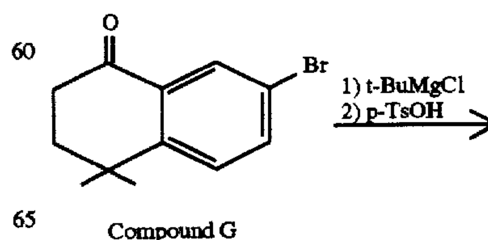
Reaction Scheme 9
