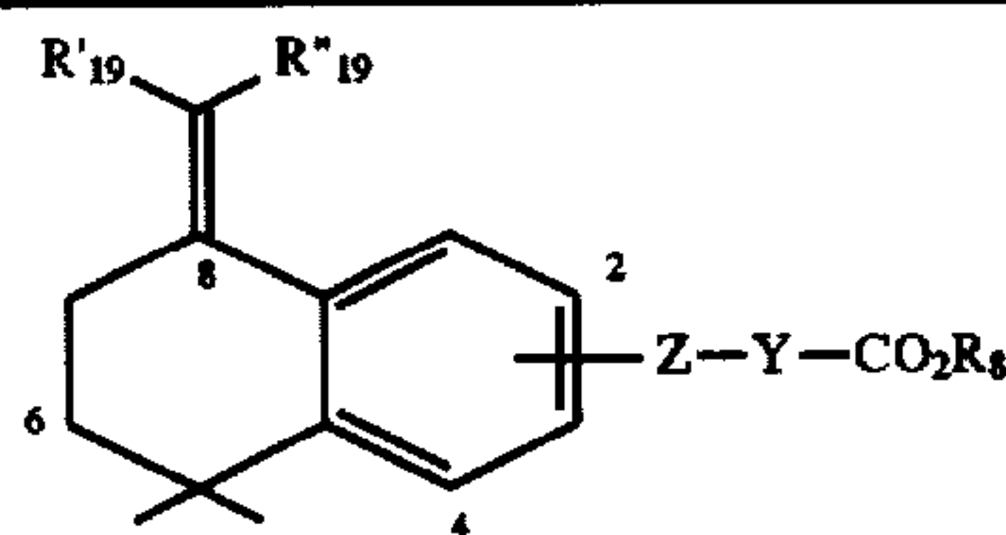
Formula 3A
