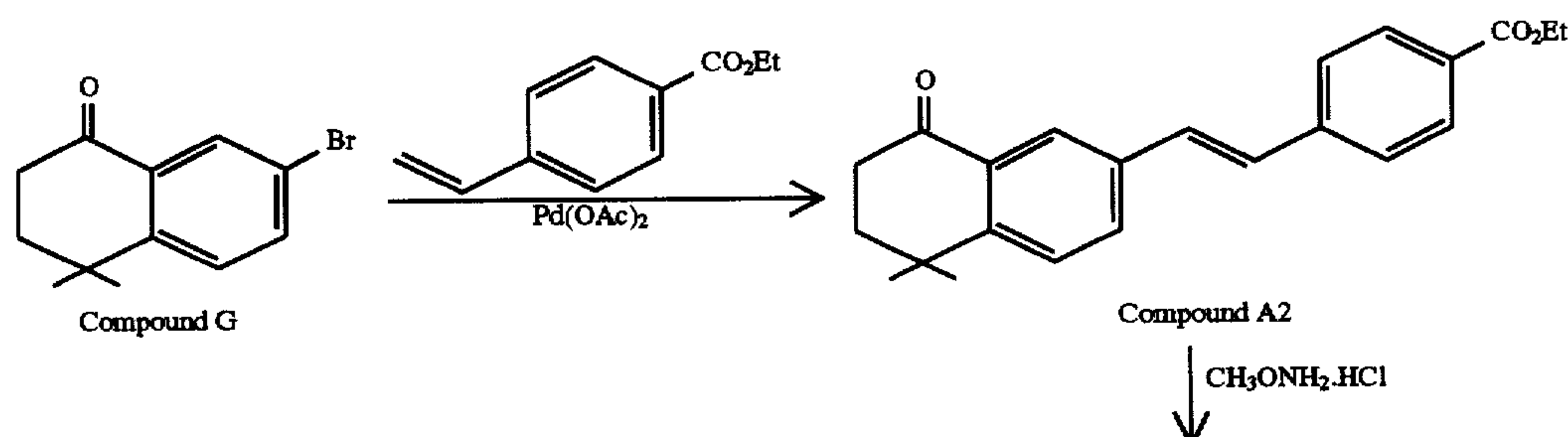
Reaction Scheme 2
