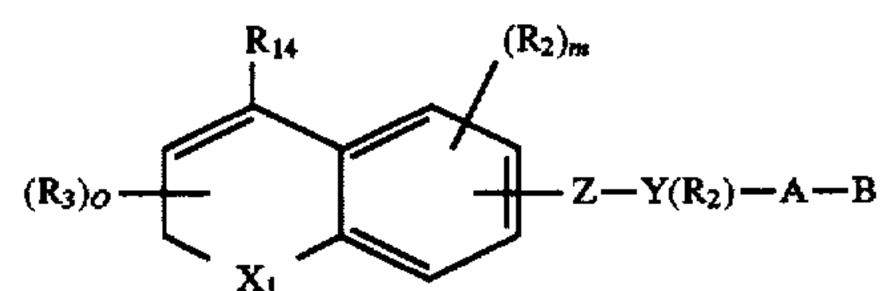
Formula 6
