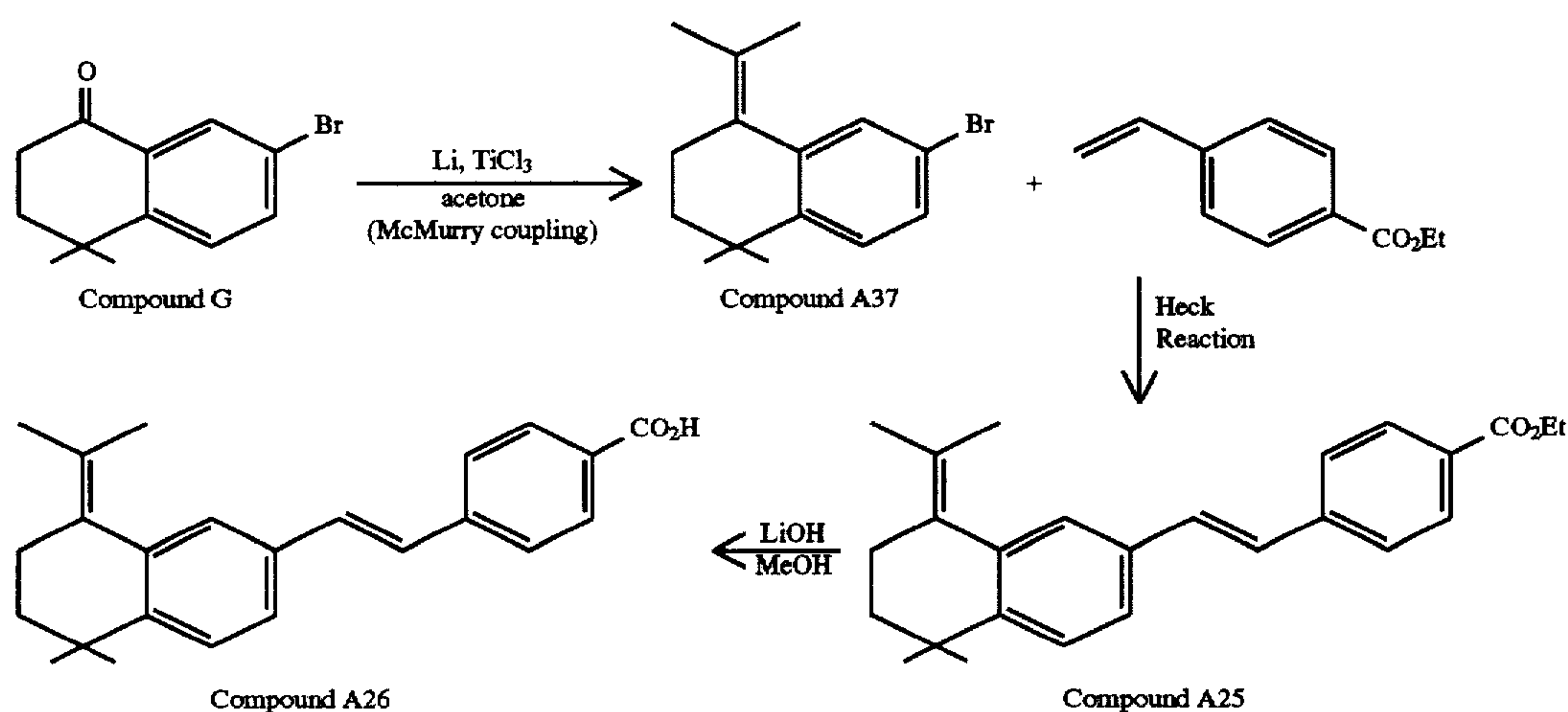
Reaction Scheme 5
