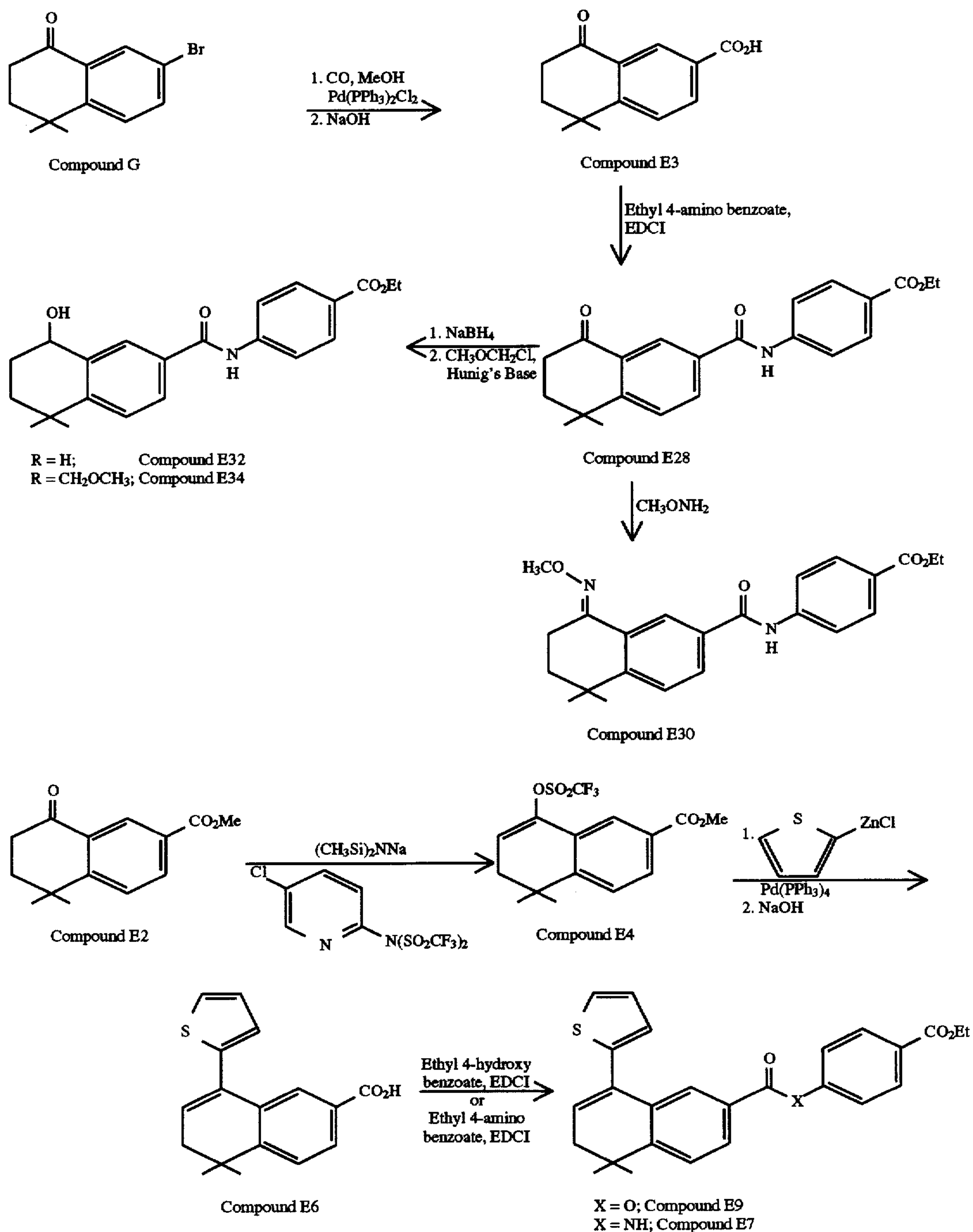
Reaction Scheme 12
