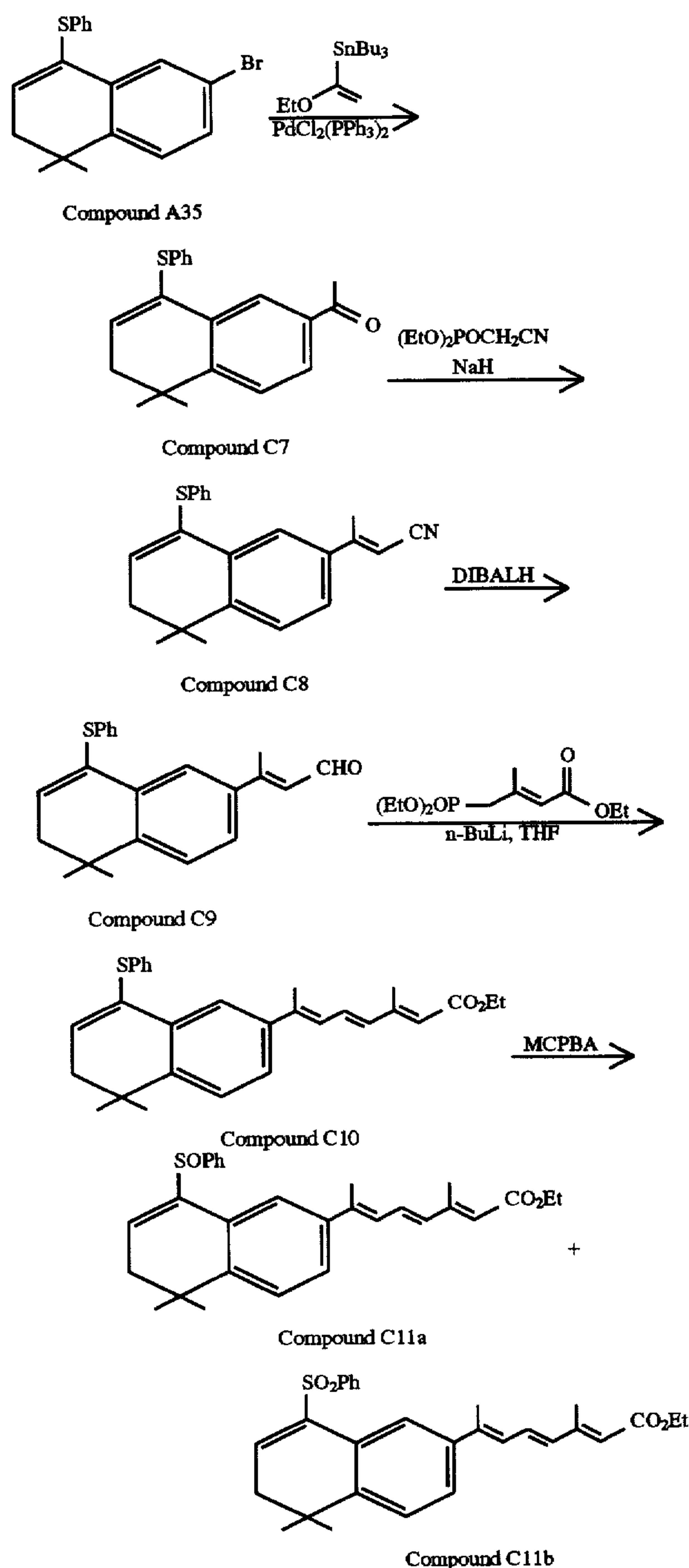
Reaction Scheme 8
