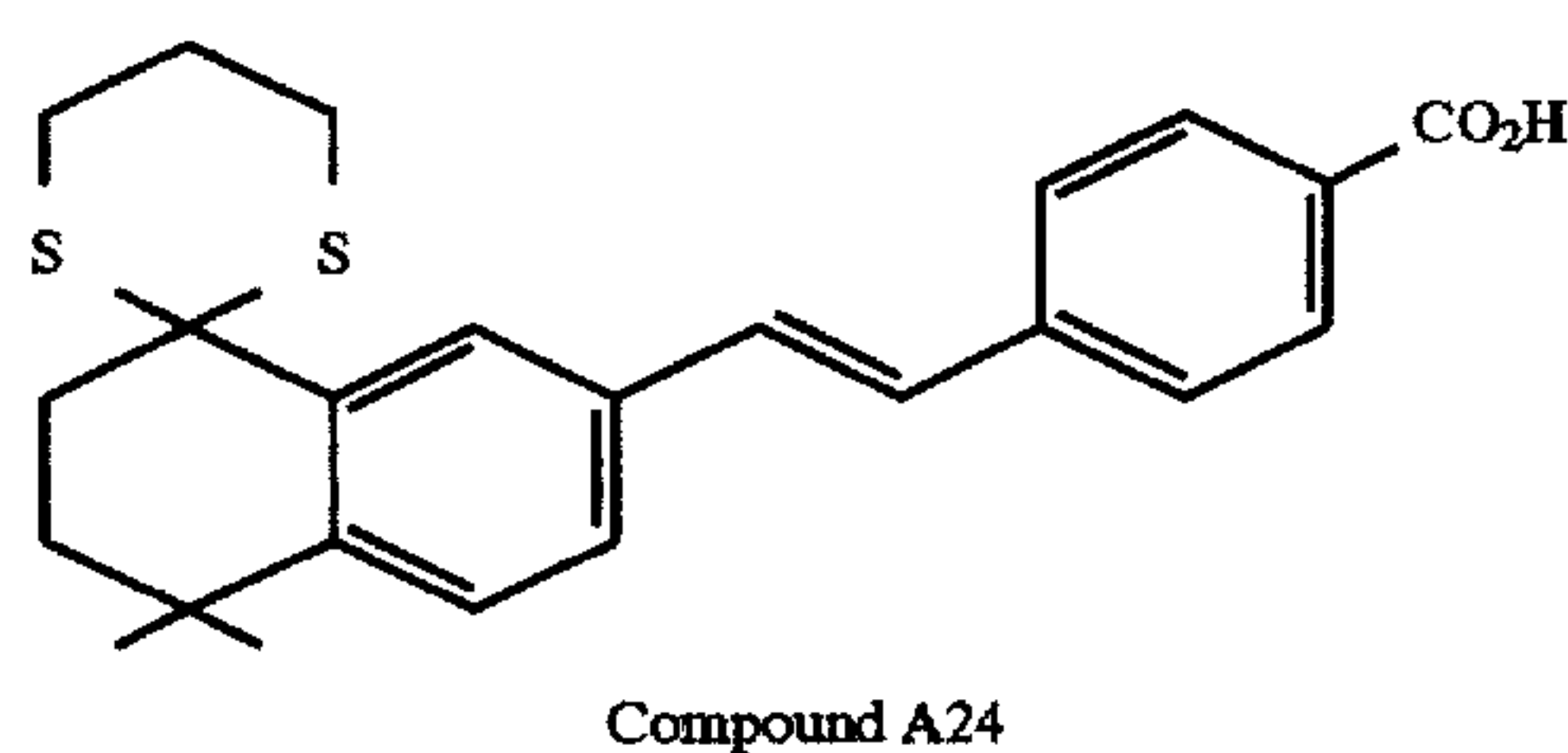
Reaction Scheme 4
