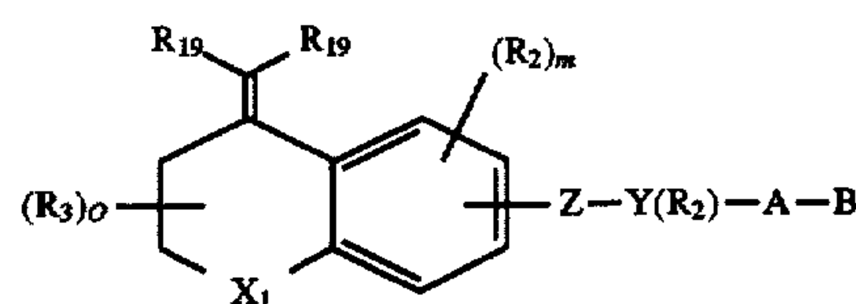
Formula 3
