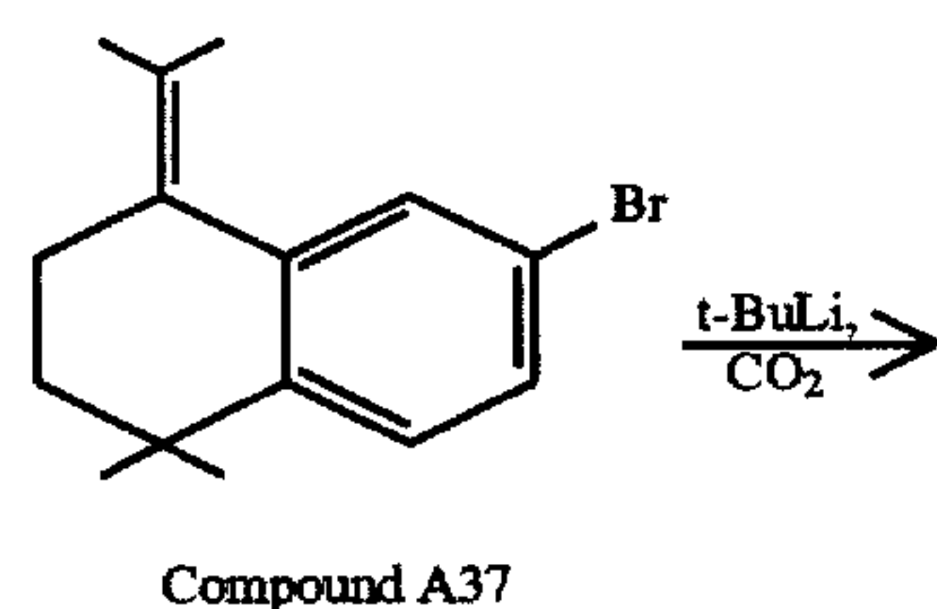
Reaction Scheme 13
