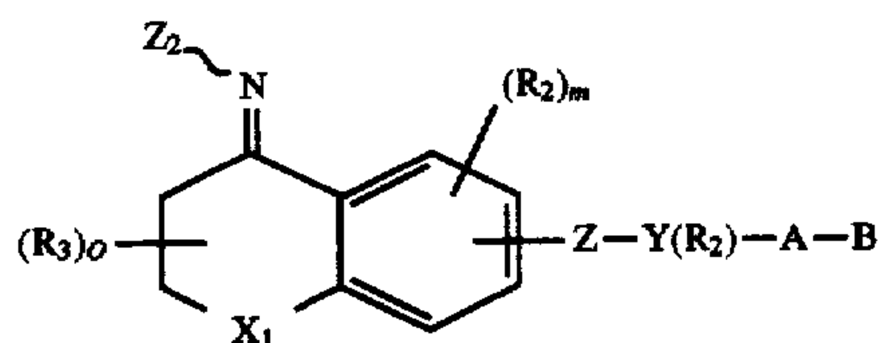
Formula 4
