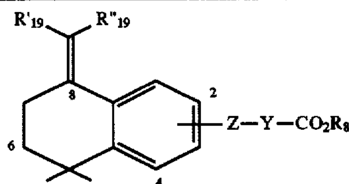
Formula 3A
