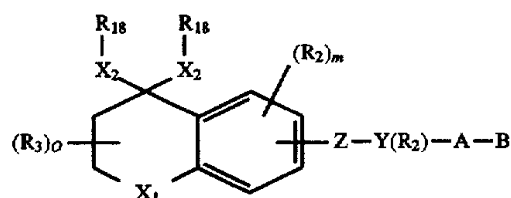
Formula 2
