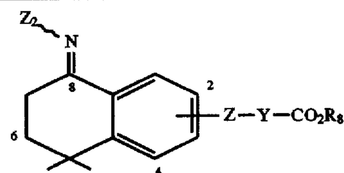
Formula 4A
