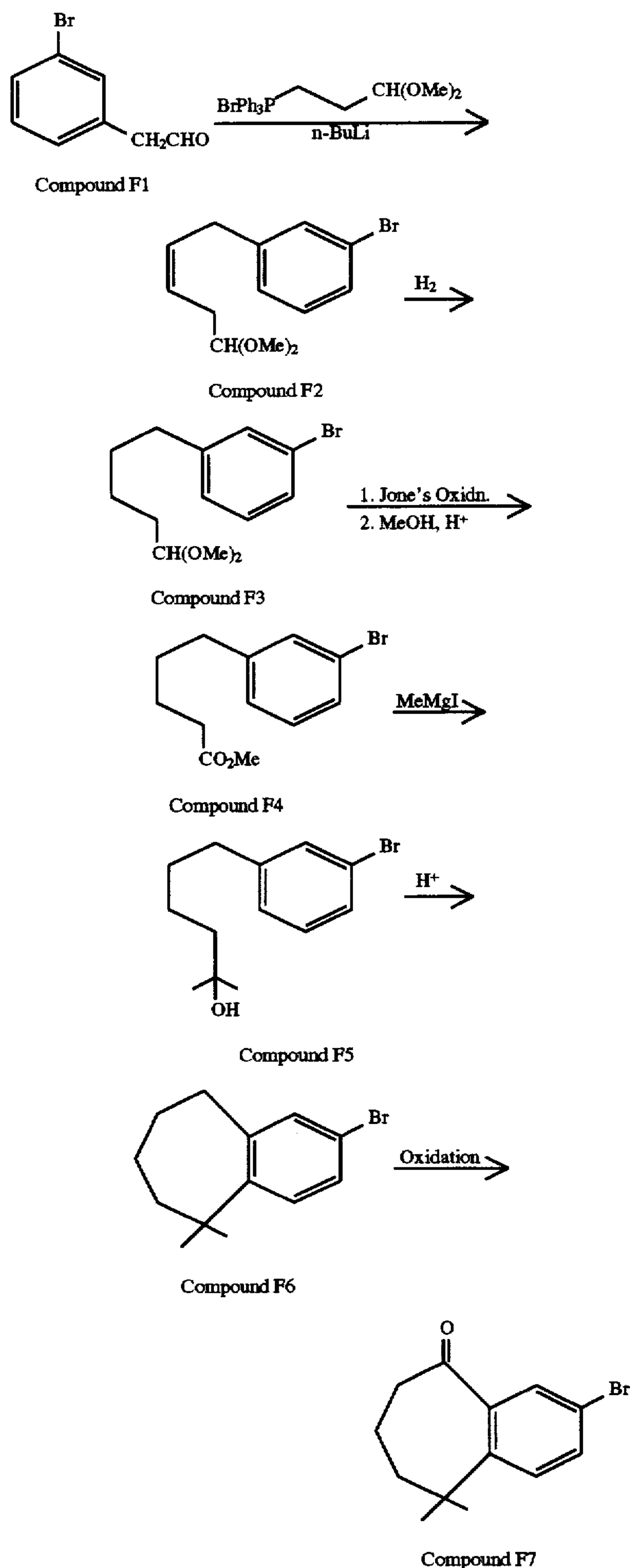
Reaction Scheme 15
