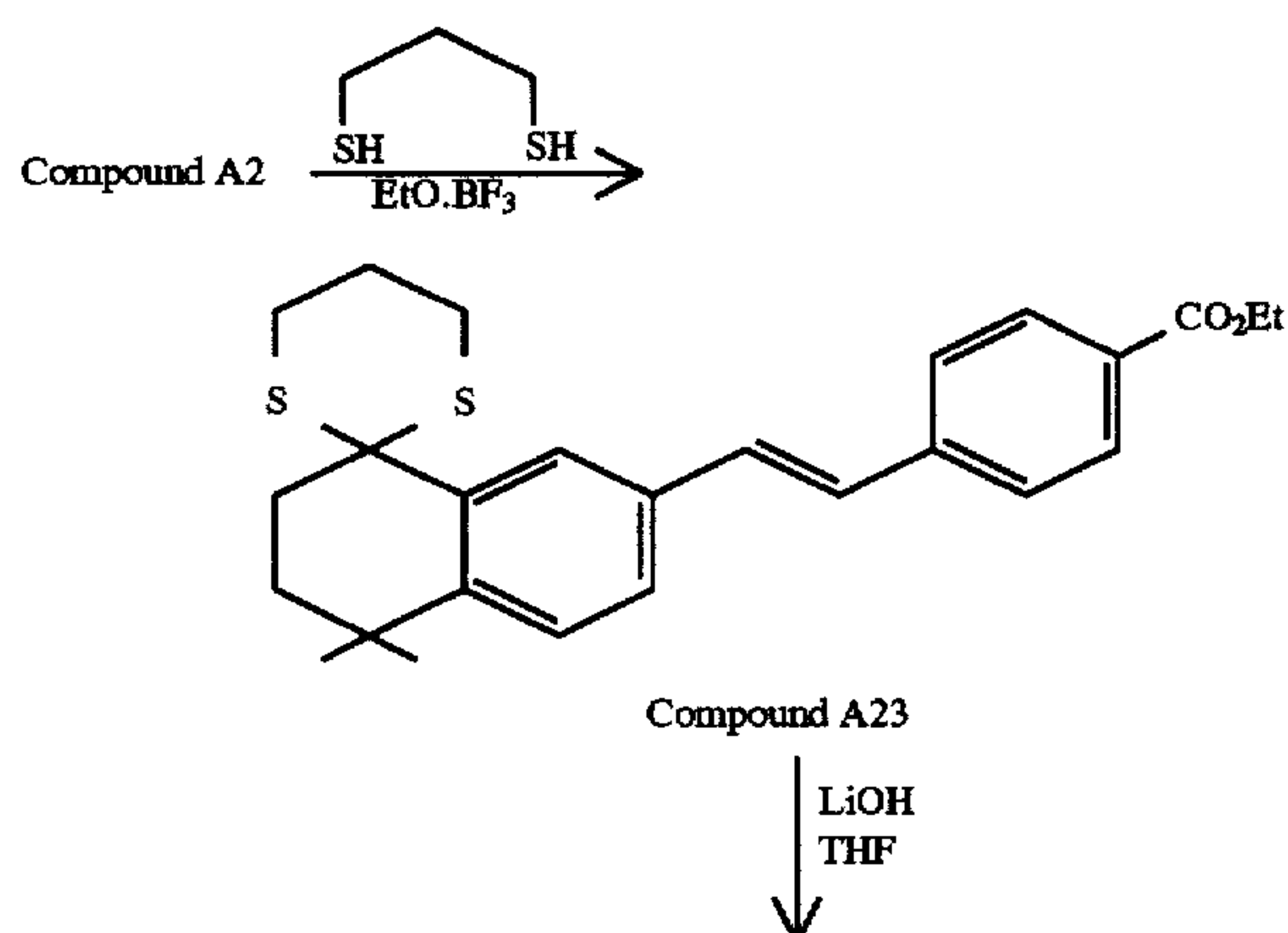
Reaction Scheme 4
