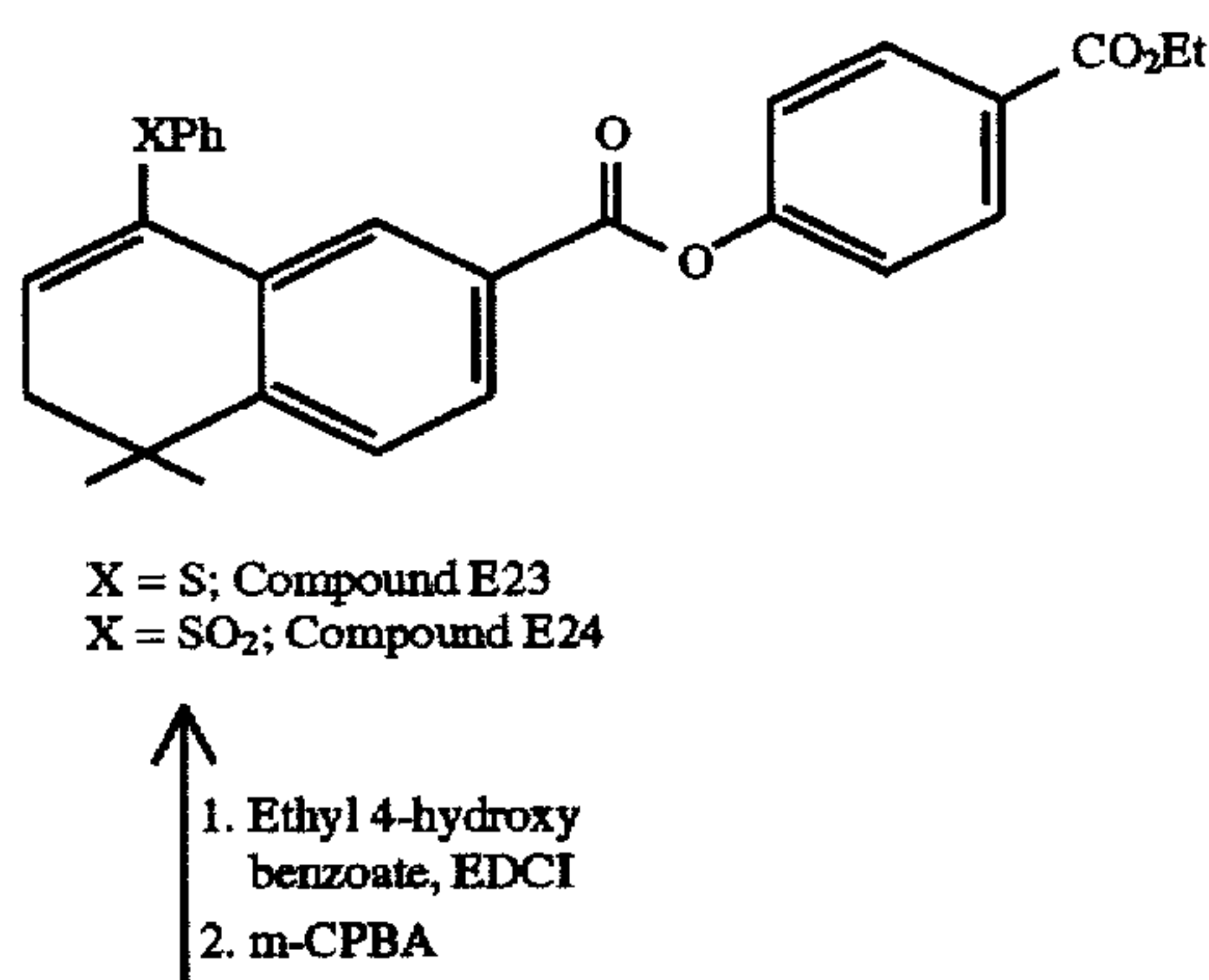
Reaction Scheme 14
