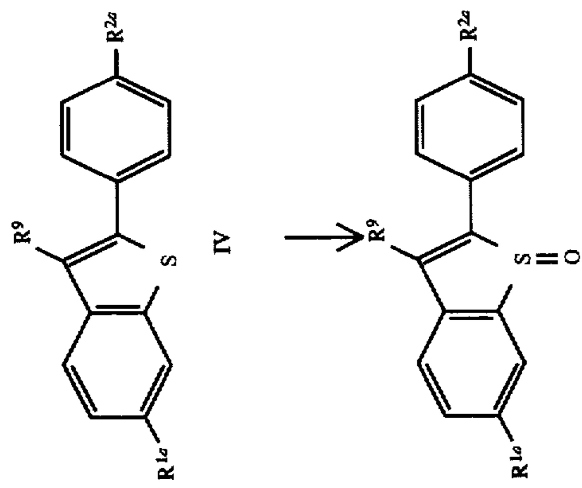
Scheme V
