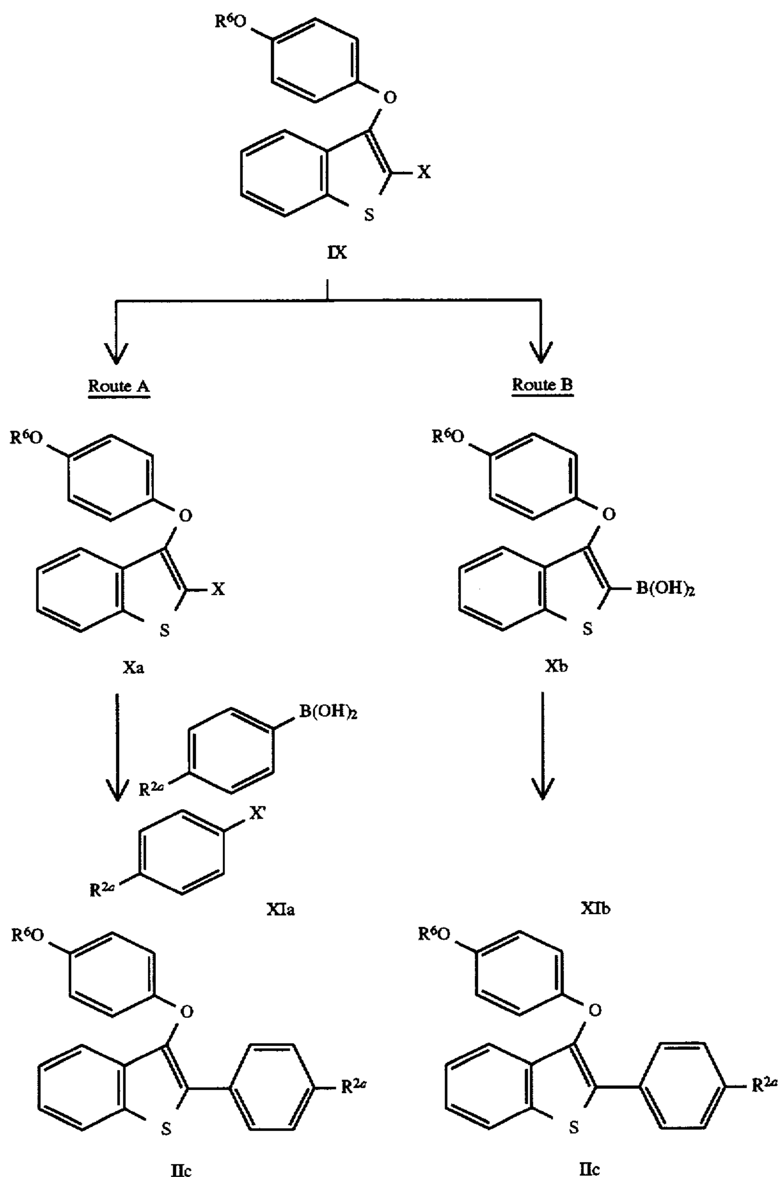
Scheme IV
