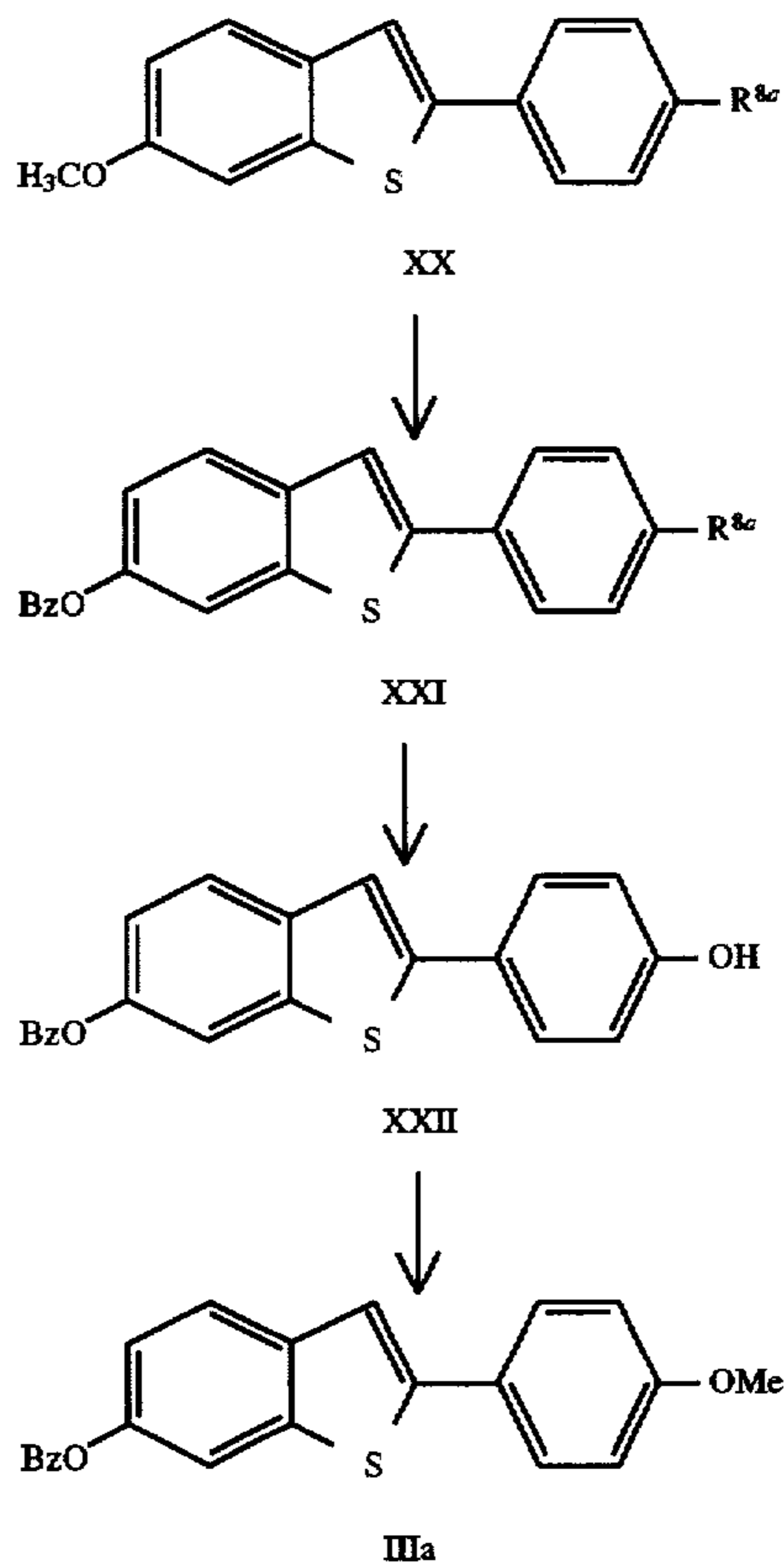
Scheme VII
