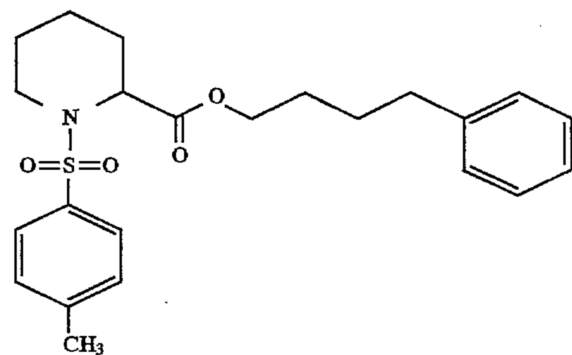
4-phenyl-1-butyl-N-(para-toluenesulfonyl)pipecolate
