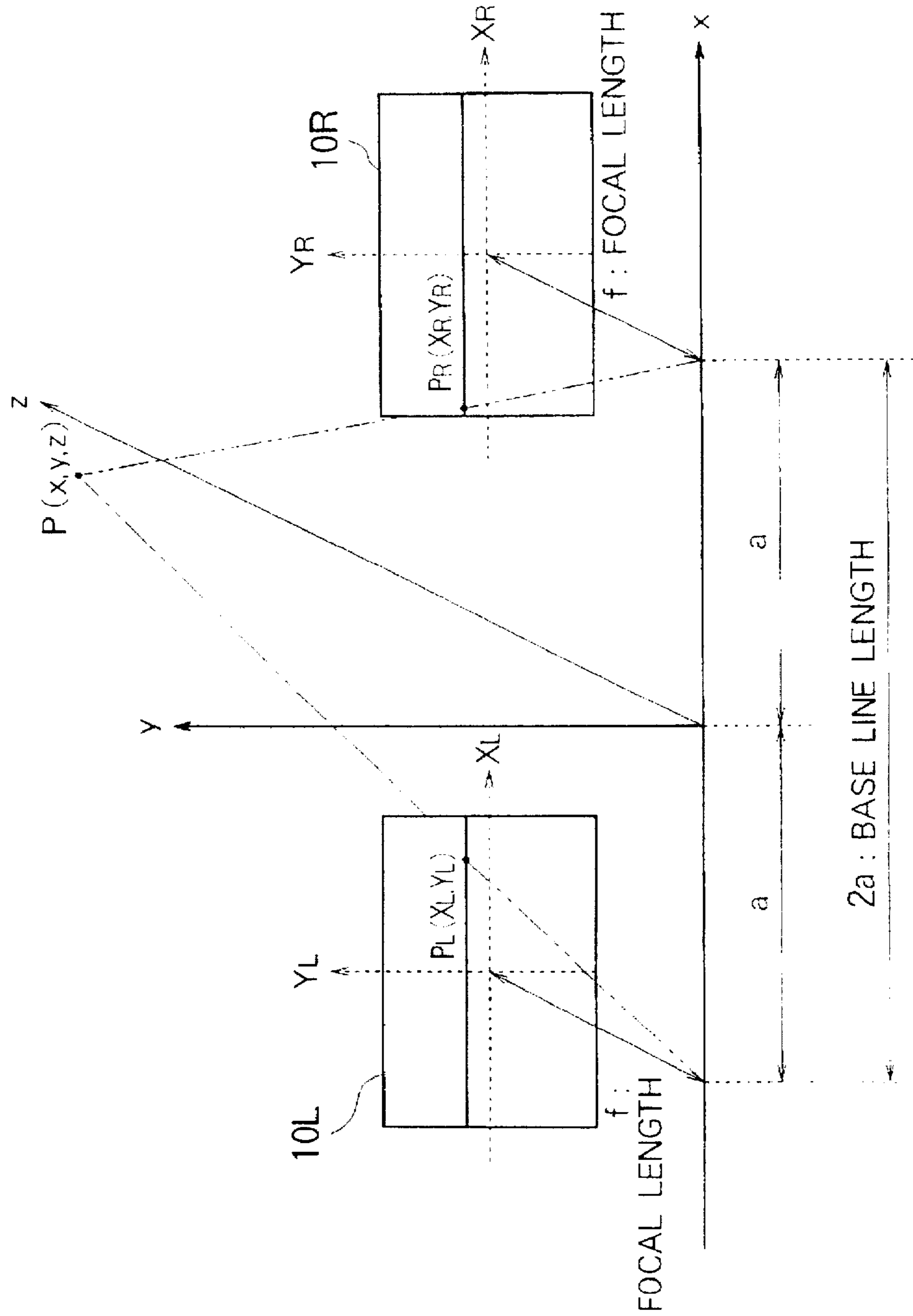
FIG. 1 PRIOR ART
