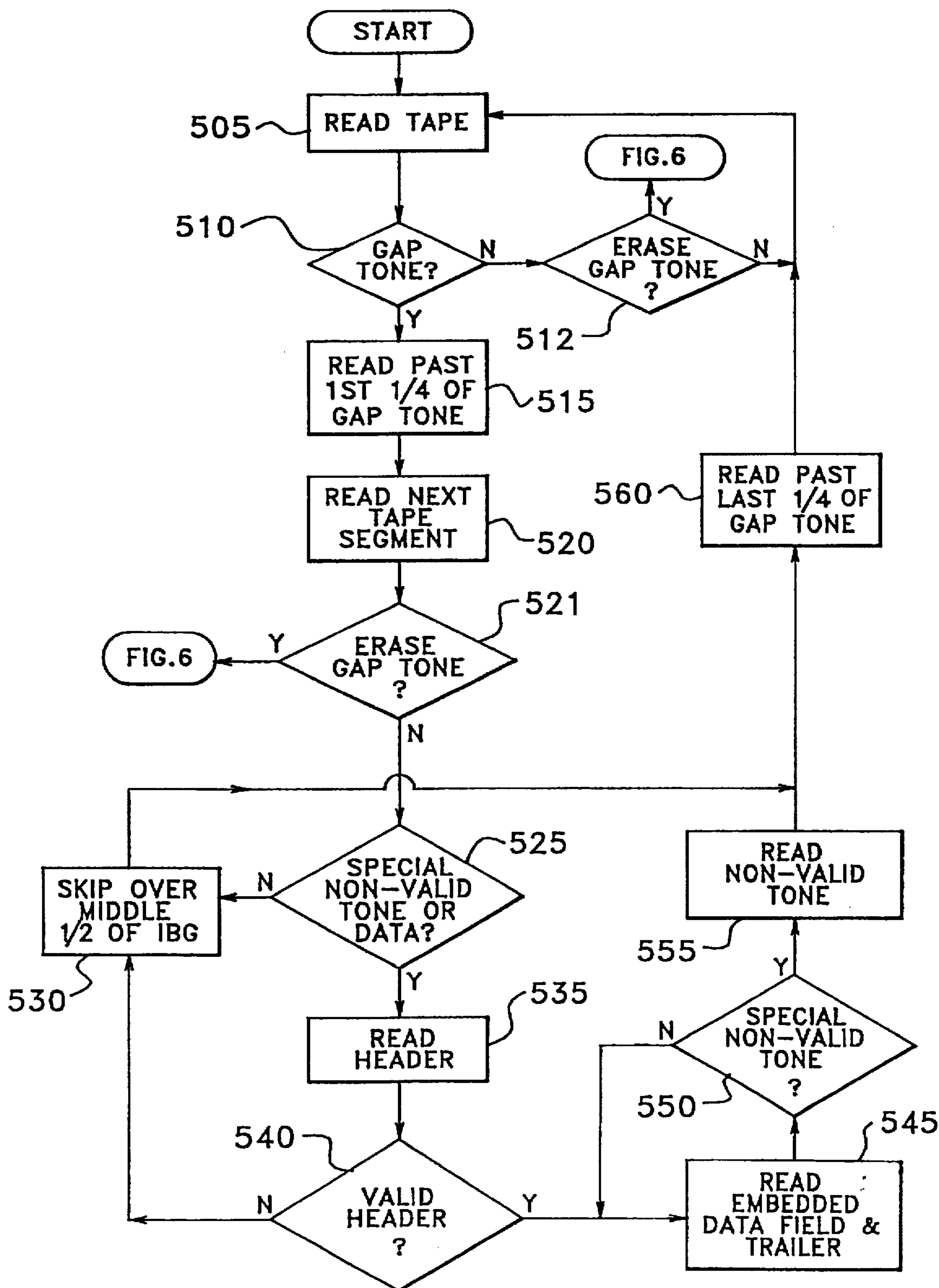
READ EMBEDDED DATA FIG. 5
