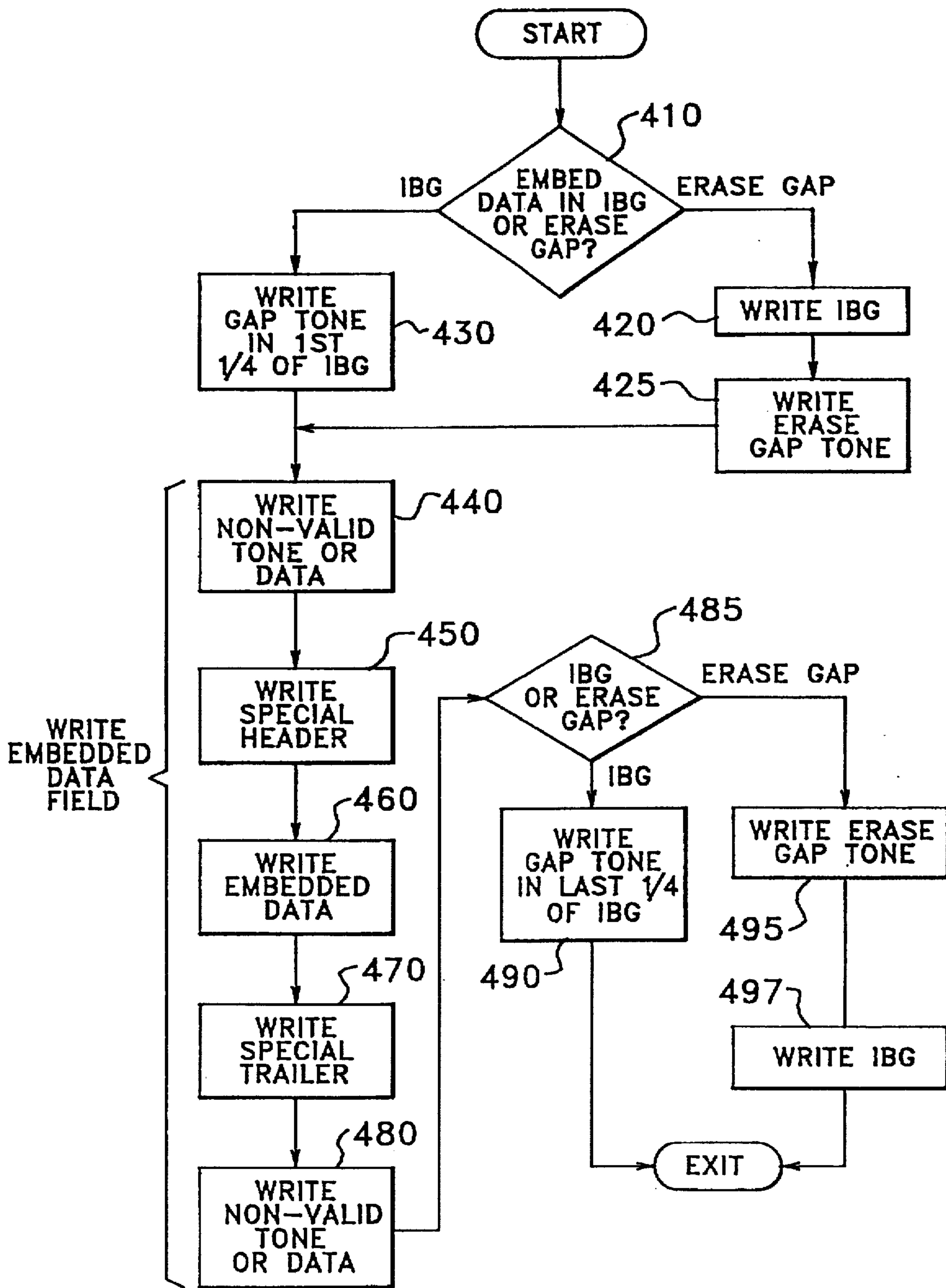
WRITE EMBEDDED DATA FIG. 4
