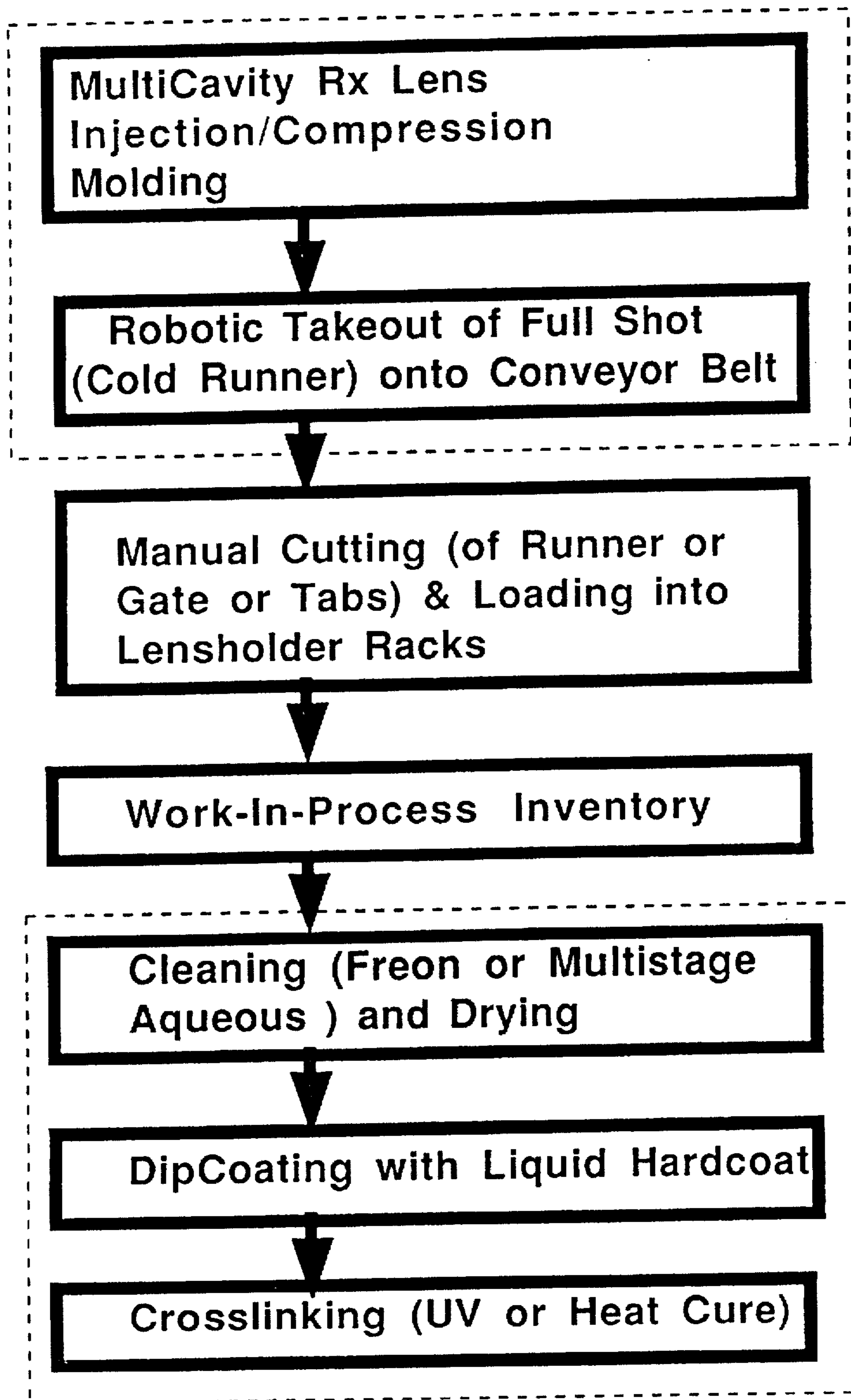
Figure 4A: Comparative Example ("Batch Process")
