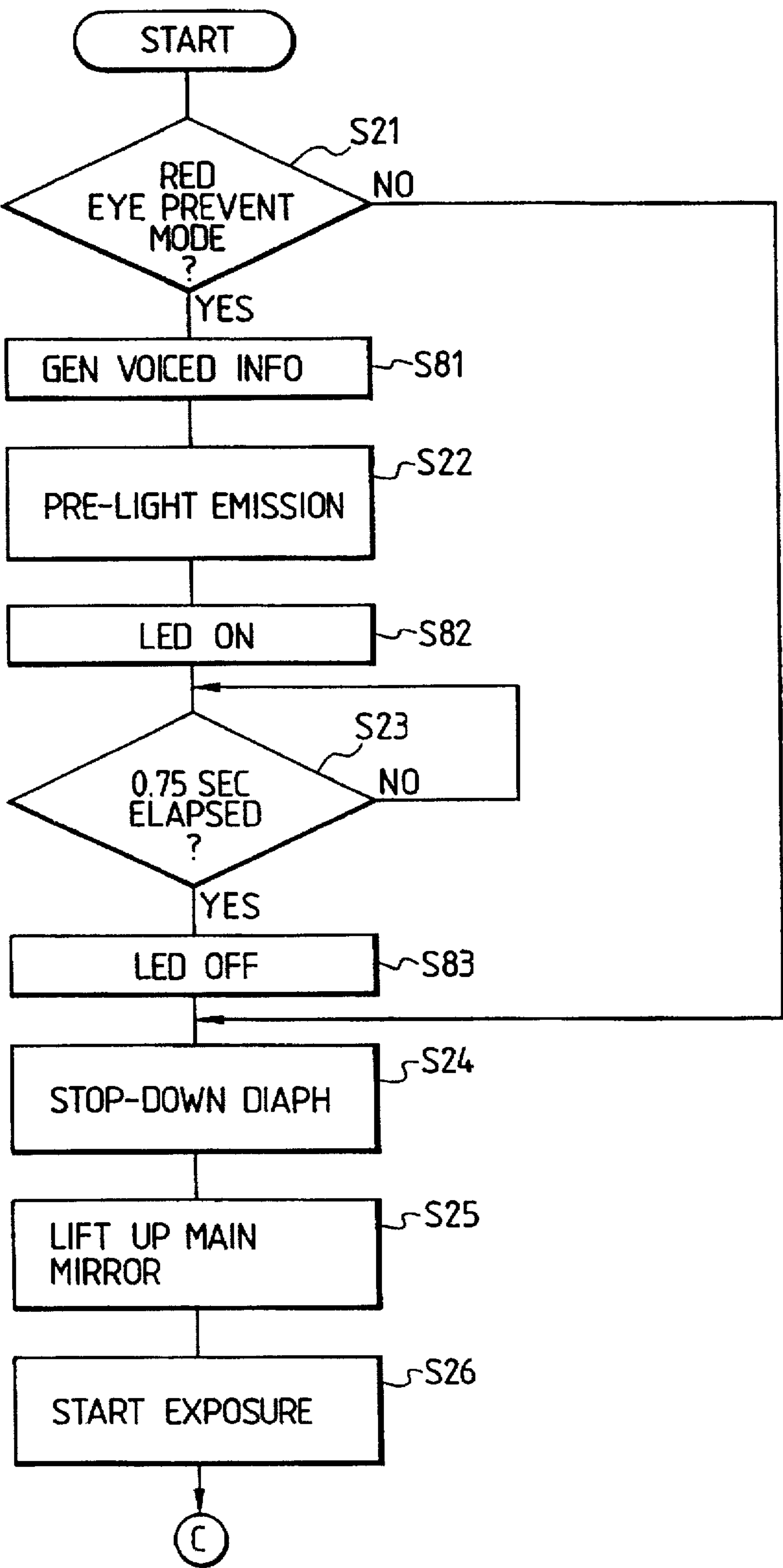
FIG. 12 INTERRUPT ROUTINE
