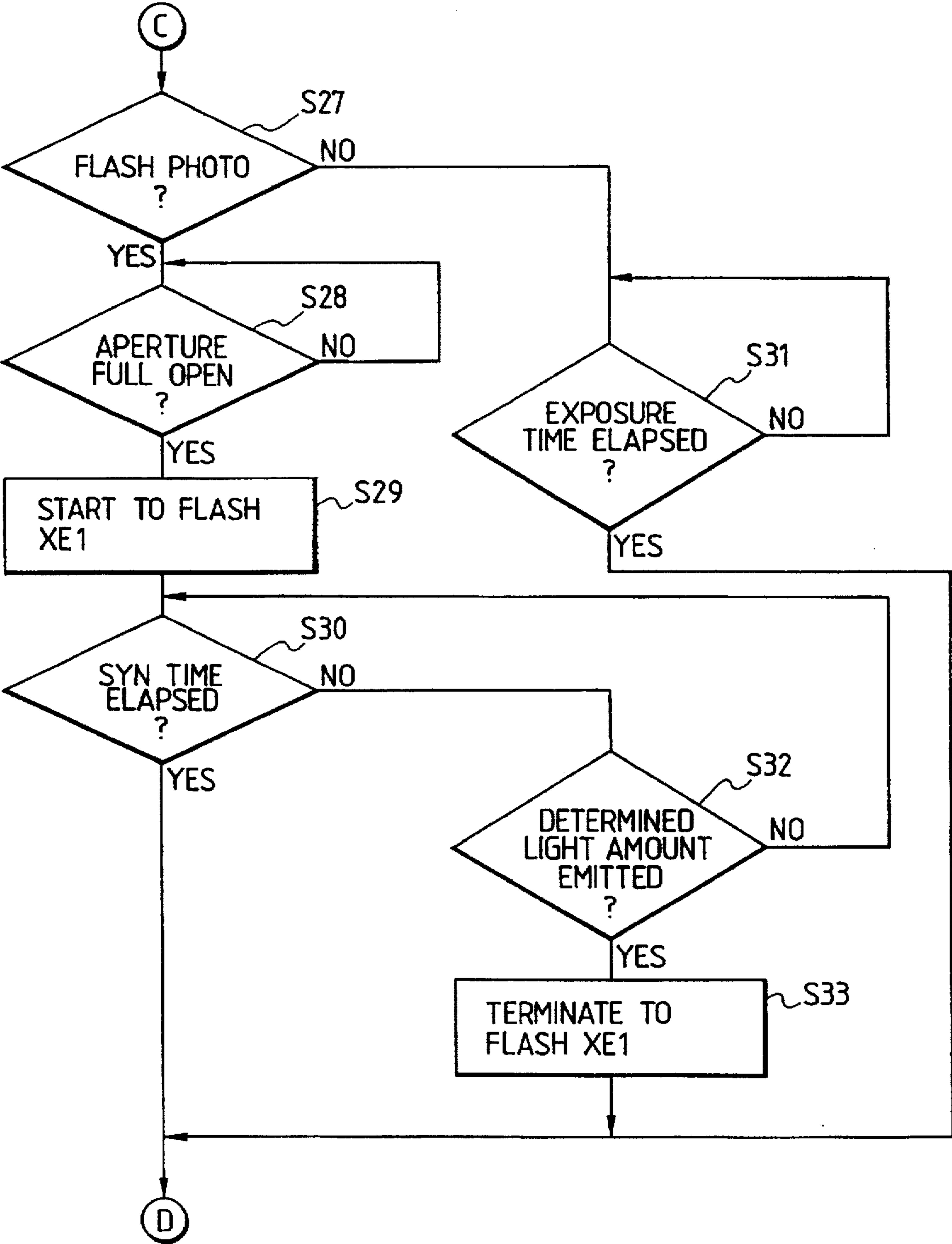
FIG. 6 INTERRUPT ROUTINE
