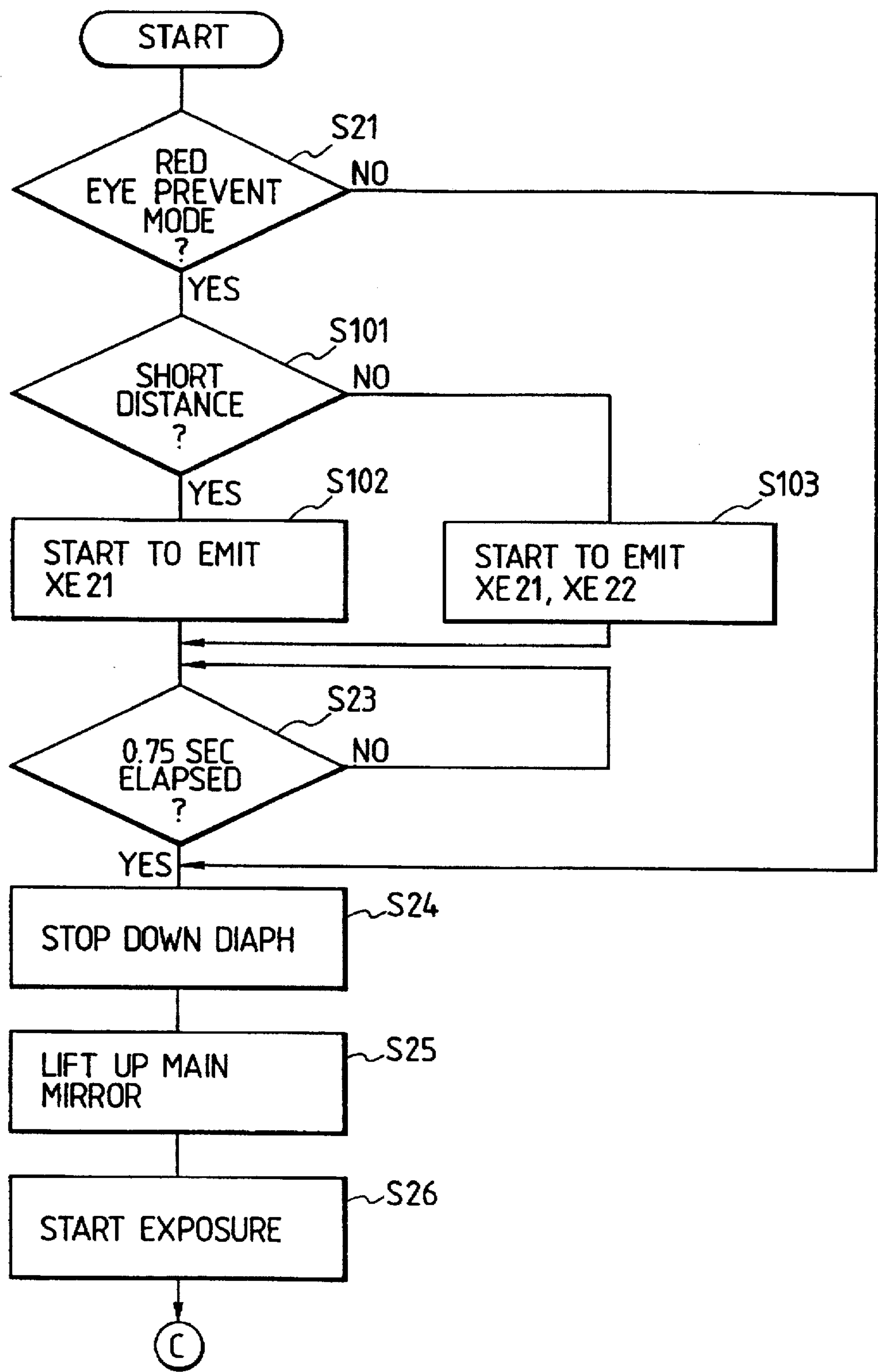
FIG. 16 INTERRUPT ROUTINE
