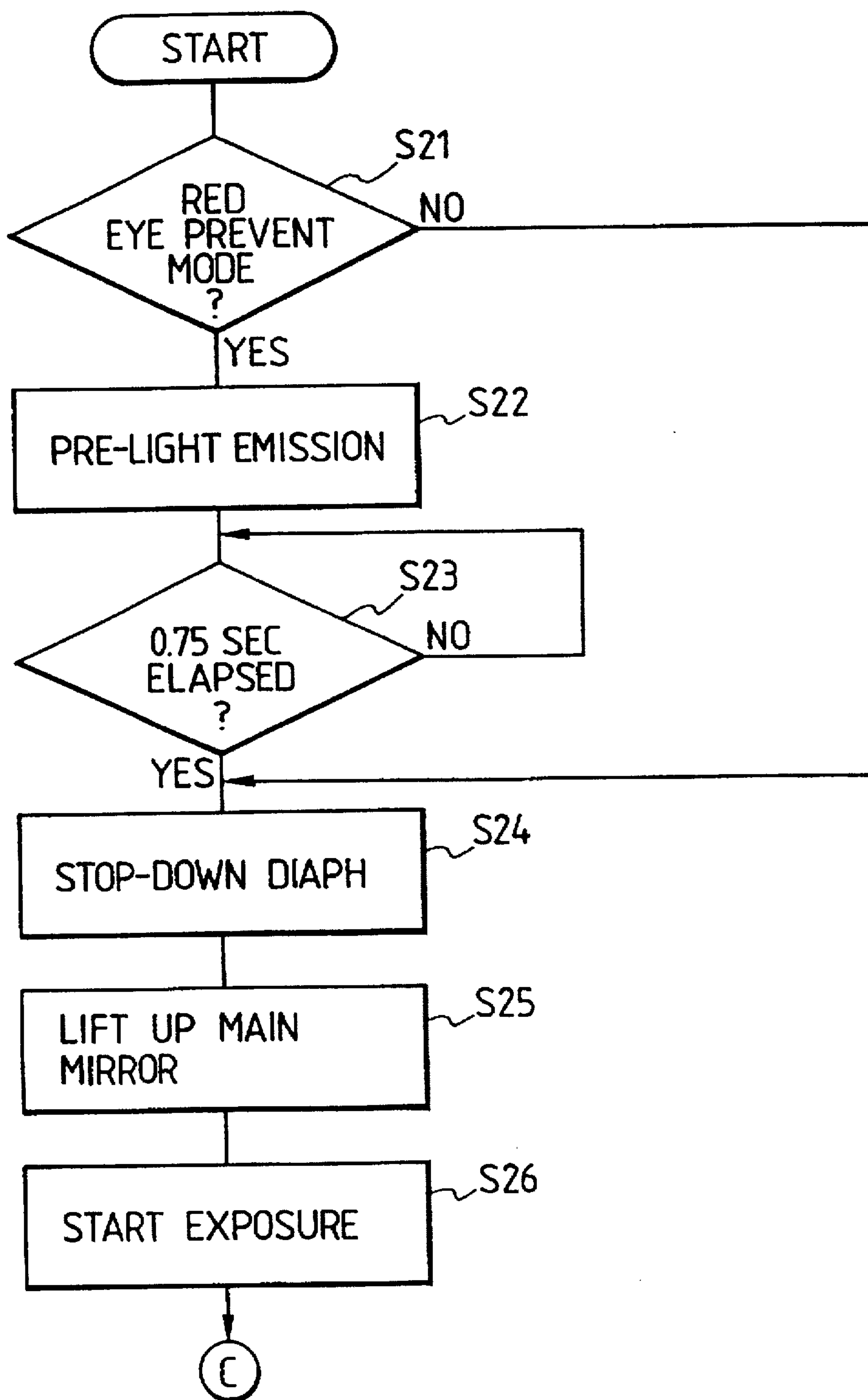
FIG. 5 INTERRUPT ROUTINE
