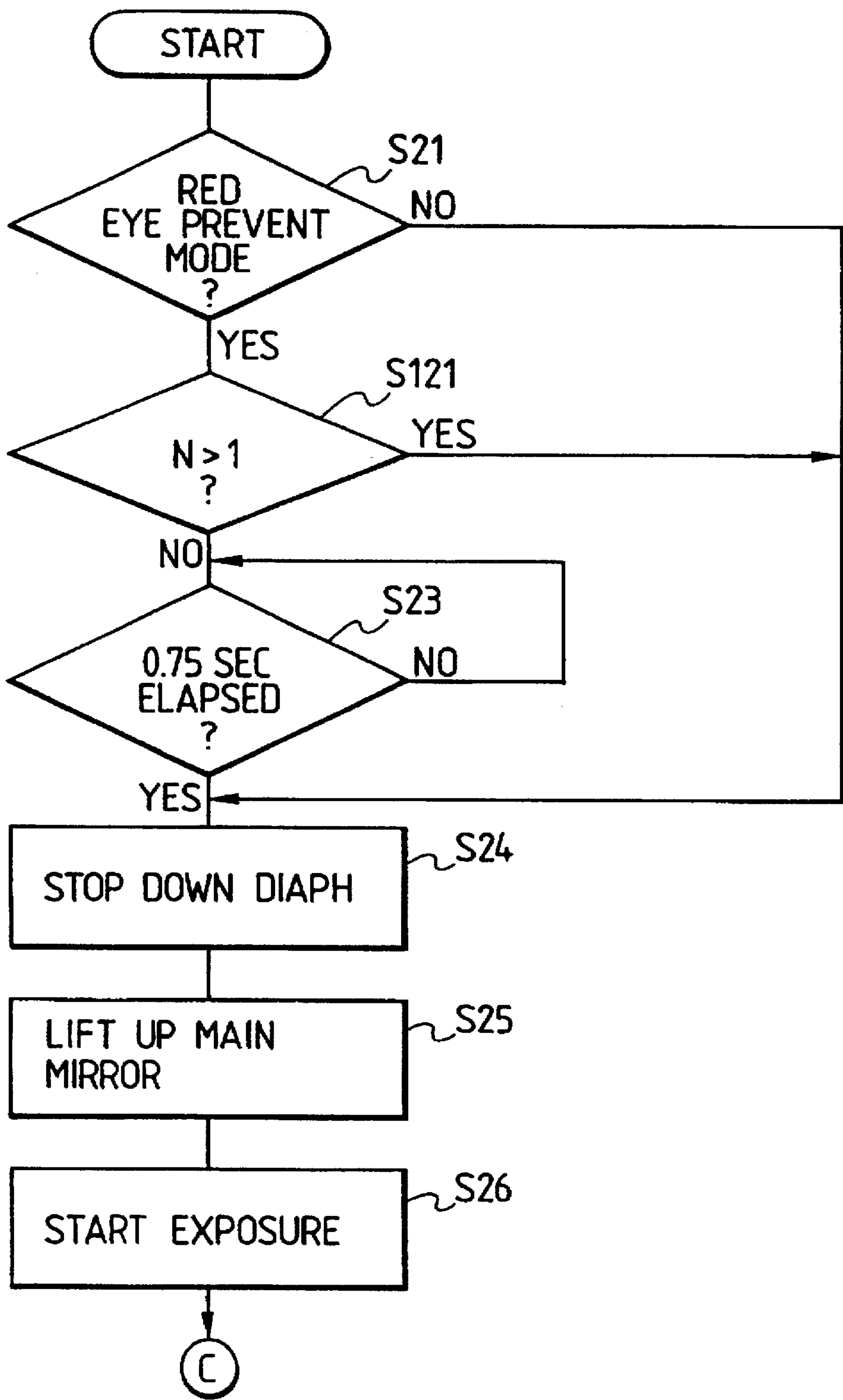
FIG. 18 INTERRUPT ROUTINE
