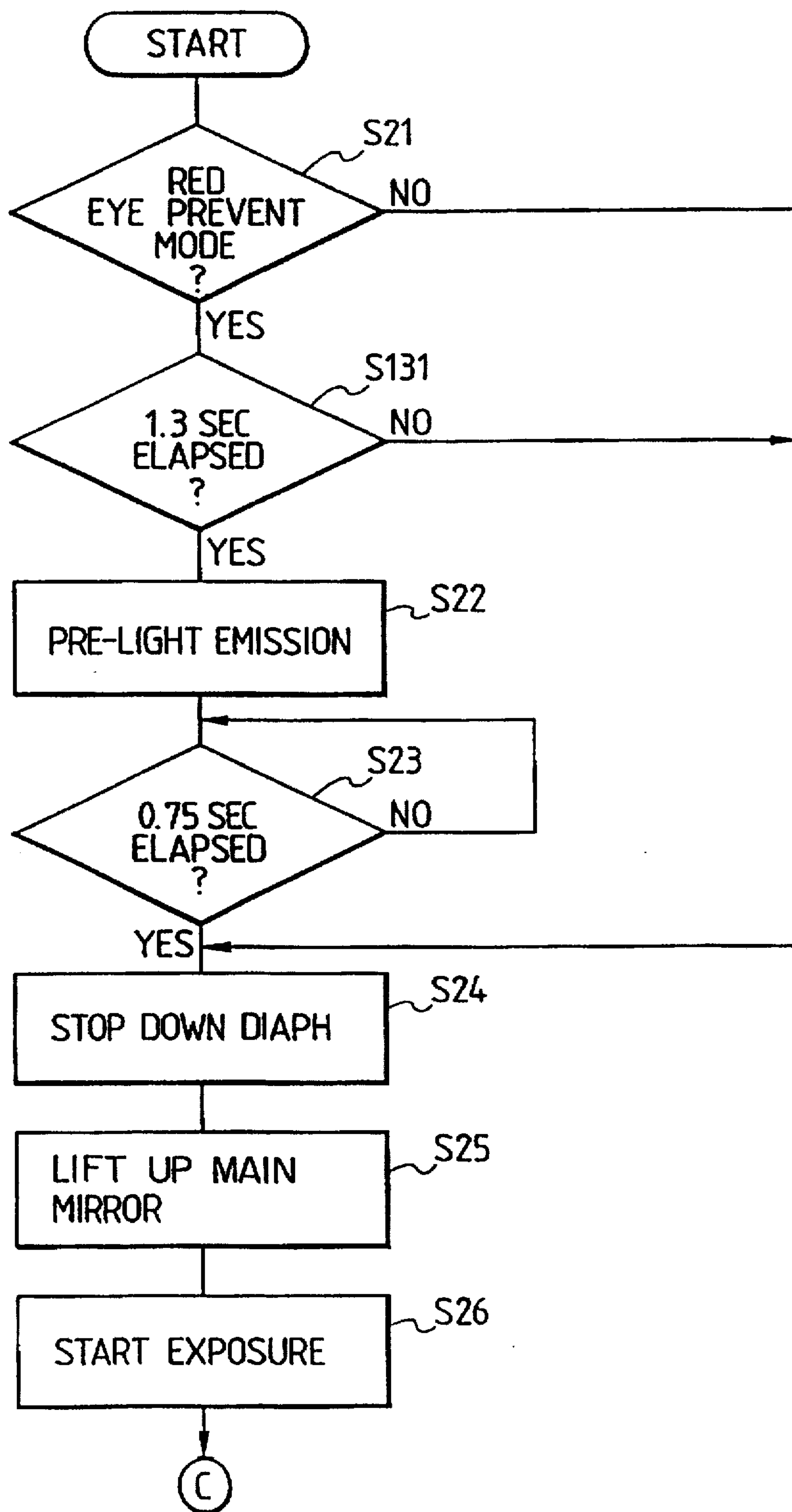
FIG. 20 INTERRUPT ROUTINE
