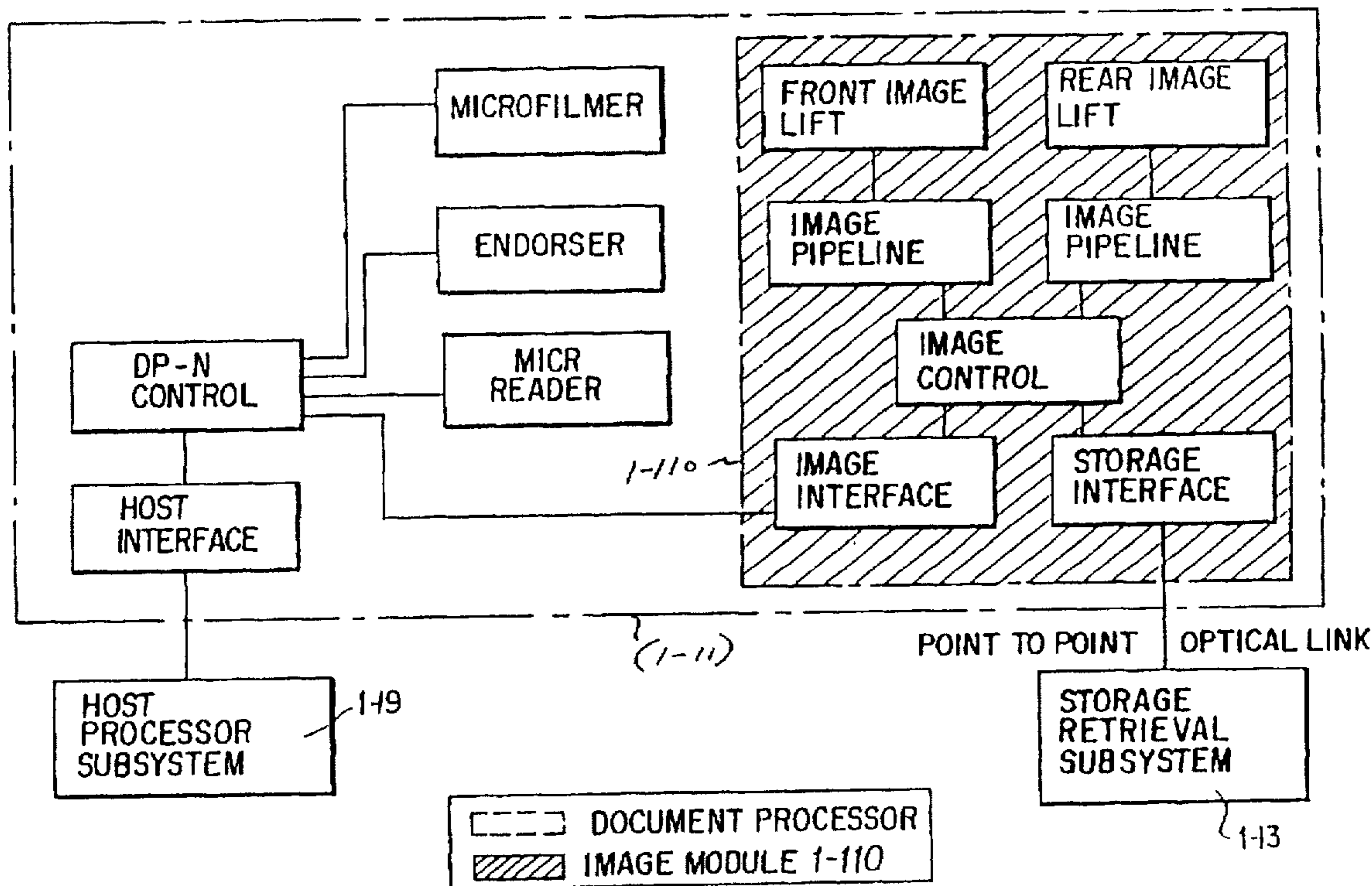
DOCUMENT PROCESSOR SUBSYSTEM FUNCTIONS
