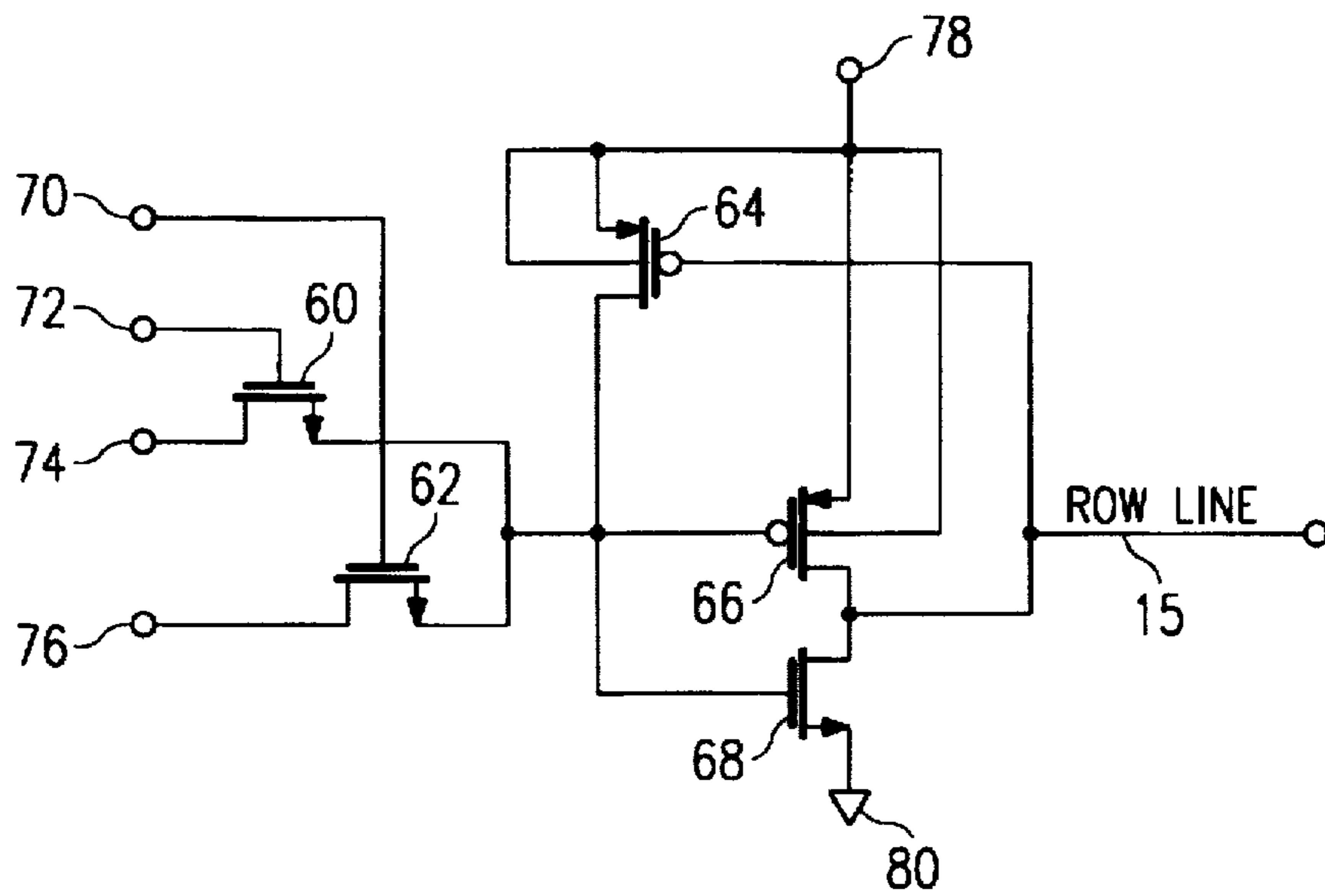
FIG. 4 (PRIOR ART)
