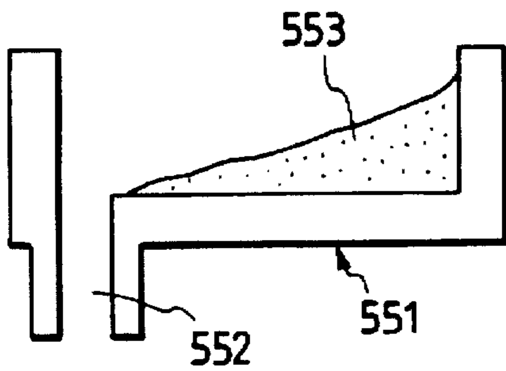
FIG. 26 PRIOR ART
