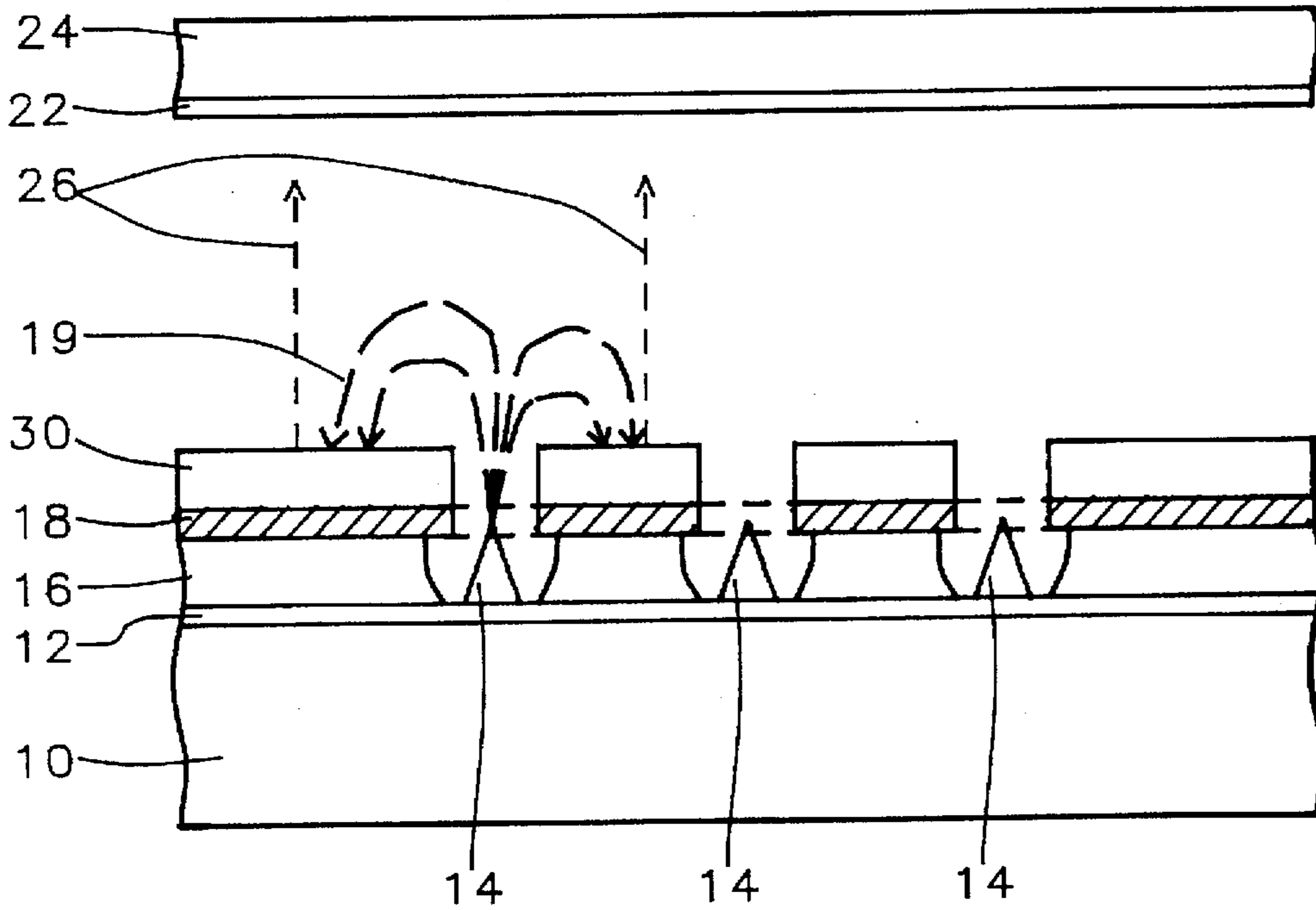
FIG. 2 - Prior Art
